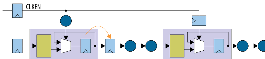
Figure 125. Retiming Example Ending Point
