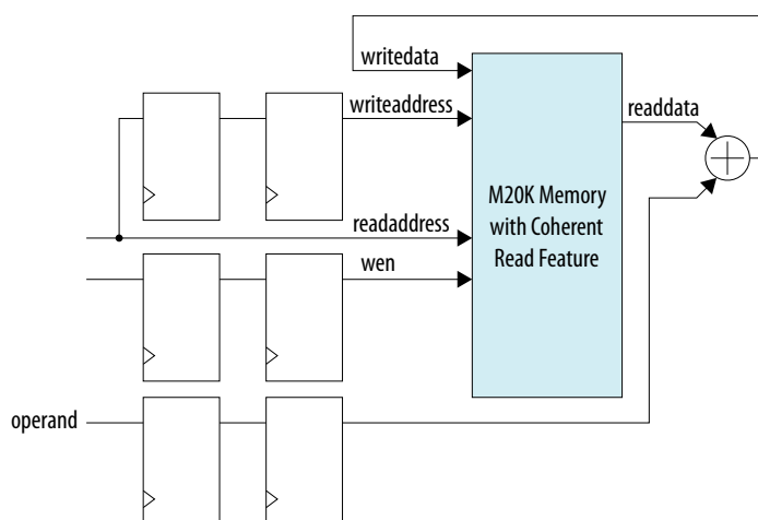
Figure 59. Registered Output Data Requires Two Register Stages
