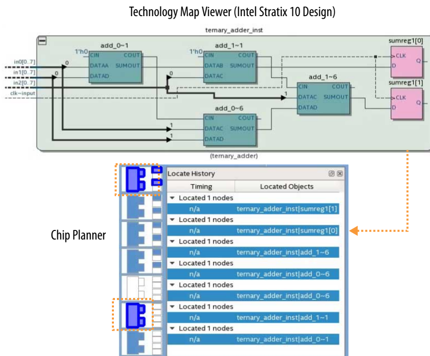
Figure 71. Intel Stratix 10: ALMs used to add 2 LSBs from a three 8-bit input adder
