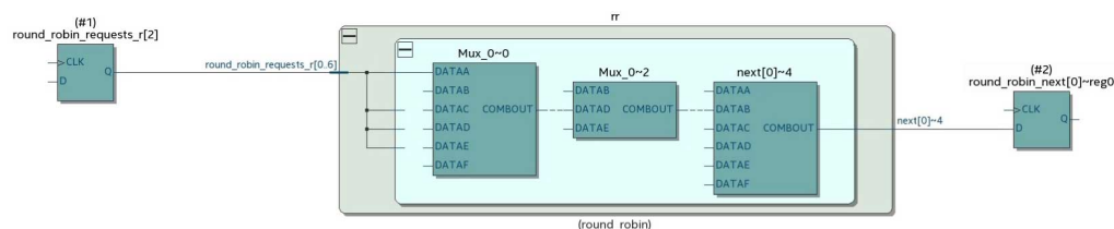
Figure 100. Critical Chain Schematic with Domain Boundary
