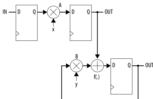
Figure 46. Separation of Forward Logic from the Loop
