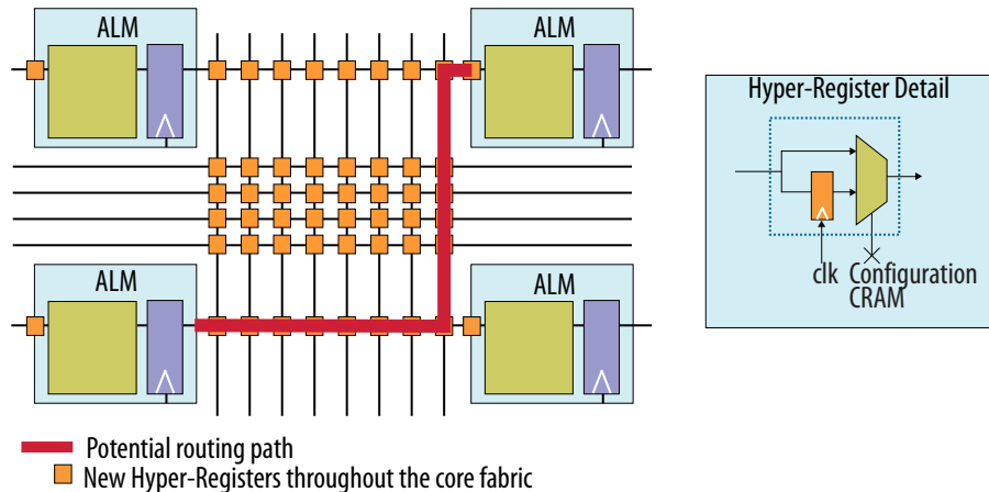
Figure 73. Hyper-Register Architecture
