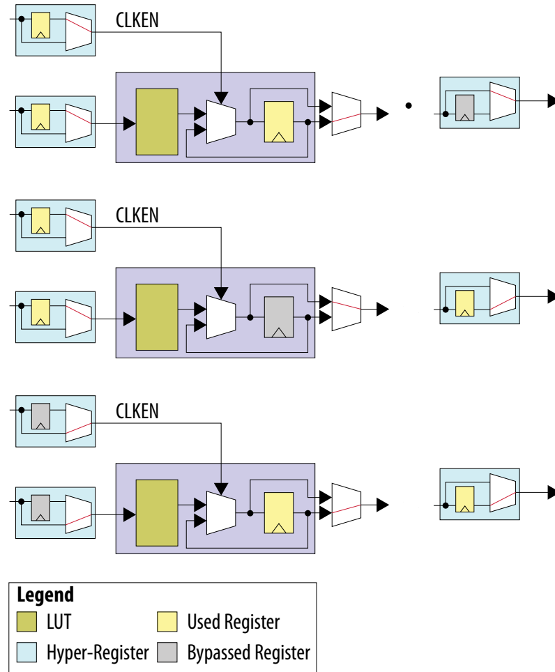
Figure 120. Retiming Steps and Structure with an ALM register and Hyper-Registers
