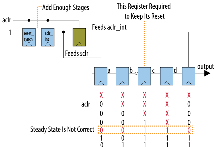
Figure 12. Validating the Output to Synchronize with Reset
