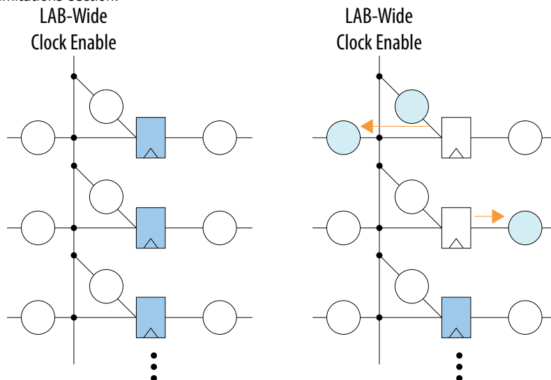
Figure 119. ALM Representing Clock Enables
