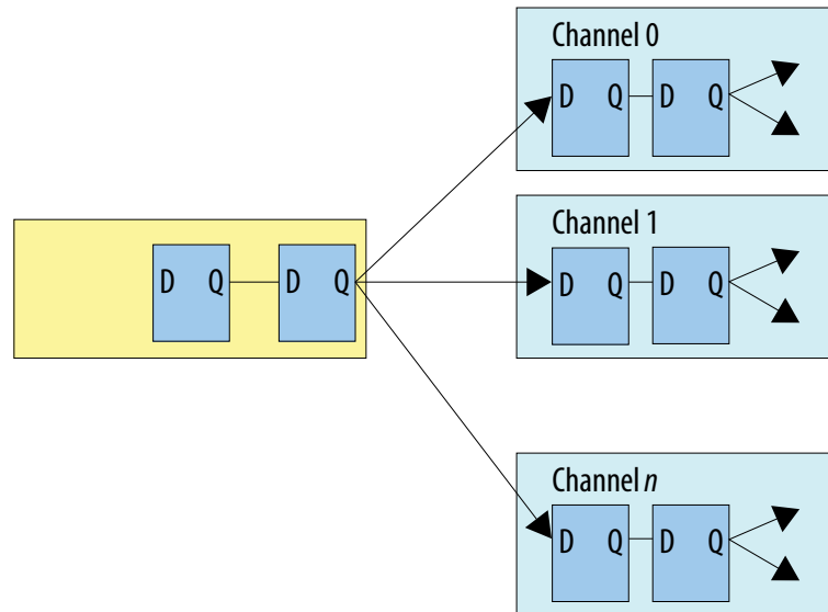
Figure 6. Optimal Pipelining of Broadcast Signals
