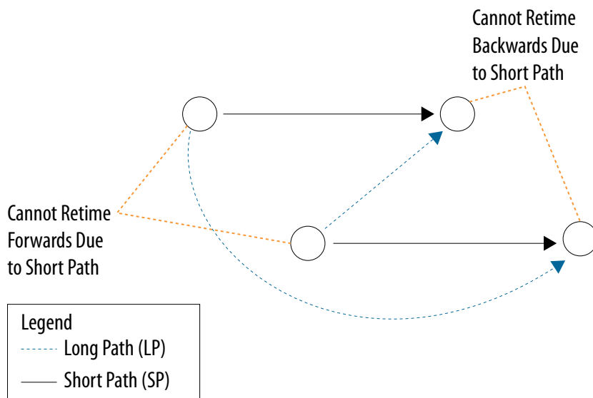
Figure 85. Critical Chain with Alternating Short Path/Long Path
