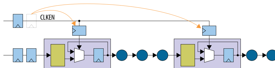
Figure 124. Retiming Example Intermediate Point
