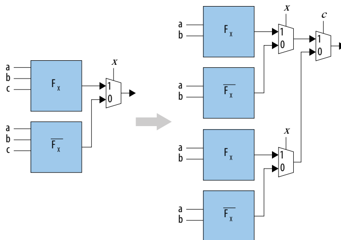
Figure 34. Repeated Shannon's Decomposition
