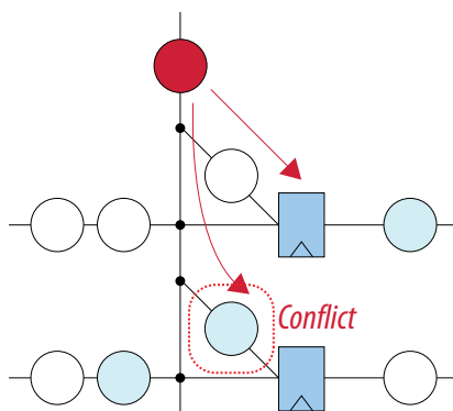
Figure 117. Retiming Example – Conflict at Synchronous Clear
