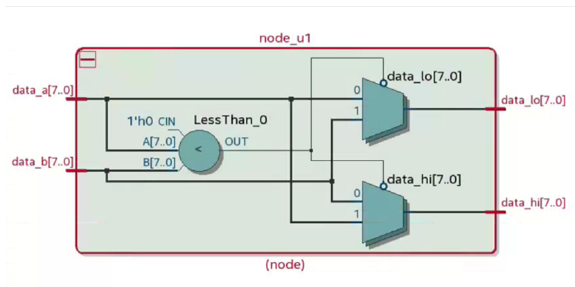
Figure 76. Node Component Connections
