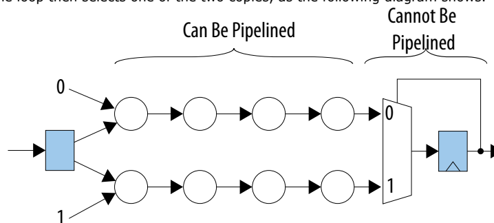
Figure 36. Loop Example after Shannon's Decomposition
