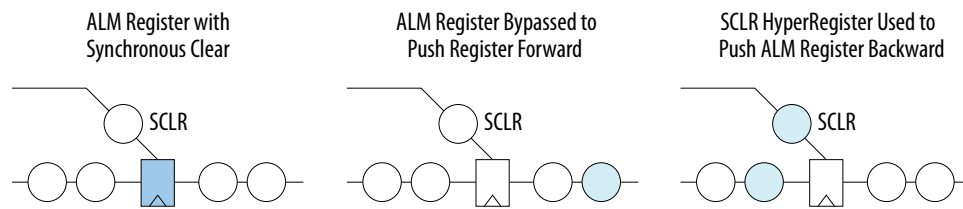
Figure 118. Aggressive Retiming
