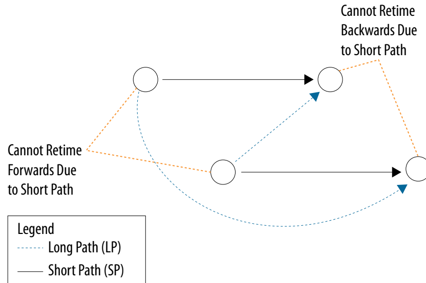
Figure 87. Critical Chain with Alternating Short Path/Long Path
