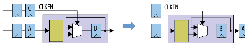
Figure 121. Retiming through a Clock Enable
