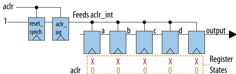
Figure 9. Partial Asynchronous Reset
