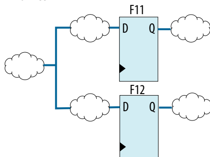
Figure 19. Circuit After Retiming Forward
