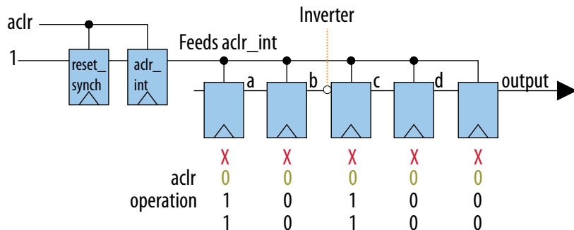
Figure 10. Circuit with an Inverter in the Register Chain
