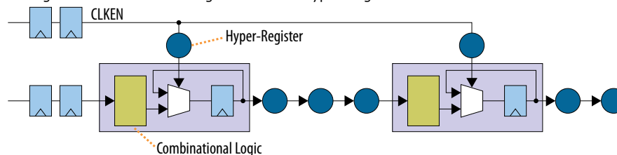
Figure 123. Retiming Example Starting Point
