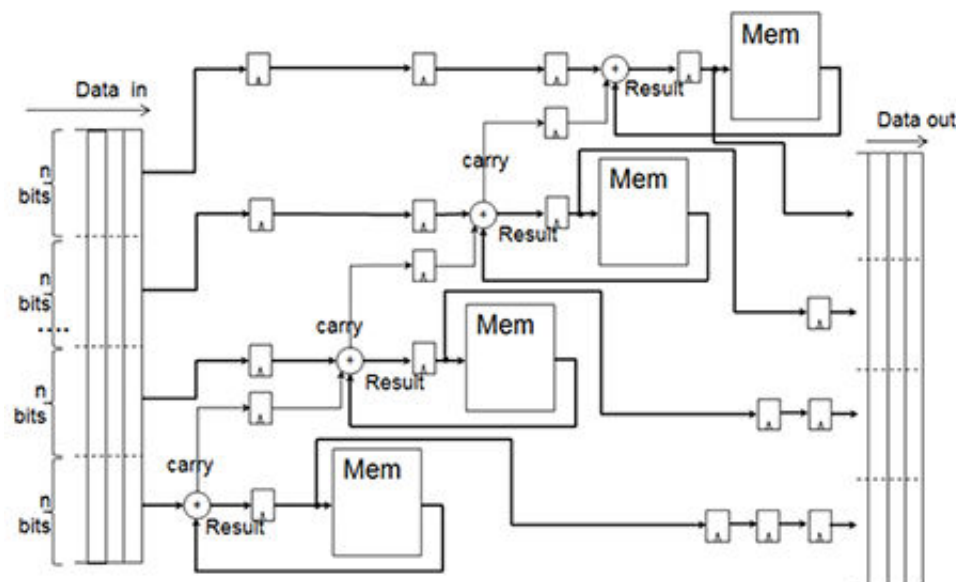
Figure 61. Pipelining Read-Modify-Write Memory
