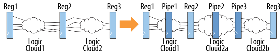
Figure 29. Hyper-Pipelining User Modifications
