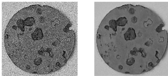
Figure 75. Before and After Images Processed with Median Filtering
