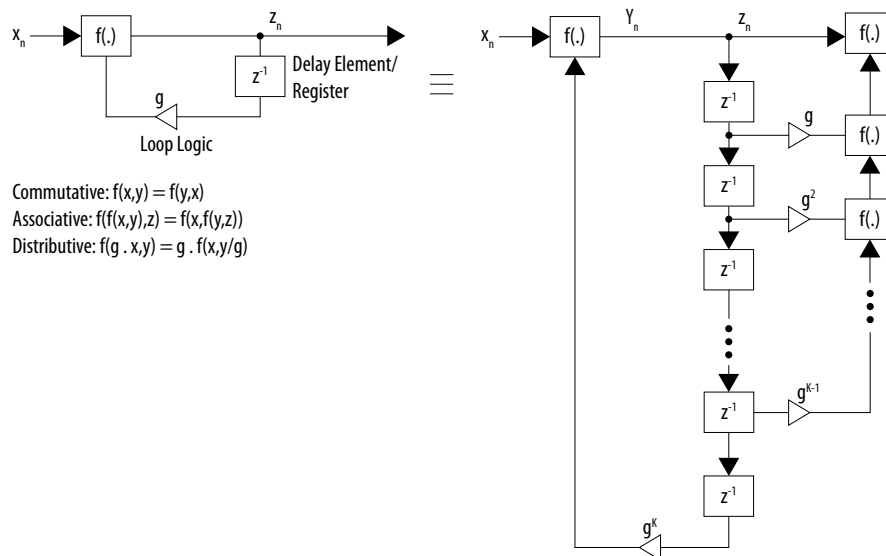
Figure 44. Equivalent Loop After Modification
