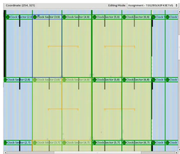
Figure 51. Clock Sector Boundary Layer in Chip Planner
