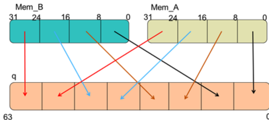
Figure 68. Memory Output Descrambling Example
