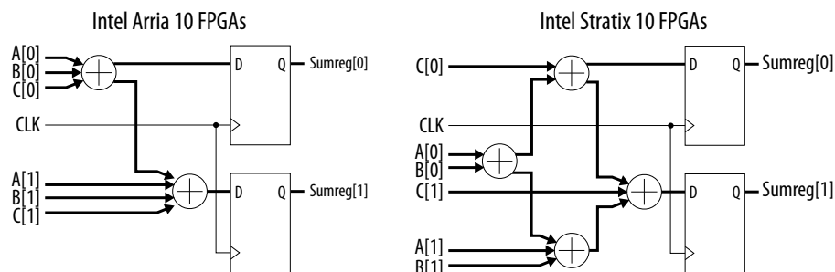
Figure 69. RTL View of Intel Arria 10 versus Intel Stratix 10 to add 2 LSBs from a three 8-bit input adder
