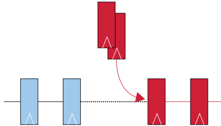
Figure 14. Simple Clock Domain Crossing After Adding Latency
