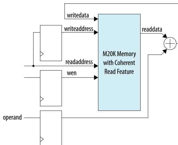
Figure 60. Unregistered Output Data Requires One Register Stage
