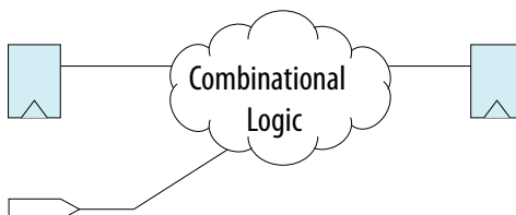
Figure 99. Domain Boundary with Unregistered Input/Output
