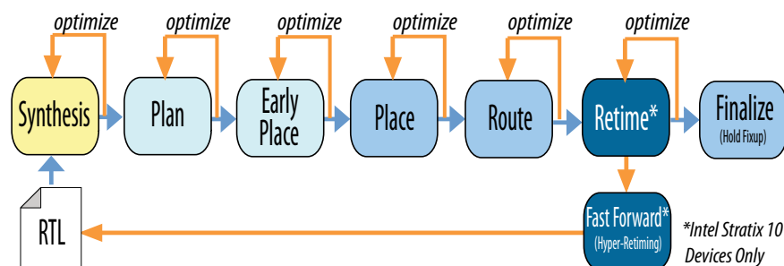
Figure 72. Hyper-Aware Design Flow
