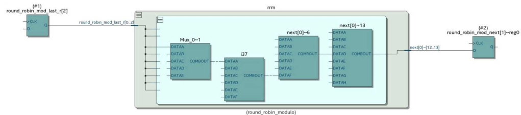
Figure 109. Schematic for Critical Chain with Performance Improvement
