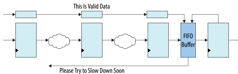
Figure 55. Using a FIFO Buffer to Control Backpressure
