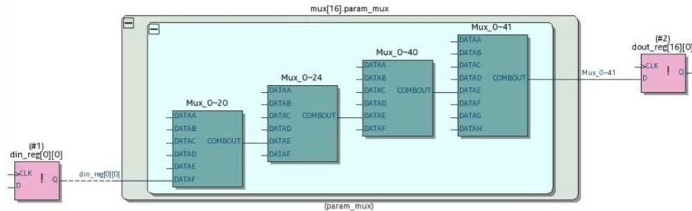
Figure 83. Critical Chain with Insufficient Registers Reported During Hyper-Retiming
