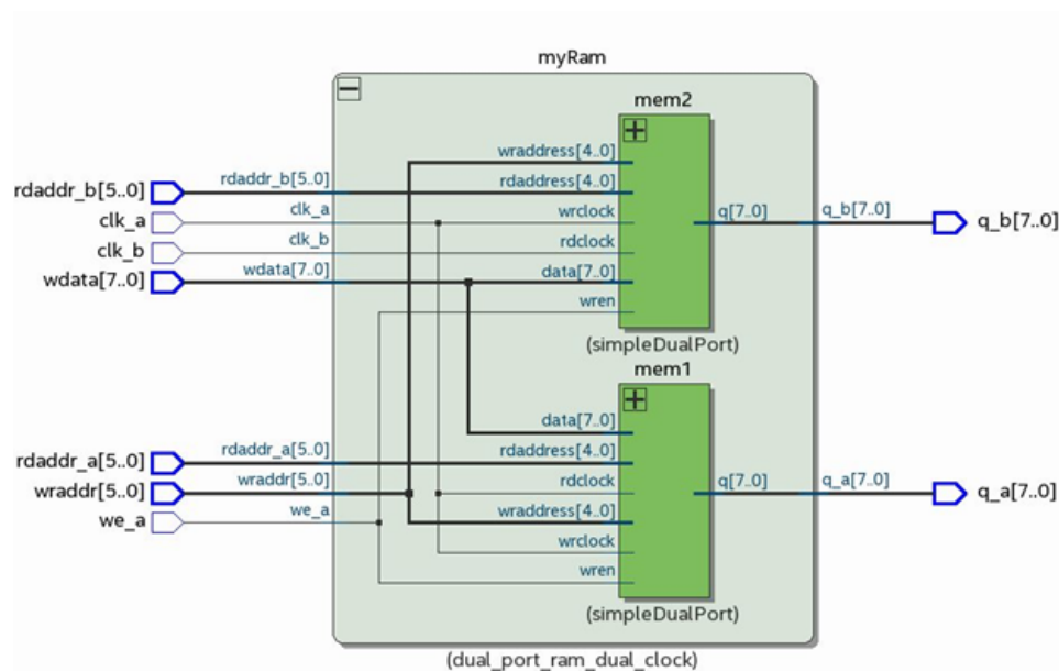
Figure 65. Simple Dual-Port Memory Implementation
