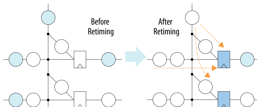
Figure 116. Retiming Example – Register Splits on the Path to other Synchronous Clear Ports
