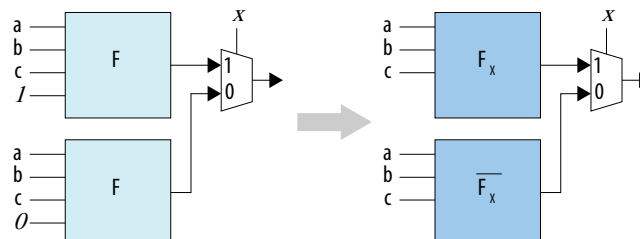
Figure 33. Shannon's Decomposition Logic Reduction
