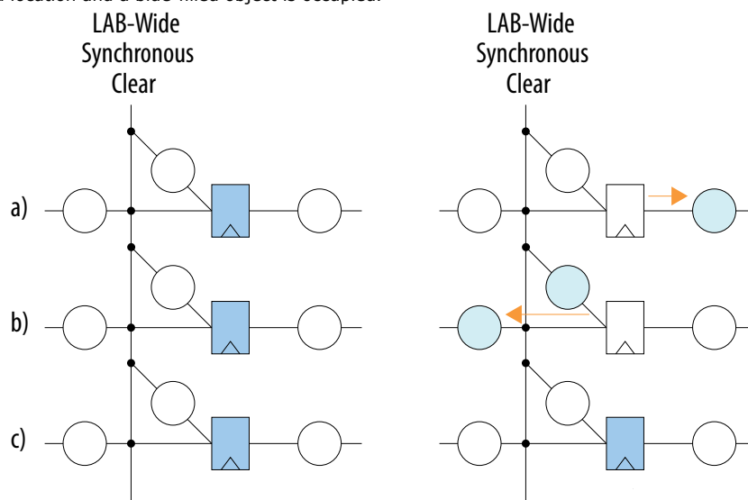
Figure 114. Retiming Example for Synchronous Resets
