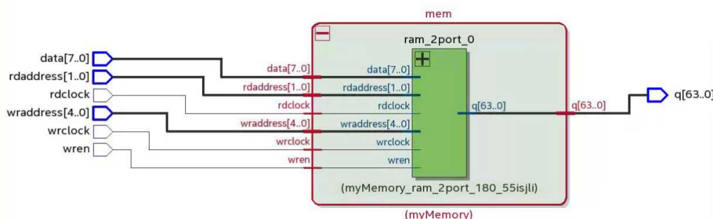
Figure 66. Dual-Port Memory with Invalid 1/8 Mixed Port Ratio
