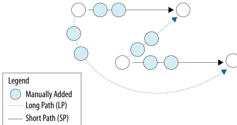
Figure 86. Sample Short Path/Long Path with Additional Latency
