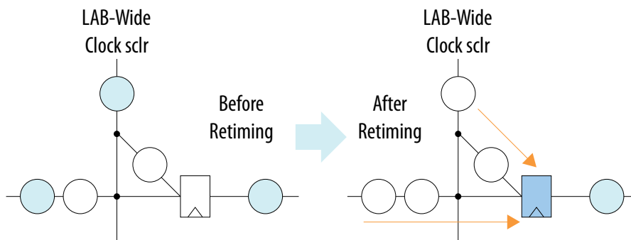
Figure 115. Retiming Example – Second Register Pushes out of ALM
