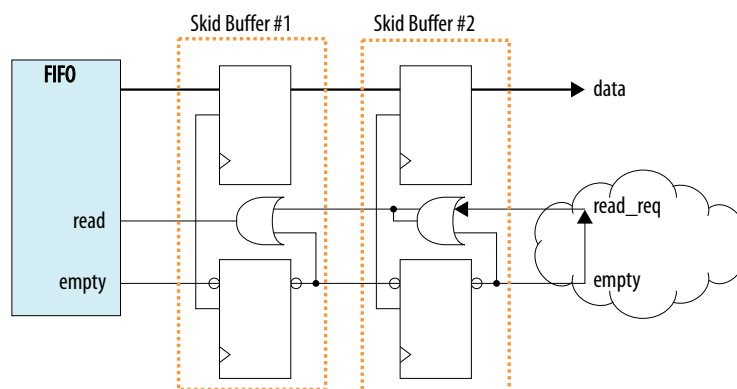
Figure 58. FIFO Flow Control Loop with Two Skid Buffers in a Read Control Loop
