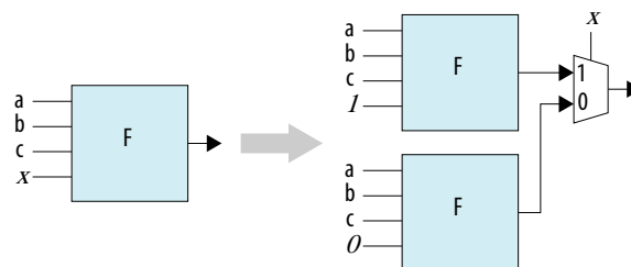
Figure 33. Shannon's Decomposition Logic Reduction
