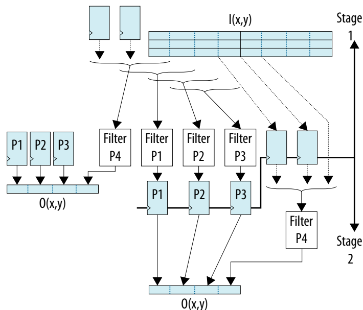
Figure 74. Median Filter Operational Diagram
