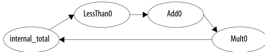
Figure 38. Elements of a Critical Chain Sub-Loop
