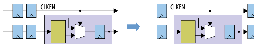
Figure 122. Retiming through a Clock Enable with a Branch Point
