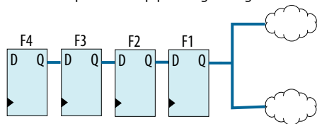
Figure 22. Impact of One Register Move
