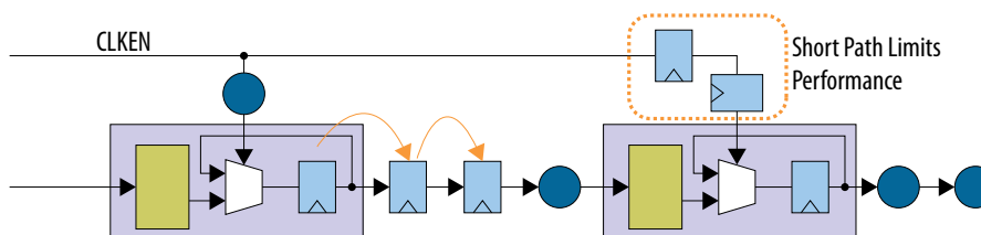
Figure 126. Retiming Example Limiting condition
