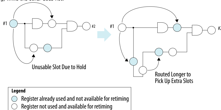
Figure 127. Short Paths Limiting Retiming
