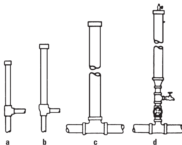
Figure 5-6 (a, b) Plain Air Chambers, (c) Standpipe Air Chamber, (d) Rechargeable Air Chamber
