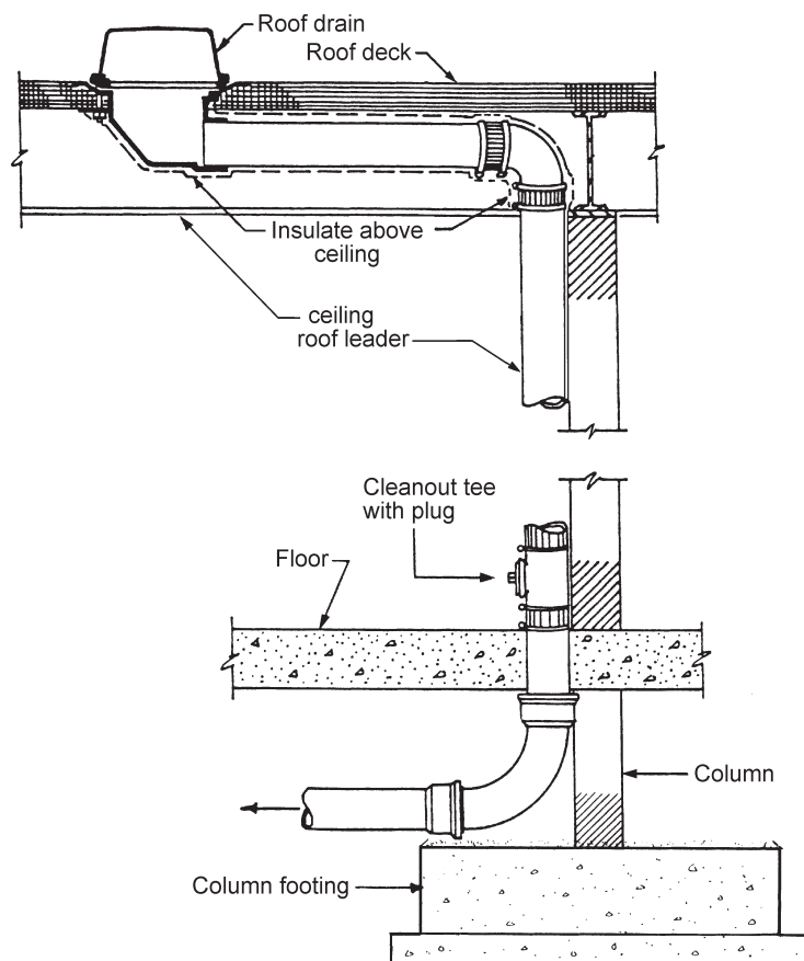
Figure 4-8 Typical Roof Drain and Roof Leader
