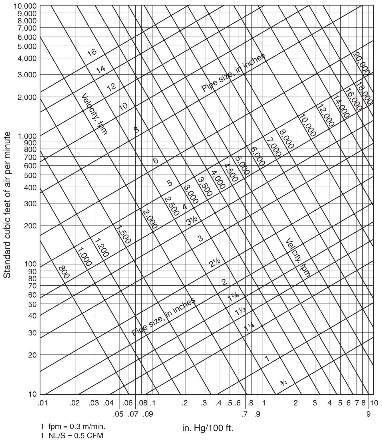
Figure 10-6 Vacuum Cleaning Piping Friction Loss Chart
