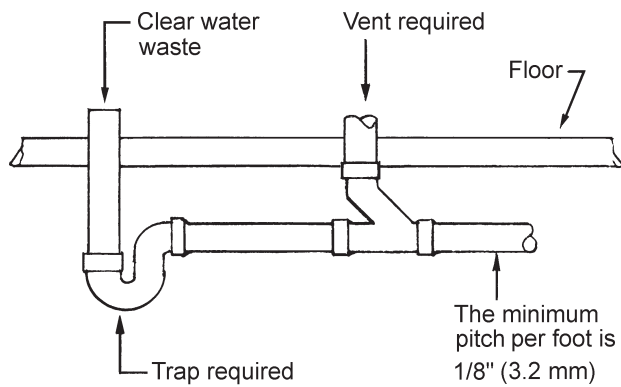
Figure 4-7 Clear Water Waste Branches for Connection to Storm System
