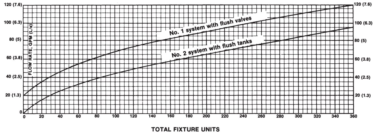
Figure 5-15 Conversion of Fixture Units, fu, to gpm (L/s)
