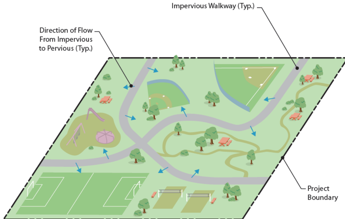
FIGURE 5-2. Self-Retaining Site
