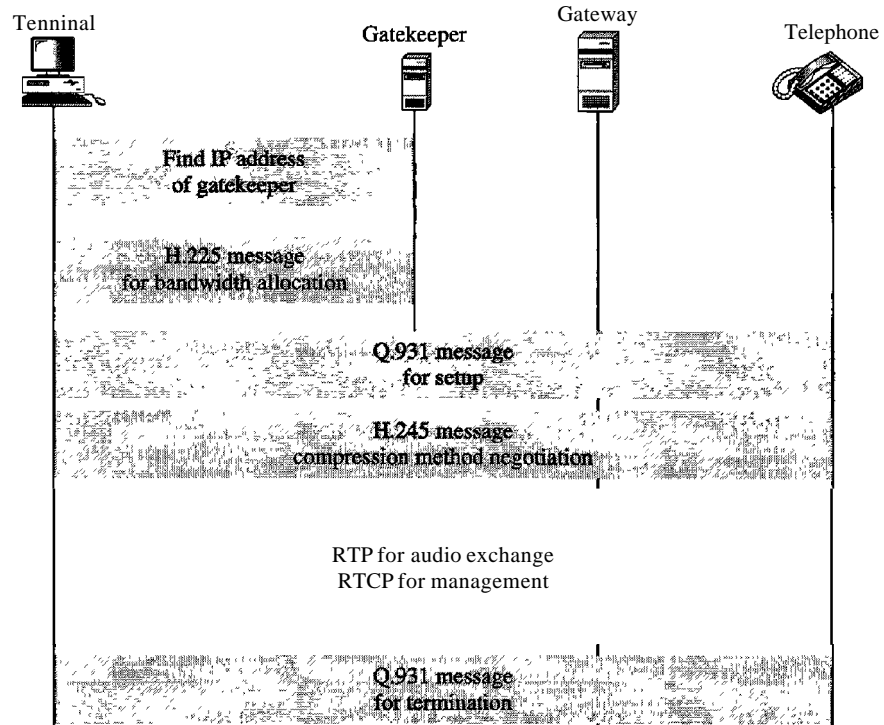
Figure 29.27 H.323 example
