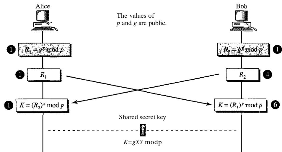
Figure 30.26 Diffie-Hellman method
