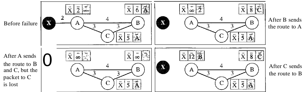
Figure 22.18 Three-node instability
