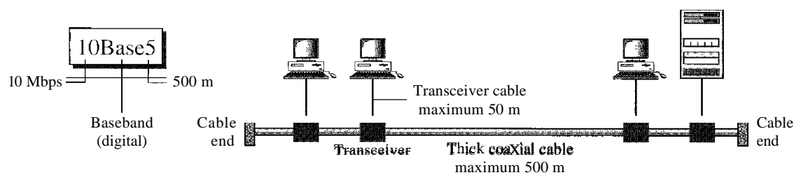
Figure 13.10 10Base5 implementation
