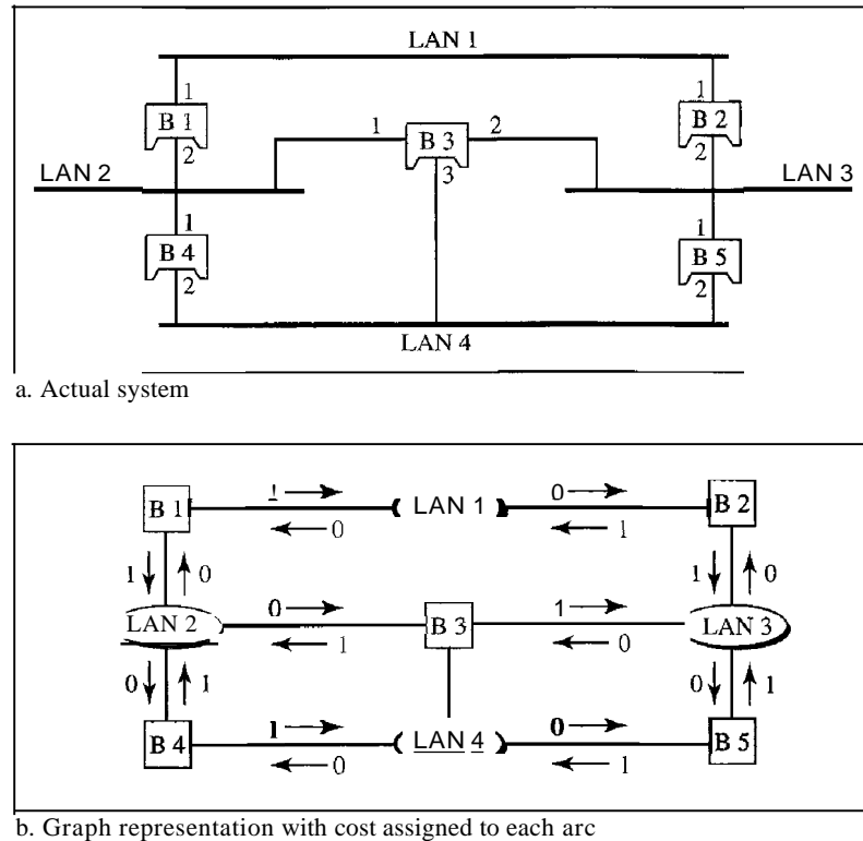
Figure 15.8 A system of connected LANs and its graph representation
