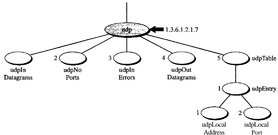
Figure 28.16 udp group
