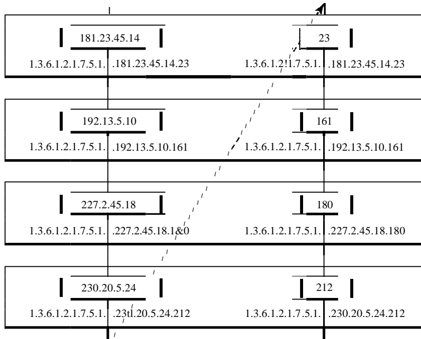
Figure 28.19 Lexicographic ordering
