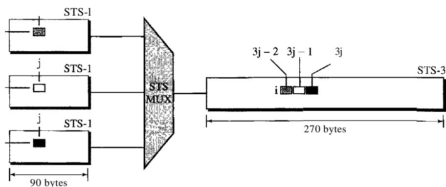
Figure 17.13 Byte interleaving
