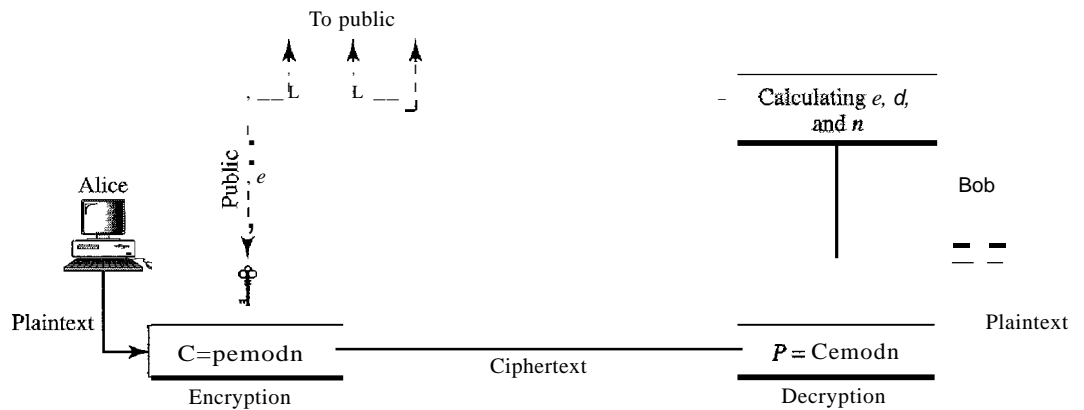
Figure 30.24 RSA
