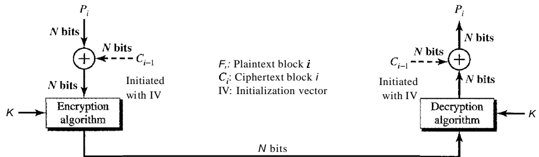
Figure 30.21 CBC mode
