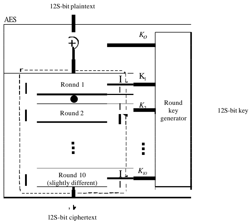
Figure 30.17 AES
