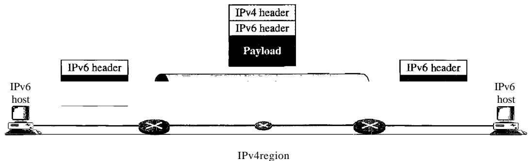
Figure 20.20 Tunneling strategy
