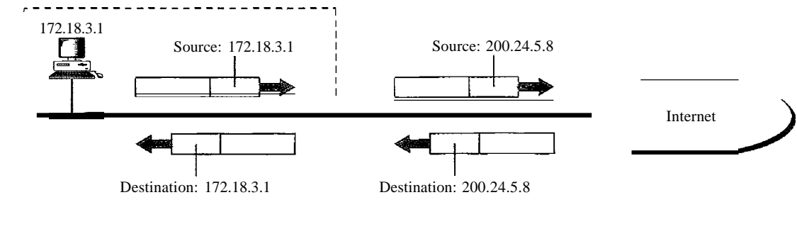
Figure 19.11 Addresses in a NAT
