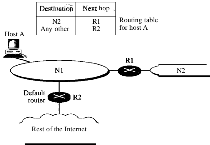
Figure 22.4 Default method
