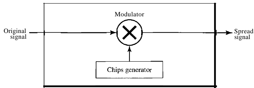
Figure 6.32 DSSS
