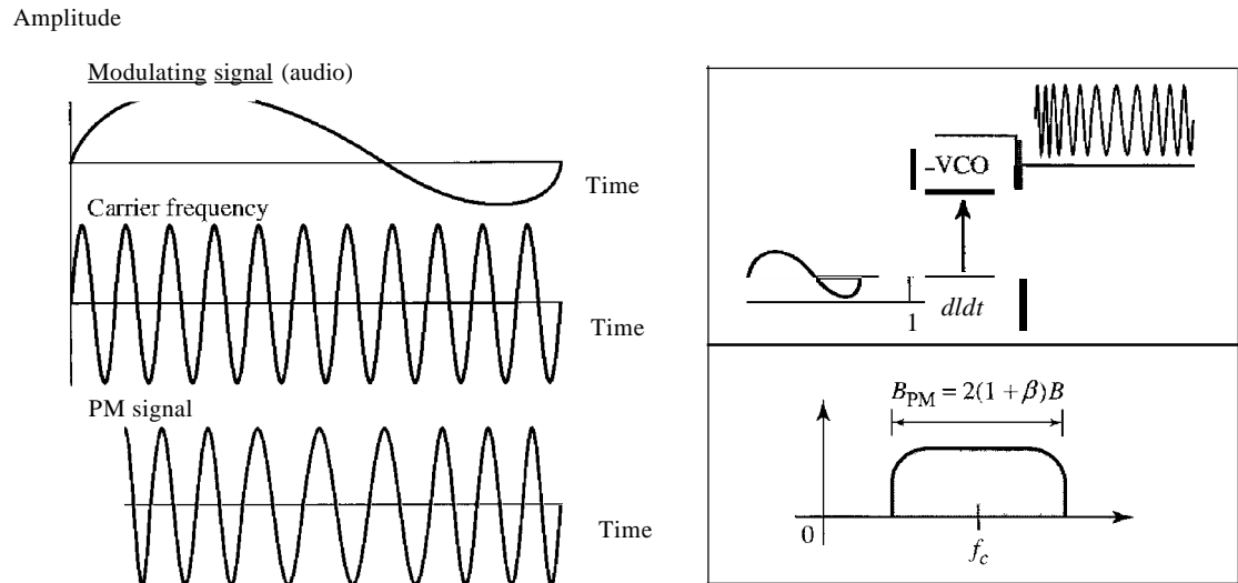
Figure 5.20 Phase modulation
