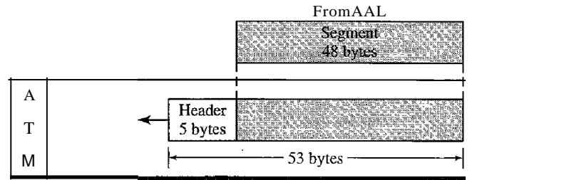
Figure 18.18 ATM layer
