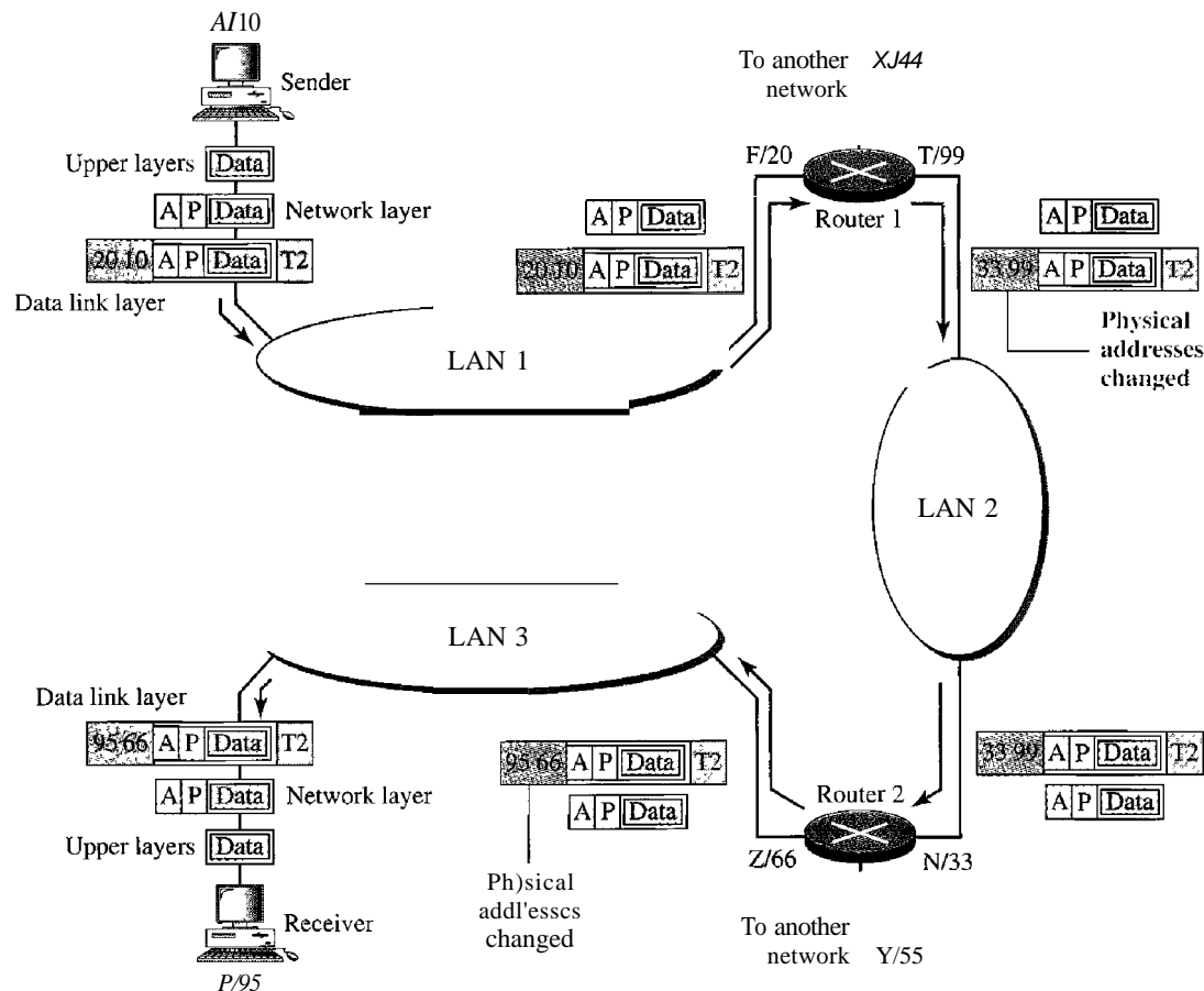
Figure 2.20 IP addresses
