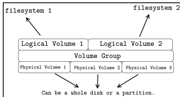
Figure 4: Visualizing LVM
