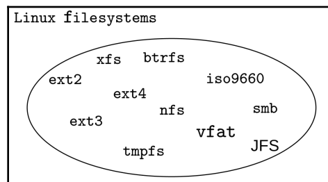
Figure 3: Linux filesystems
