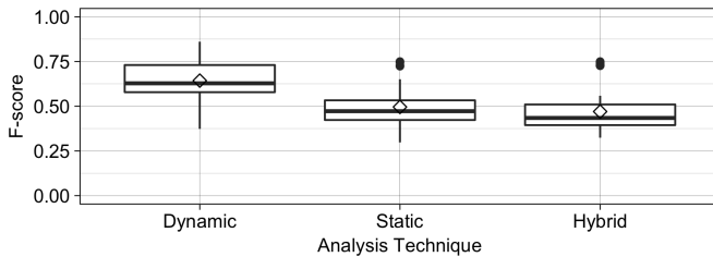
Fig. 6. F-score of Lacuna for each analysis technique.
