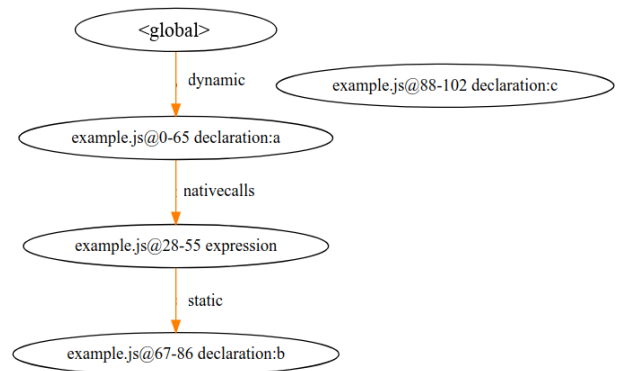
Fig. 3. Running example - G_w . Format of node labels: sourcefile@s-e type[:name] , where s and e are the start and end character positions of the function definition in sourcefile , type can be either declaration or expression , and name is its name.
