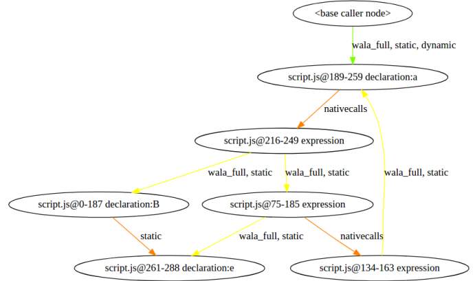
Fig. 4. Example Lacuna function graph output for a trivial JavaScript file.
