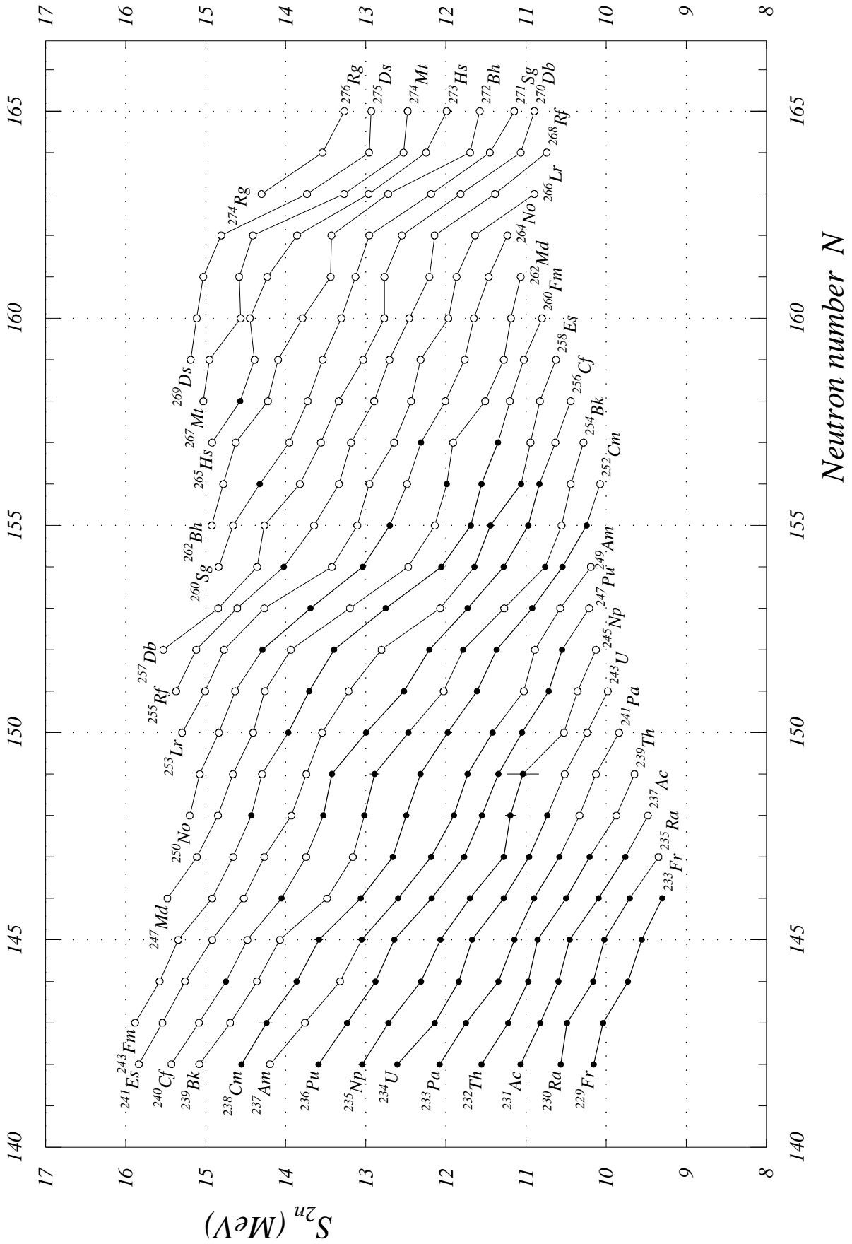
Fig. 8. Two-neutron separation energies N = 142 to 165
