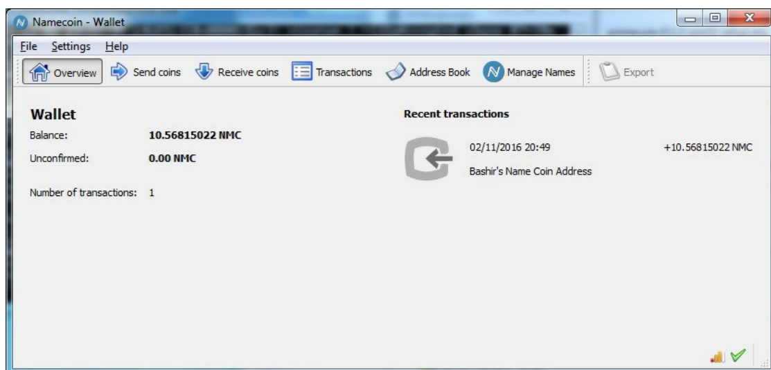
Namecoin wallet
