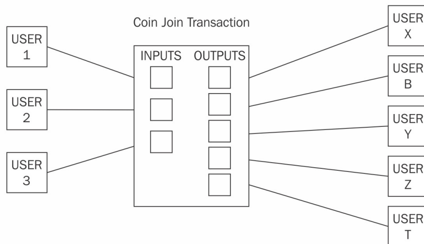
CoinJoin transaction with three users joining their transaction into a single larger CoinJoin transaction
