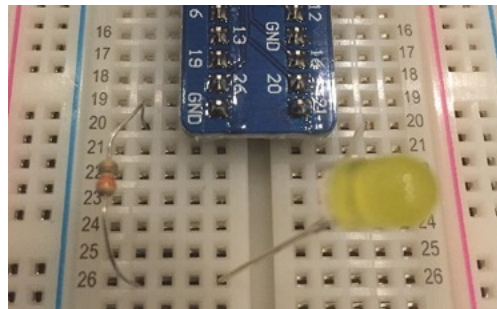
Connections for components on the breadboard
