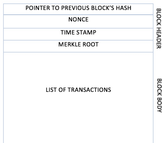
The generic structure of a block.
