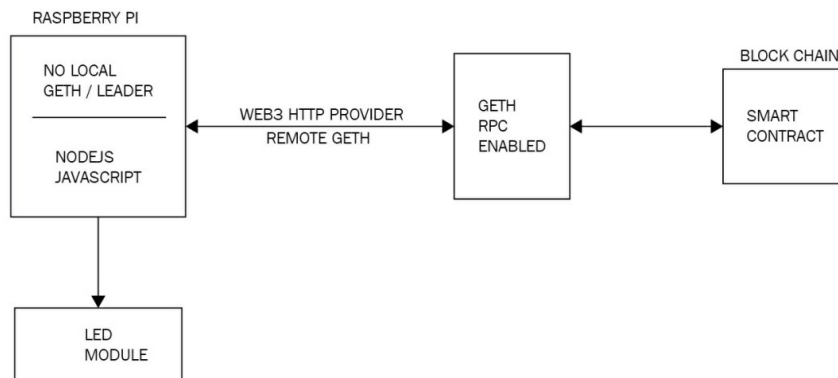
Application architecture of room rent IoT application (IoT device without local ledger)
