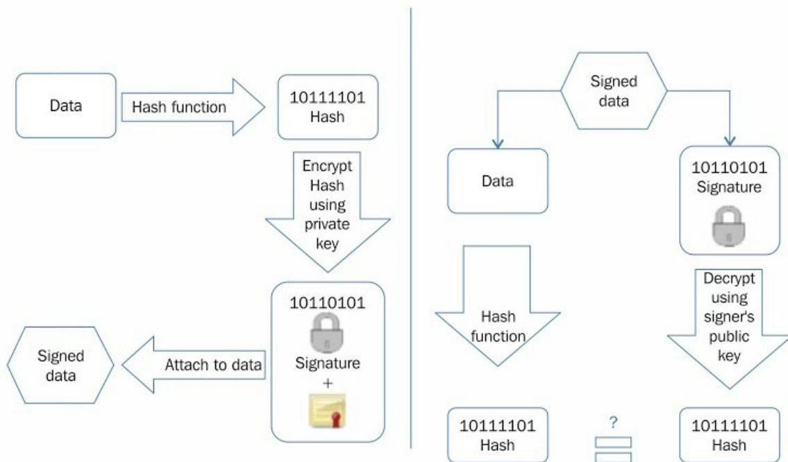
Digital signing (left) and verification process (right) (Example of RSA digital signatures)
