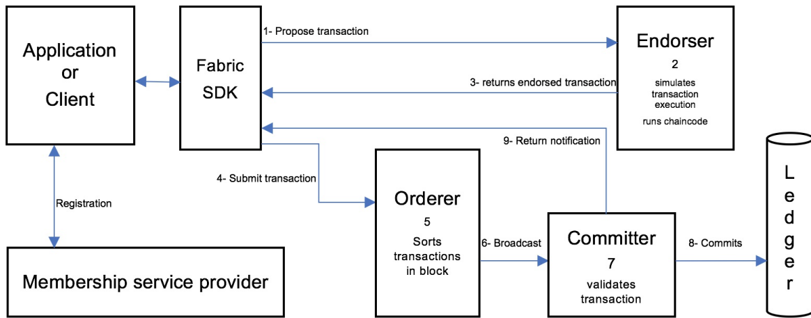
The transaction flow architecture
