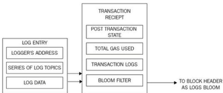
Transaction receipts and logs bloom
