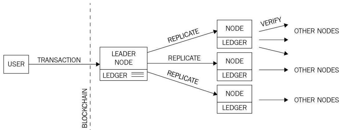
Consensus mechanism in Kadena
