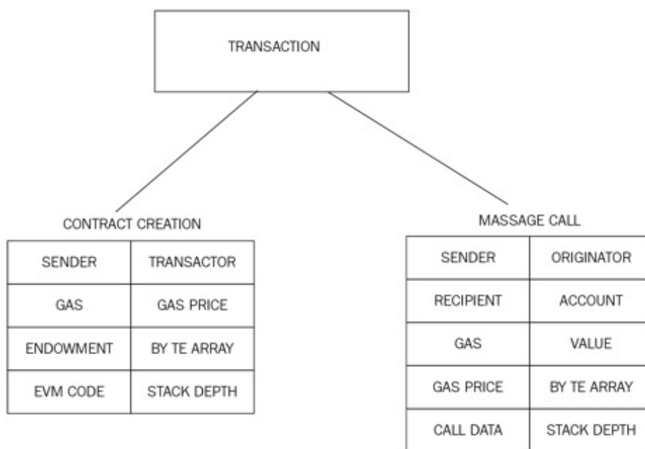
Types of transactions, required parameters for execution
