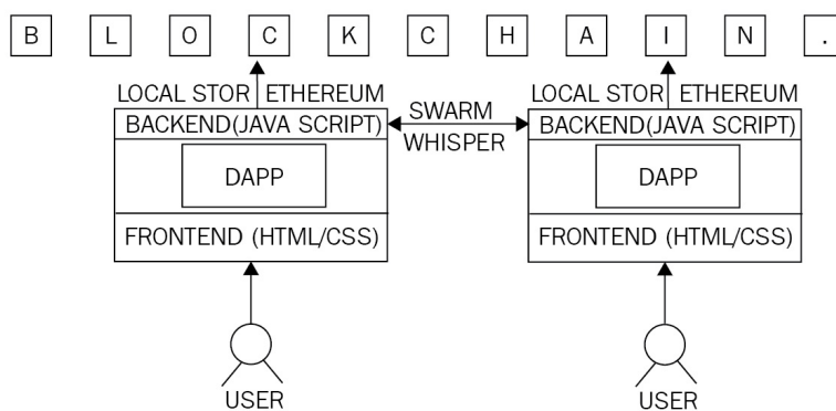
The diagram shows blockchain, Whisper, and Swarm
