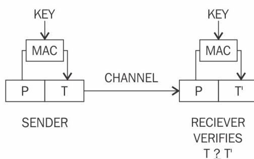
Operation of a MAC function
