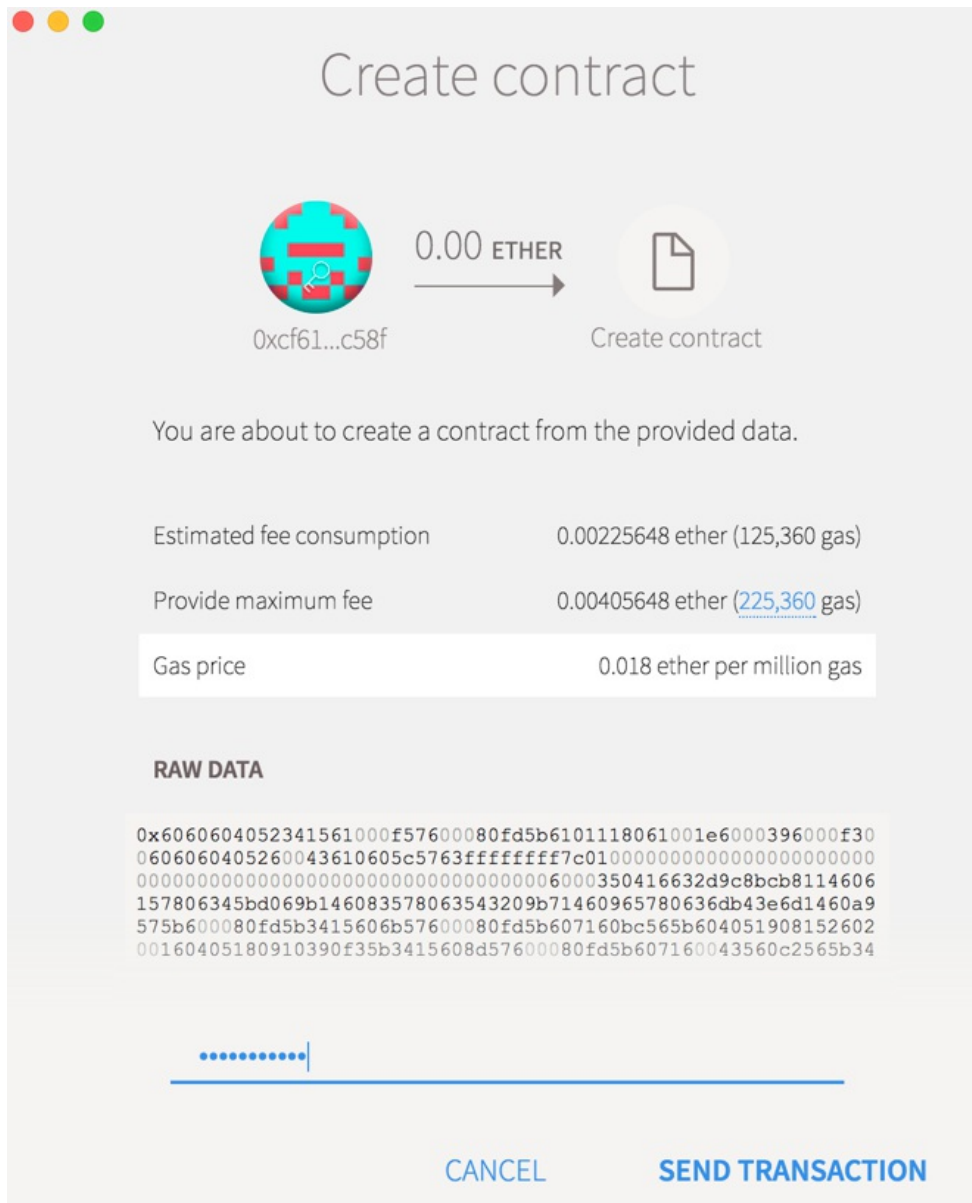
Create a contract using Mist
