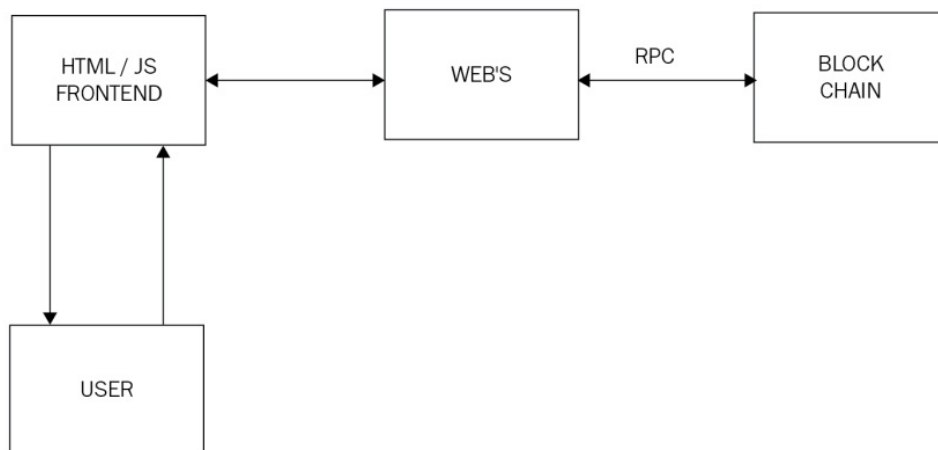
web3.js, frontend, and blockchain interaction architecture
