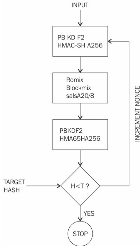
Scrypt ASIC design simplified flowchart
