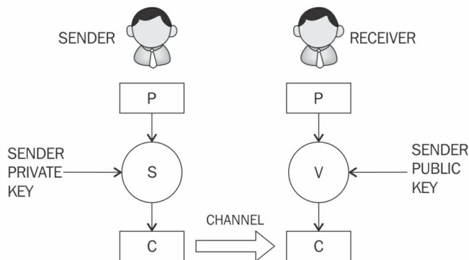
SIGNING & VERIFICATION USING PUBLIC / PRIVATE KEY
