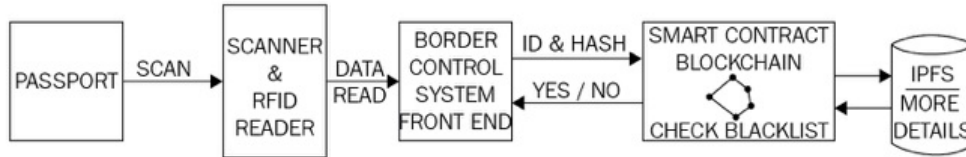
Automated border control using blockchain
