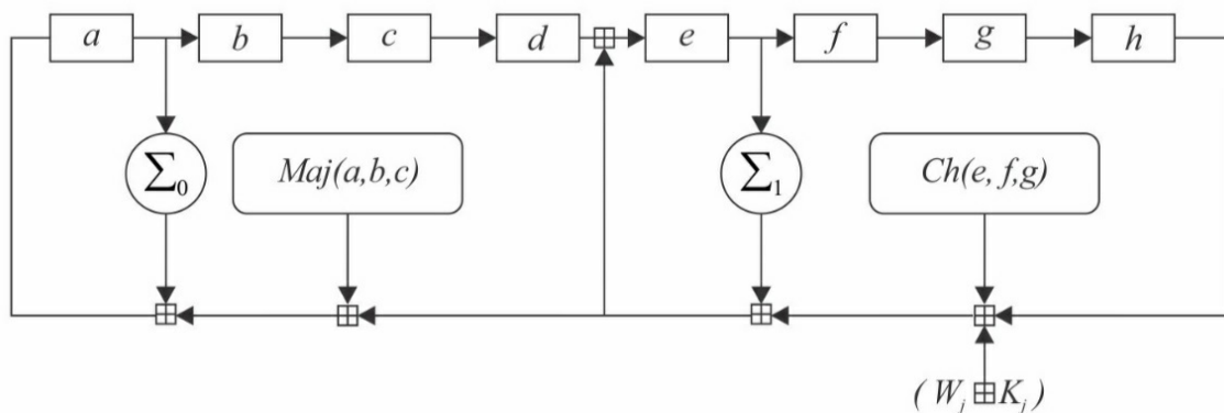
One round of a SHA-256 compression function
