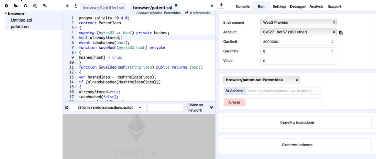
Create contract using browser solidity
