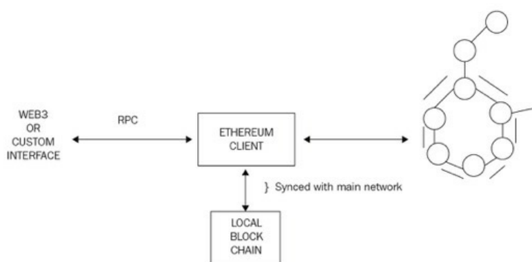
The Ethereum stack showing various components
