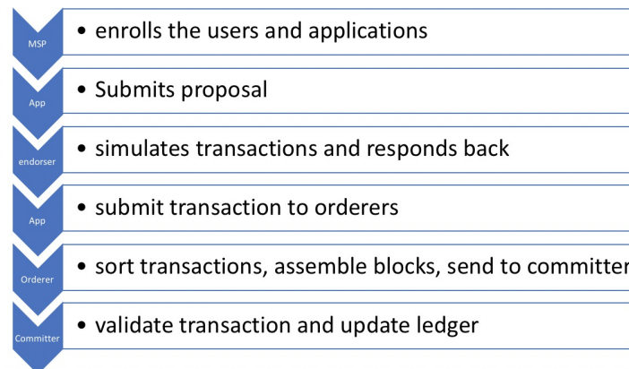
The transaction life cycle
