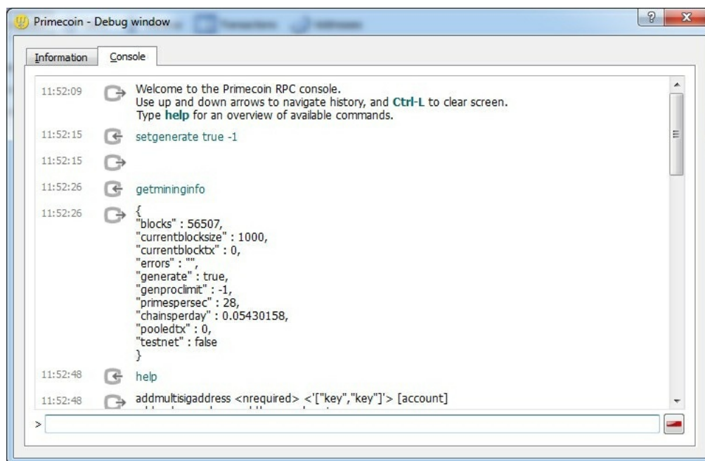
Primecoin mining
