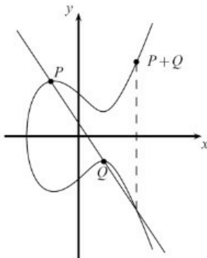
Point addition over R
