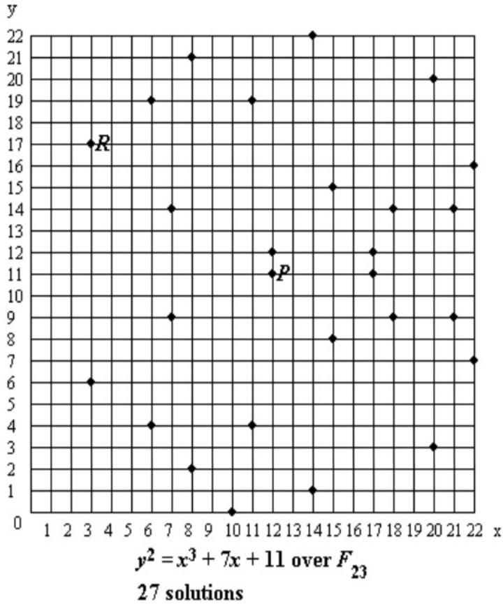
Example of point doubling
