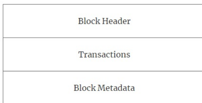
Block structure
