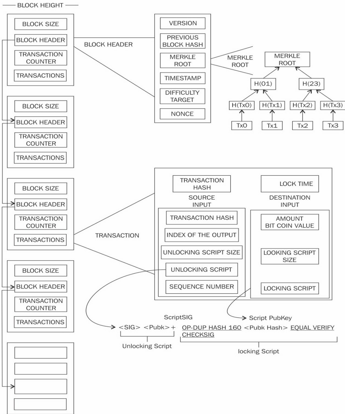
A visualization of the blockchain, block, block header, transactions and scripts
