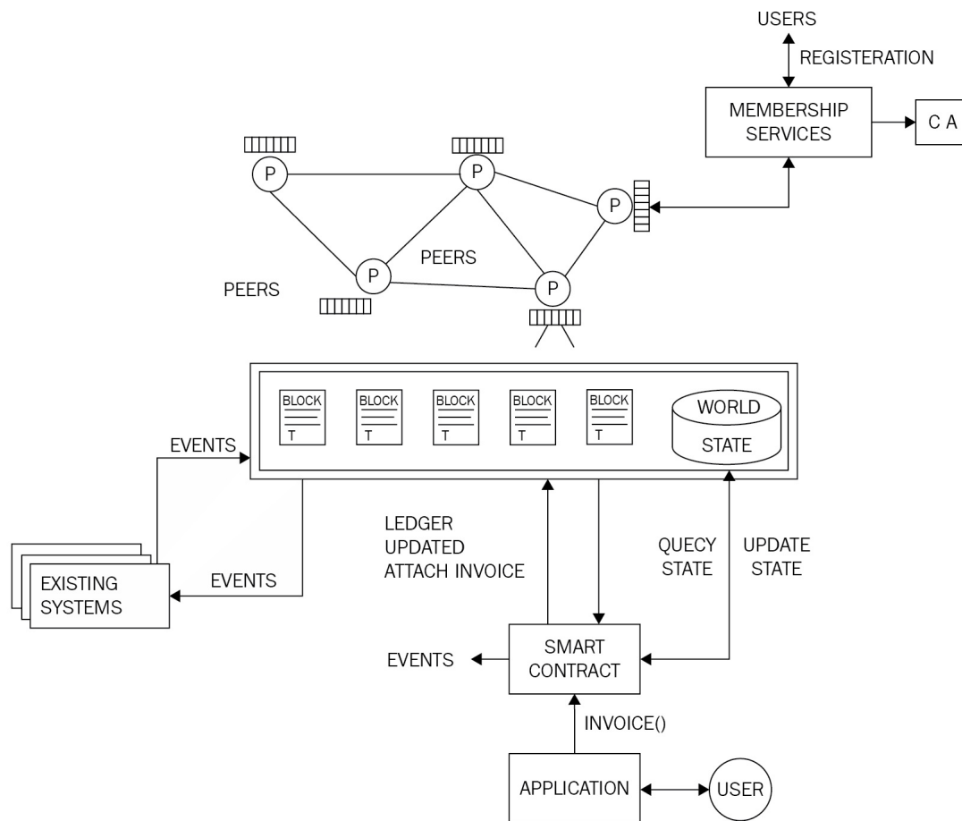
A high-level overview of Hyperledger Fabric
