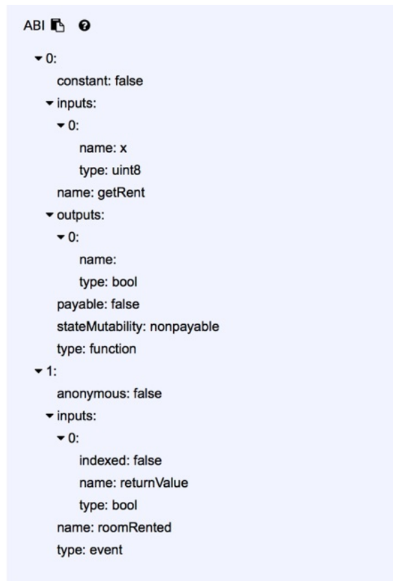
ABI from Remix IDE
