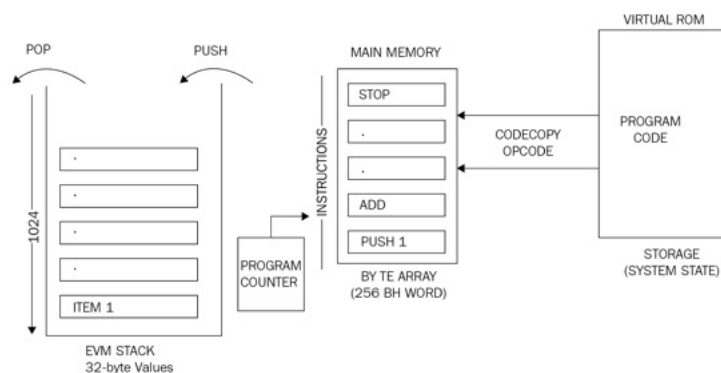
EVM operation
