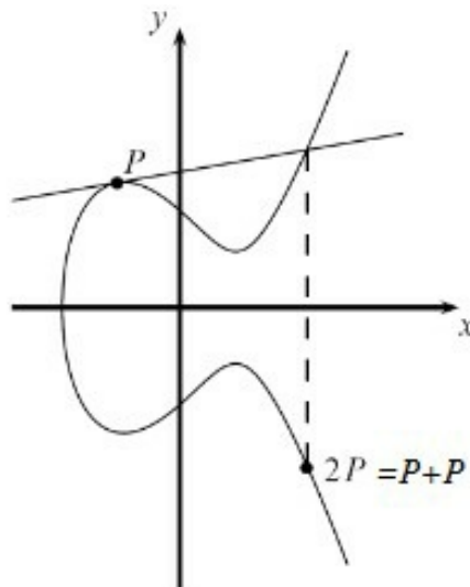
Graph representing point doubling over real numbers
