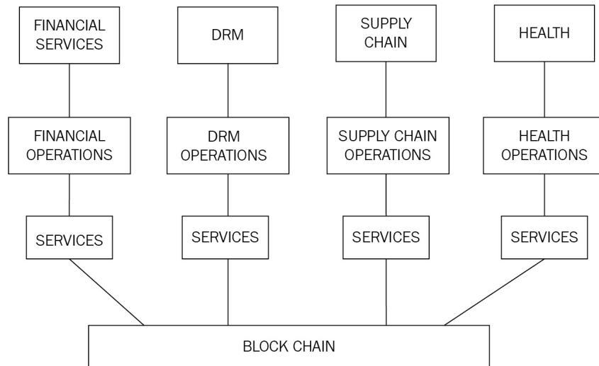
The Sawtooth (transaction families) smart contract paradigm
