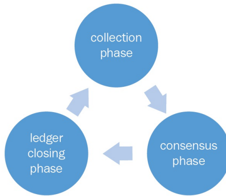
Ripple consensus protocol phases
