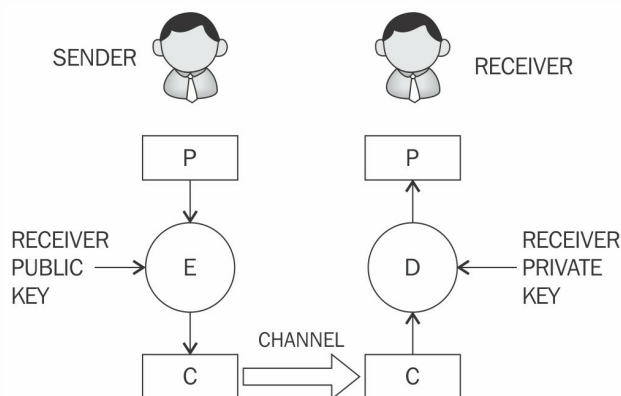
ENCRYPTION DECRYPTION USING PUBLIC / PRIVATE KEY
