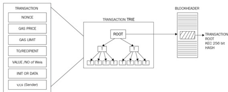
The relationship between transaction, transaction trie and block header
