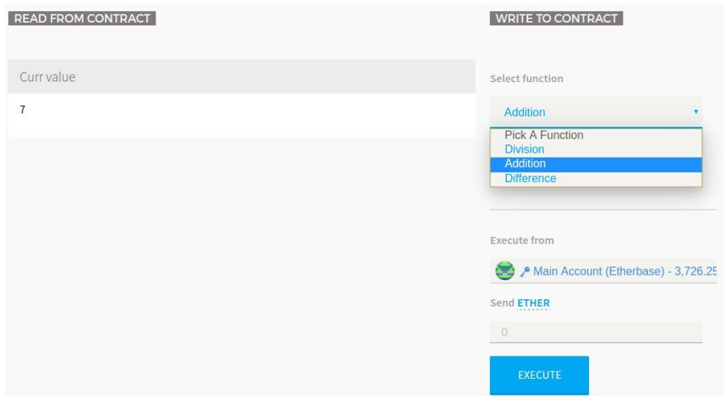
Interaction with the contract using read and write options in Mist
