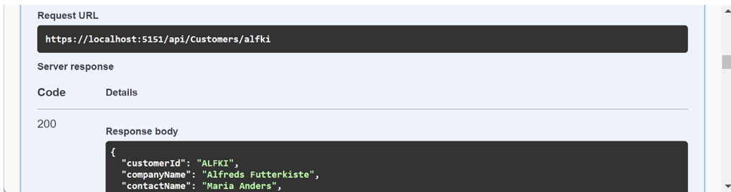
Figure 14.8: Information on ALFKI in a successful Swagger request
