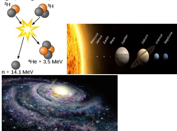
Figure 1 (a) Power of Sun from the fusion 2 hydrogen’s (1 Proton, 1 Neutron) into Helium with excess mass and E=mc^2 (2 protons 2 neutrons); (b) Sun (left), 8 planets: Mercury, Venus, Earth (& moon), Mars, Jupiter, Saturn, Uranus, Neptune (as well as dwarf Planet Pluto; and other comet, meteorites). (c) Milky Way Not in scale.
