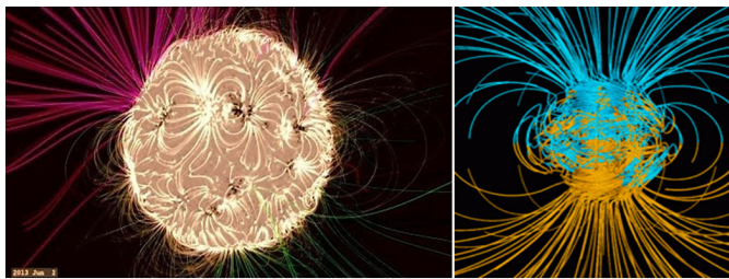
Figure 3 (a) Sun Magnetic field (NASA GSFC, 2013 June 1) simulated (b) the Earth Magnetic Field (noaa.gov).
