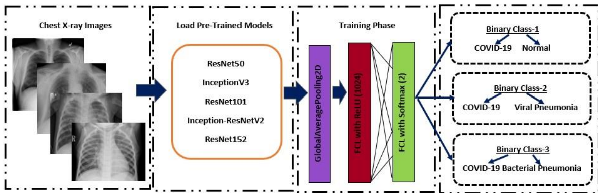
Figure 2. Schematic representation of pre-trained models for the prediction of normal (healthy), COVID-19, bacterial and viral pneumonia patients.
