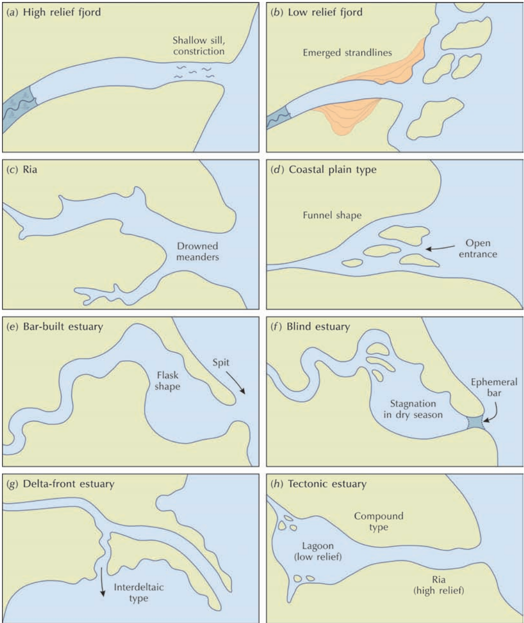
Figure 13.18 Types of estuary: a physiographic classification. Fjords are drowned glacial troughs (p. 268). Rias are erstwhile river valleys drowned by Holocene sea-level rise. They may include mudflats and have barrier spits at their mouths. Coastal plain estuaries are, as their name suggests, estuaries in coastal plains. Bar-built or barrier estuaries have barriers that enclose broad and shallow lagoons. Blind estuaries are closed by an ephemeral bar and stagnate in dry seasons. Delta-front estuaries are associated with river deltas. Tectonic estuaries are formed by folding, faulting, or other tectonic processes. Part of the San Francisco Bay, California, estuary comes under this heading. Source: Adapted from Fairbridge (1980)
