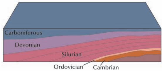
(b) Cambrian–Carboniferous
