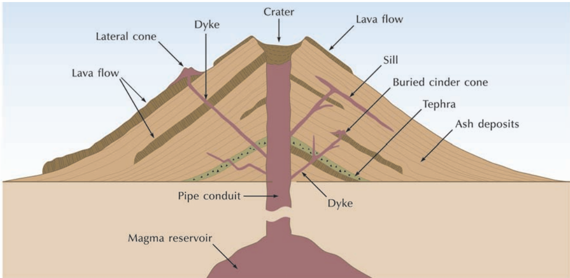
Figure 6.5 The structure of a typical strato-volcano. Source: Adapted from MacDonald (1972, 23)
