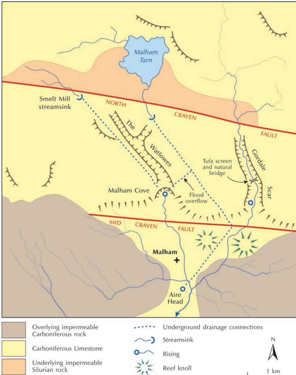
Figure 14.12 Limestone features around Malham Cove, Craven, Yorkshire Dales, England. Compare with Plate 14.15. Source: Adapted from Jennings (1971, 91)
