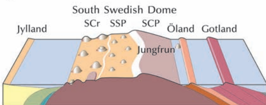
(g) Present
