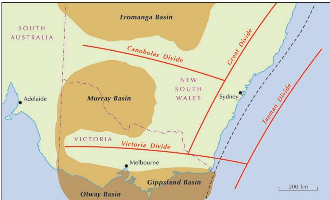
Figure 15.16 Major basins and divides of south-east Australia. The Eromanga Basin is part of the Great Artesian Basin. Source: Adapted from Ollier and Pain (1994)
