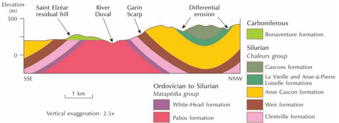
Figure 15.14 Cross-section across the Saint Elzéar region, eastern Quebec, Canada. The palaeosurface, which has been exhumed by erosion, can be seen to the south-south-east of the Garin Scarp cutting across Ordovician and Silurian rocks. Source: Adapted from Jutras and Schroeder (1999)
