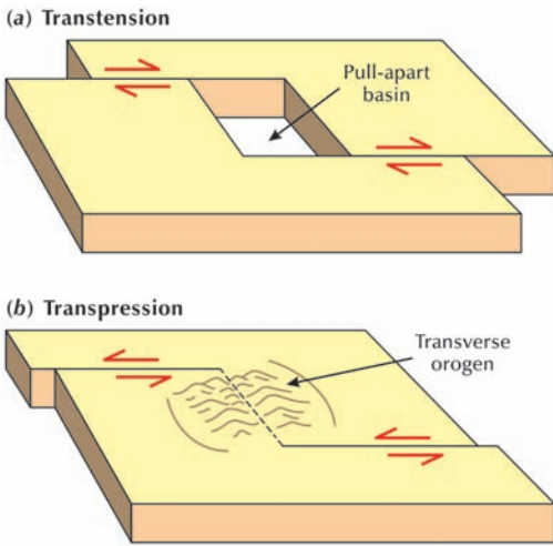
Figure 5.13 Landforms associated with oblique-slip faults. (a) Pull-apart basin formed by transension. (b) Transverse orogen formed by transpression.
