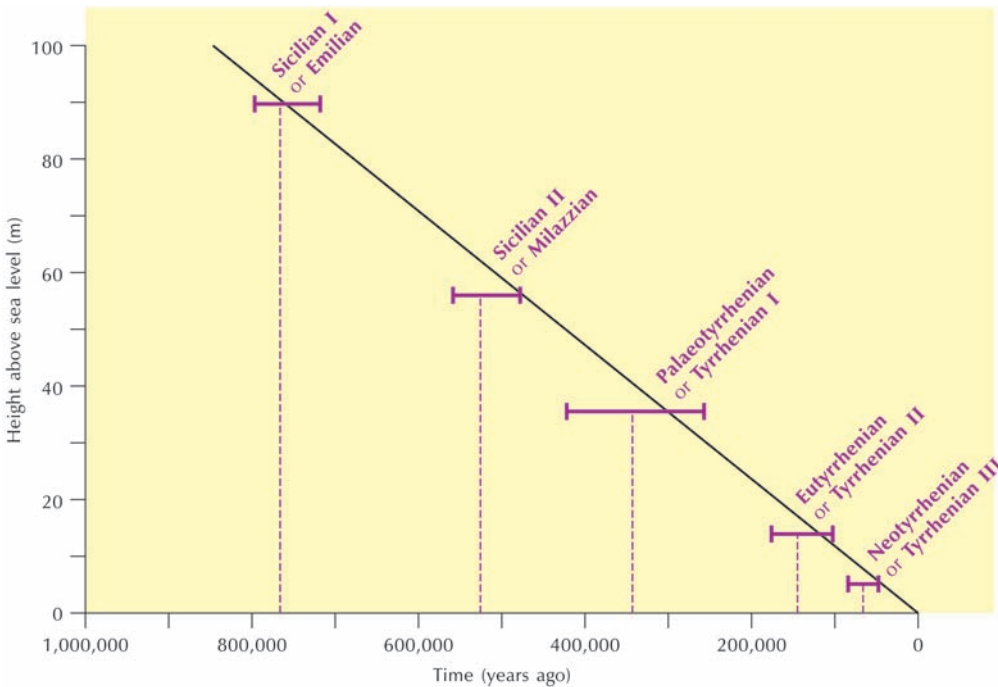
Figure 13.24 Quaternary sea-levels in the Mediterranean: the classic interpretation.
