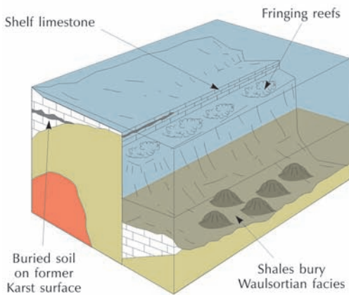
Figure 15.13 Schematic diagram showing the evolution of limestone landscapes in northern England. The Craven Fault, a major east–west fault across the northern Pennines, separates the Askrigg tilt-block from the Craven Deep. Source: Adapted from Douglas (1987)
