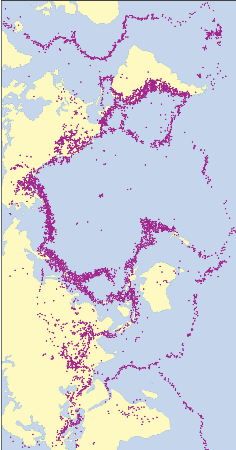
Figure 5.6 Global distribution of earthquakes. Source: Adapted from Ollier (1996)
