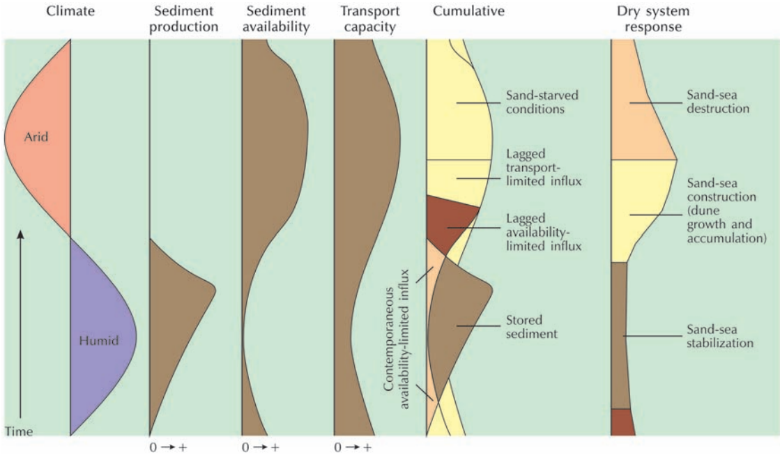
Figure 12.13 Process–response model for Saharan sand seas based on sediment production, sediment availability (supply), and transport capacity. The system is driven by a climatic cycle from humid to arid, shown on the left. An explanation is given in the text. Source: Adapted from Kocurek (1998)
