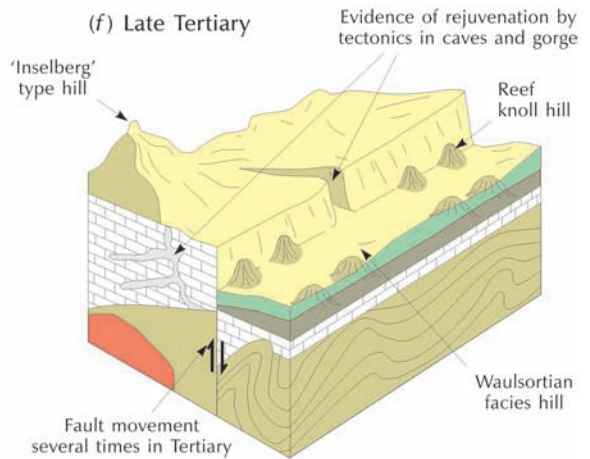
Figure 15.13 Schematic diagram showing the evolution of limestone landscapes in northern England. The Craven Fault, a major east–west fault across the northern Pennines, separates the Askrigg tilt-block from the Craven Deep. Source: Adapted from Douglas (1987)
