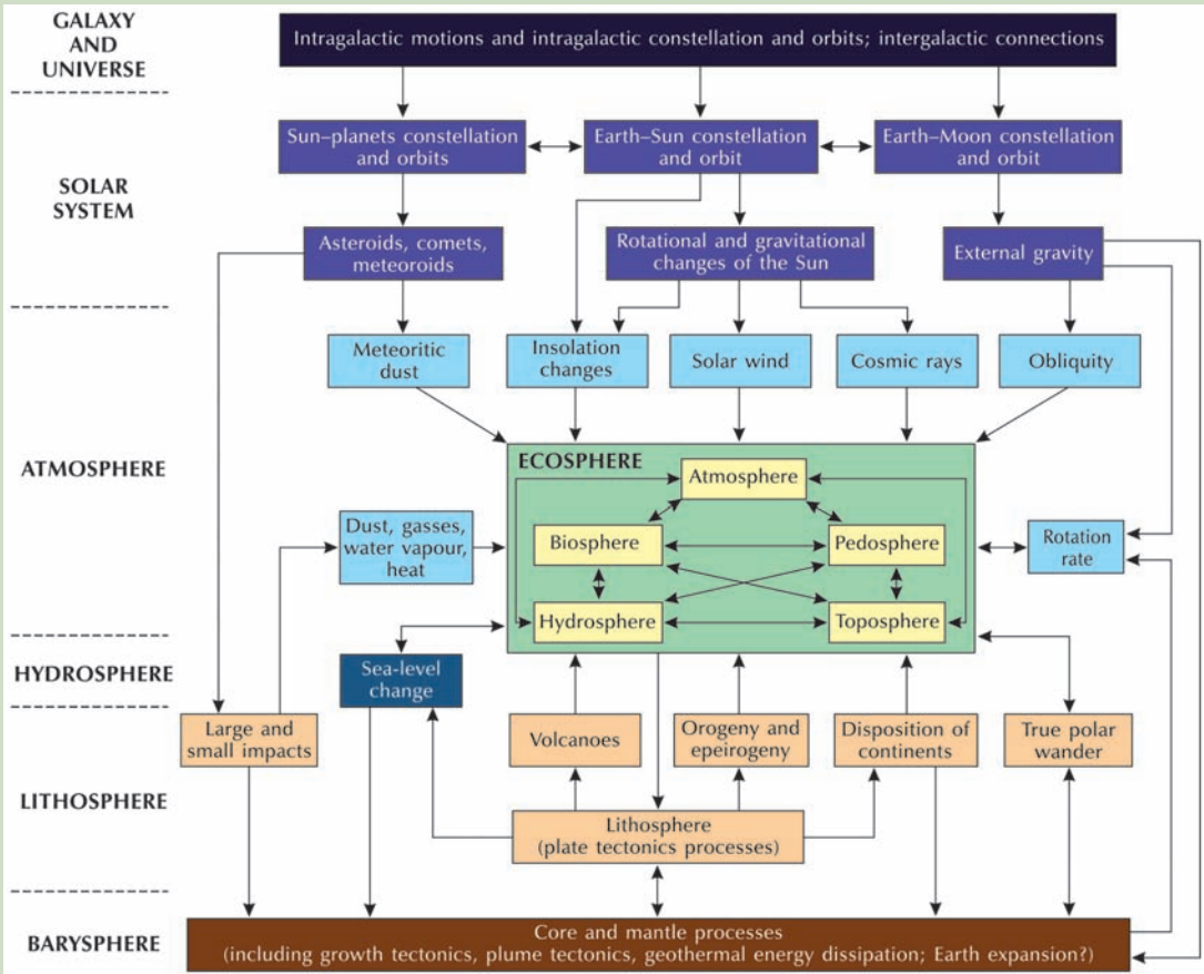
Figure 4.3 Interacting terrestrial spheres and their cosmic and geological settings. Source: Adapted from Huggett (1991, 1995, 1997b)
