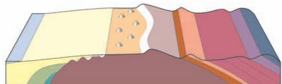
(f) Mid-Miocene–Pliocene
