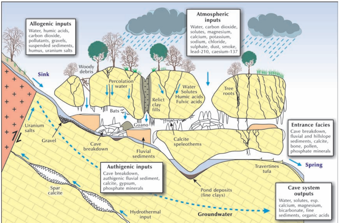
Figure 14.17 The cave system. Source: Adapted from Gillieson (1996, 7)
