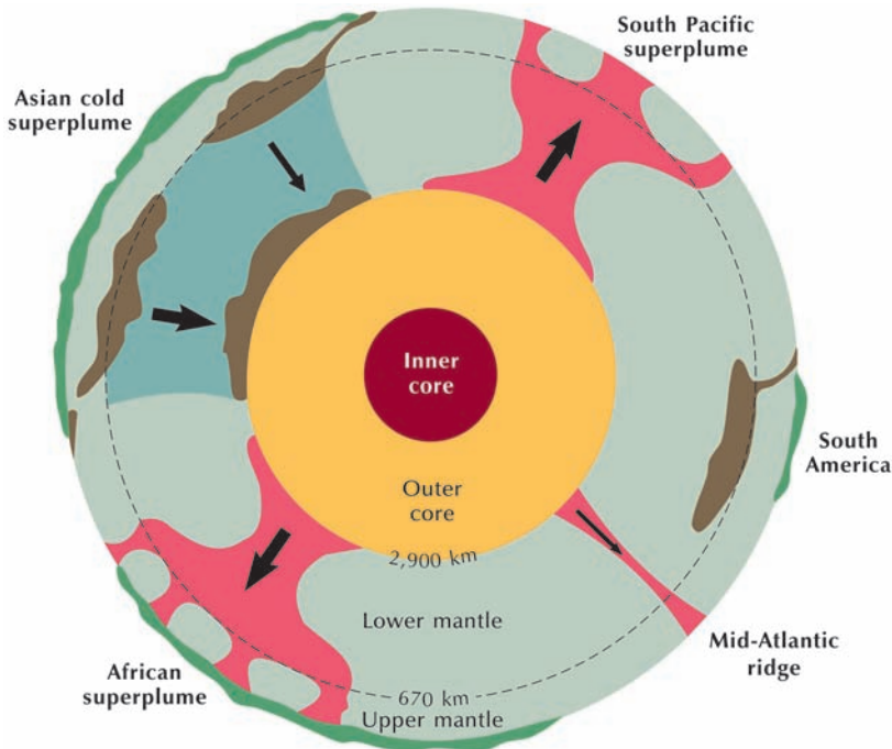
Figure 5.7 A possible grand circulation of Earth materials. Oceanic lithosphere, created at mid-ocean ridges, is subducted into the deeper mantle. It stagnates at around 670 km and accumulates for 100–400 million years. Eventually, gravitational collapse forms a cold downwelling on to the outer core, as in the Asian cold superplume, which leads to mantle upwelling occurring elsewhere, as in the South Pacific and African hot superplumes. Source: Adapted from Fukao et al. (1994)
