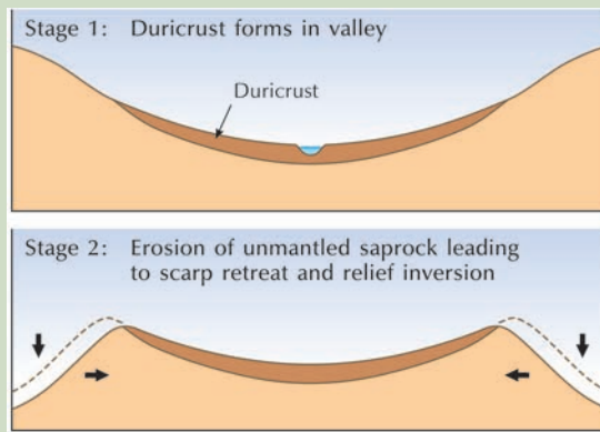
Figure 7.4 Development of inverted relief associated with duricrust formation.
