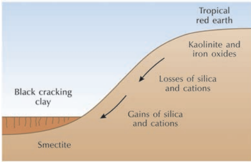
Figure 7.9 Clay types in a typical tropical toposequence. Source: Adapted from Ollier and Pain (1996, 141)
