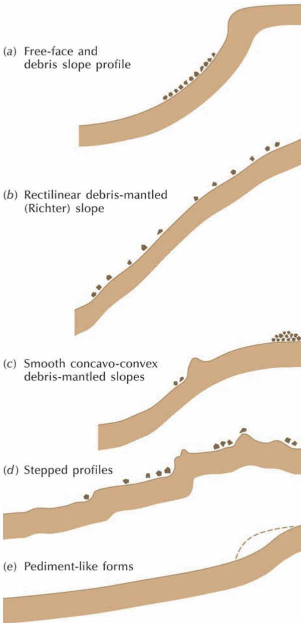
Figure 11.6 Types of periglacial slopes. (a) Cliff above a debris slope. (b) Rectilinear, debris-mantled or Richter slope. (c) Smooth concavo-convex profile with frost-shattered and solifluction debris. (d) Stepped profiles: cryoplanation or altiplanation terraces. (e) Pediment-like forms, or cryopediments. Source: Adapted from French (2007, 217)
