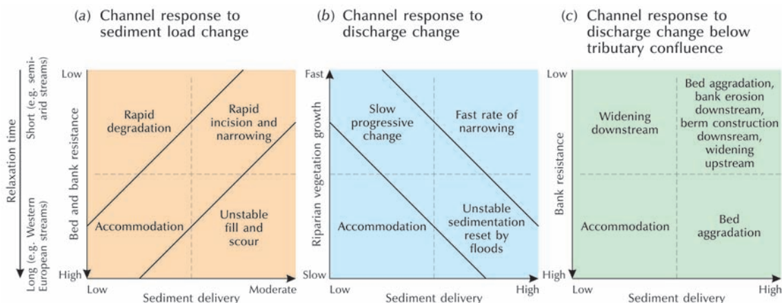
Figure 9.27 Domains of channel change in response to changing sediment load and discharge in different regions. Responses are to (a) A dominant reduction in sediment loads, (b) A dominant reduction in floods. (c) The special case of channel change below a tributary confluence in a regulated river dominated by flood reduction. Source: Adapted from Petts and Gurnell (2005)
