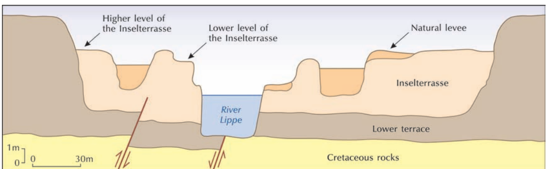
Figure 9.30 Schematic cross-section of the lower Lippe Valley in north-west Germany, showing terraces. Source: Adapted from Herget (1998)
