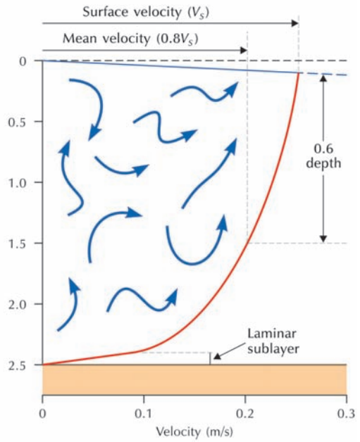
Figure 9.2 Velocity profiles of (a) laminar and (b) turbulent flow in a river.
