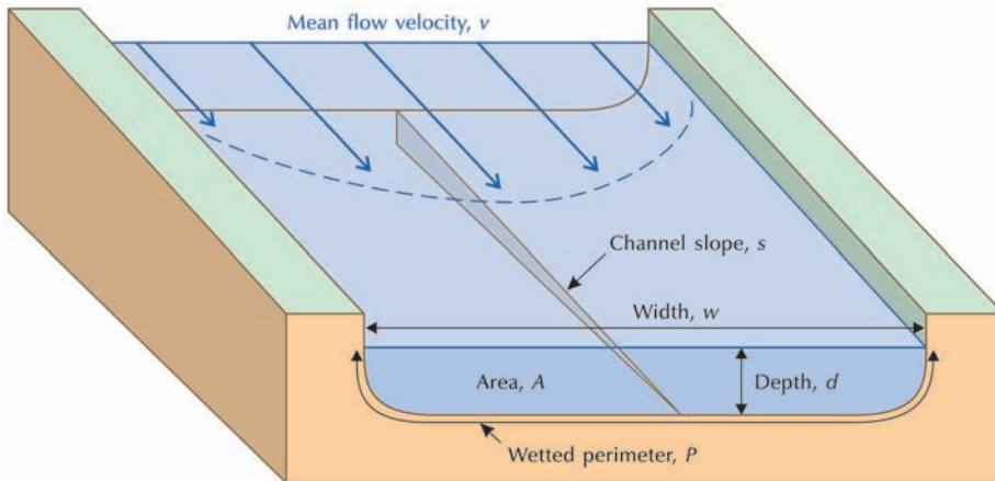
Figure 9.3 Variables used in describing streamflow.
