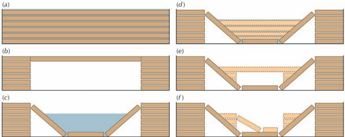
Figure 1.4 Steno's six-stage landscape history of the Tuscan region. First, just after Creation, the region was covered by a 'watery fluid', out of which inorganic sediments precipitated to form horizontal, homogeneous strata. Second, the newly formed strata emerged from their watery covering to form a single, continuous plain of dry land, beneath which the force of fires or water ate out huge caverns. Third, some of the caverns might have collapsed to produce valleys, into which rushed the waters of the Flood. Fourth, new strata of heterogeneous materials containing fossils were deposited in the sea, which now stood at higher level than it had prior to the Flood and occupied the valleys. Fifth, the new strata emerged when the Flood waters receded to form a huge plain, and were then undermined by a second generation of caverns. Finally, the new strata collapsed into the cavities eaten out beneath them to produce the Earth's present topography in the region. Source: Adapted from Steno (1916 edn)
