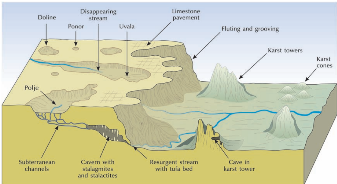
Figure 14.5 Schematic diagram of some karst features.
