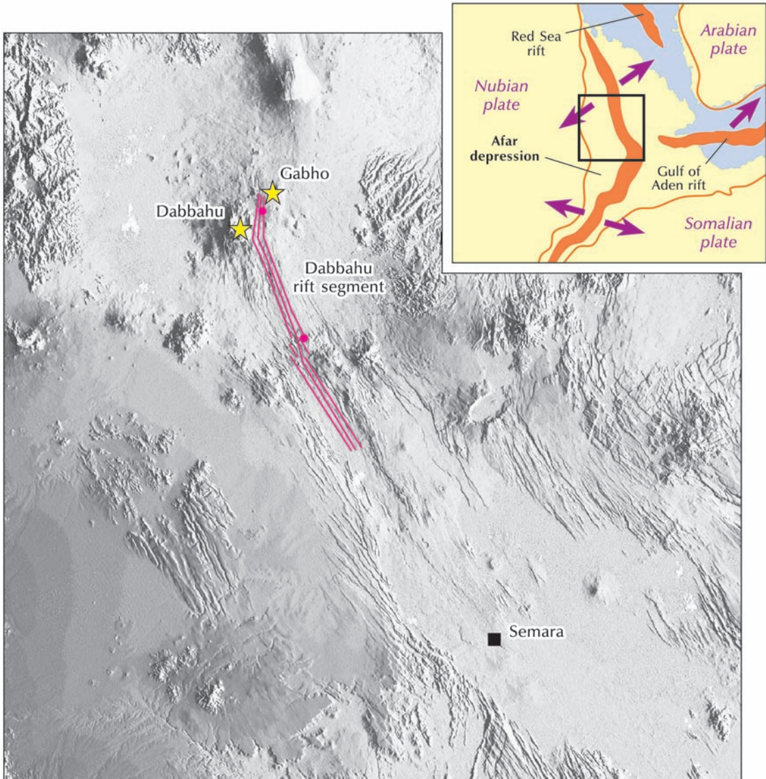
Figure 5.1 Topographic relief of the 60-km-long Dabbahu rift segment within the Afar Depression. The inset shows directions of plate divergence between the stable African (Nubian), Arabian, and Somalian plates. Source: Adapted from Cynthia Ebinger, Royal Holloway, University of London.
