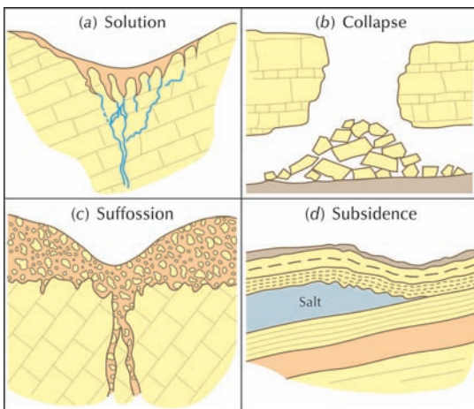
Figure 14.7 The main genetic classes of doline. (a) Solution doline. (b) Collapse doline. (c) Suffosion doline. (d) Subsidence doline. Source: Adapted from Ford and Williams (1989, 398)
