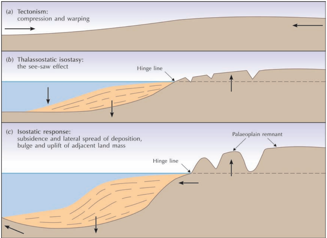
Figure 15.15 Sequence of events following a marine incursion into an Australian cratonic basin, and consequent uplift of adjacent land. Source: Adapted from Twidale (1994)
