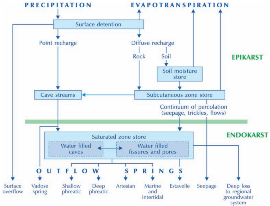
Figure 14.4 The karst drainage system: storages and flows. Source: Adapted from Ford and Williams (1989, 169)
