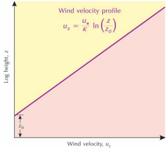
Figure 12.2 Wind velocity profile. Note that the relationship between wind velocity and height is a straight line because the height axis is logarithmic; in the diagram showing the velocity profile in water (Figure 9.2), the height axis is arithmetic and the relationship is a curve.
