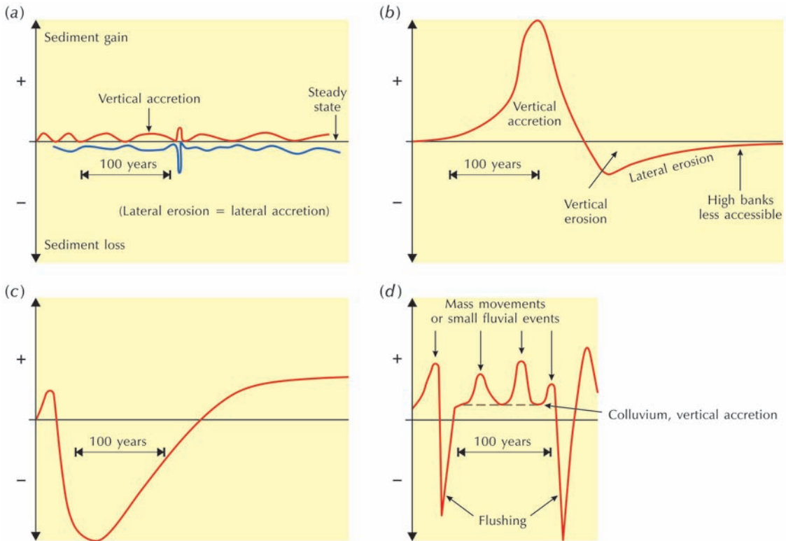
Figure 9.7 Four common patterns of valley sediment storage and flux under natural conditions. (a) Quasi-steady-state typical of humid regions. (b) Great sediment influx with later amelioration producing vertical accretion of channels and aggradation of floodplains. (c) Valley trenching (arroyo cutting). (d) High-energy instability seen as episodic gains and losses in mountain and arid streams. Source: Adapted from Trimble (1995)
