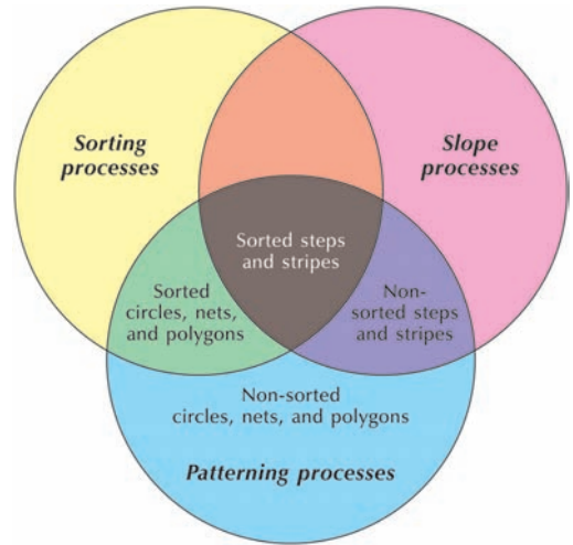
Figure 11.5 Relationships between patterned ground and sorting processes, slope processes, and patterning processes. Source: Adapted from Washburn (1979, 160)
