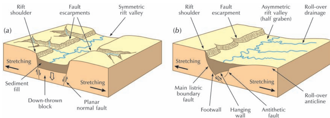
Figure 6.18 Down-faulted structures. (a) Graben. (b) Half-graben. Source: After Summerfield (1991, 92)
