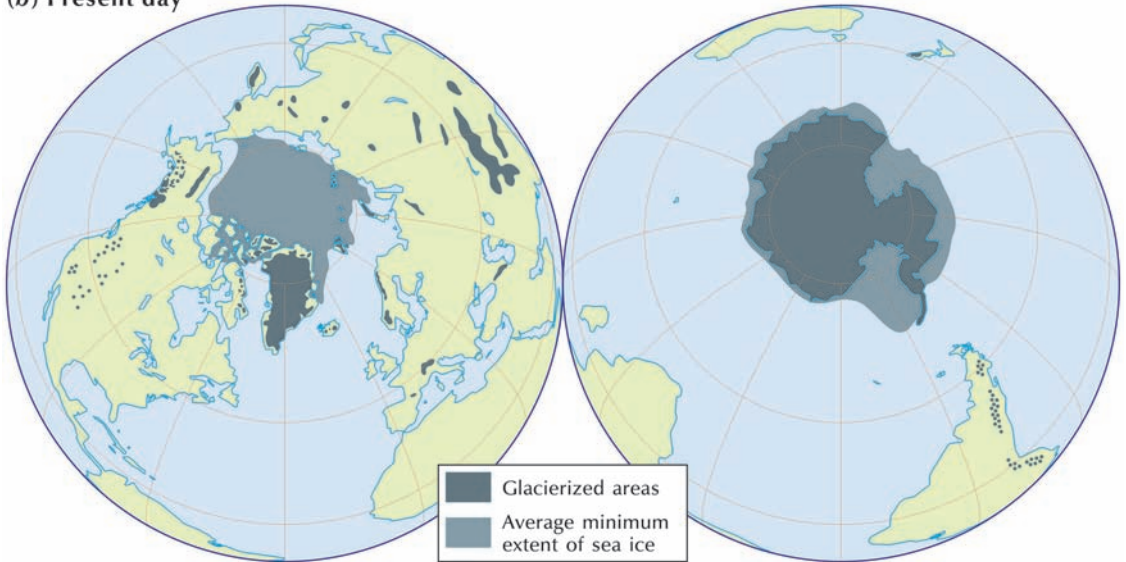
Figure 10.1 Distribution of ice.
