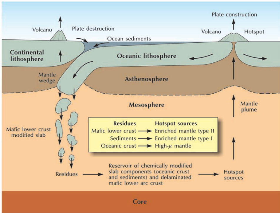
Figure 5.3 Interactions between the asthenosphere, lithosphere, and mesosphere. The oceanic lithosphere gains material from the mesosphere (via the asthenosphere) at constructive plate boundaries and hotspots and loses material to the mesosphere at destructive plate boundaries. Subduction feeds slab material (oceanic sediments derived from the denudation of continents and oceanic crust), mantle lithosphere, and mantle wedge materials to the deep mantle. These materials undergo chemical alteration and accumulate in the deep mantle until mantle plumes bear them to the surface, where they form new oceanic lithosphere. Source: Adapted from Tatsumi (2005)
