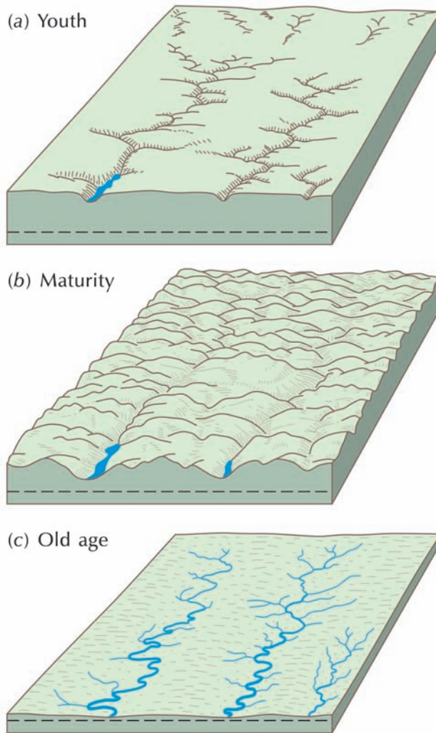
Figure 1.6 William Morris Davis's idealized 'geographical cycle' in which a landscape evolves through 'life-stages' to produce a peneplain. (a) Youth: a few 'consequent' streams (p. 214), V-shaped valley cross-sections, limited floodplain formation, large areas of poorly drained terrain between streams with lakes and marshes, waterfalls and rapids common where streams cross more resistant beds, stream divides broad and ill-defined, some meanders on the original surface. (b) Maturity: well-integrated drainage system, some streams exploiting lines of weak rocks, master streams have attained grade (p. 211), waterfalls, rapids, lakes, and marshes largely eliminated, floodplains common on valley floors and bearing meandering rivers, valley no wider than the width of meander belts, relief (difference in elevation between highest and lowest points) is at a maximum, hillslopes and valley sides dominate the landscape. (c) Old age: trunk streams more important again, very broad and gently sloping valleys, floodplains extensive and carrying rivers with broadly meandering courses, valleys much wider than the width of meander belts, areas between streams reduced in height and stream divides not so sharp as in the maturity stage, lakes, swamps, and marshes lie on the floodplains, mass-wasting dominates fluvial processes, stream adjustments to rock types now vague, extensive areas lie at or near the base level of erosion. Source: Adapted from Holmes (1965, 473)
