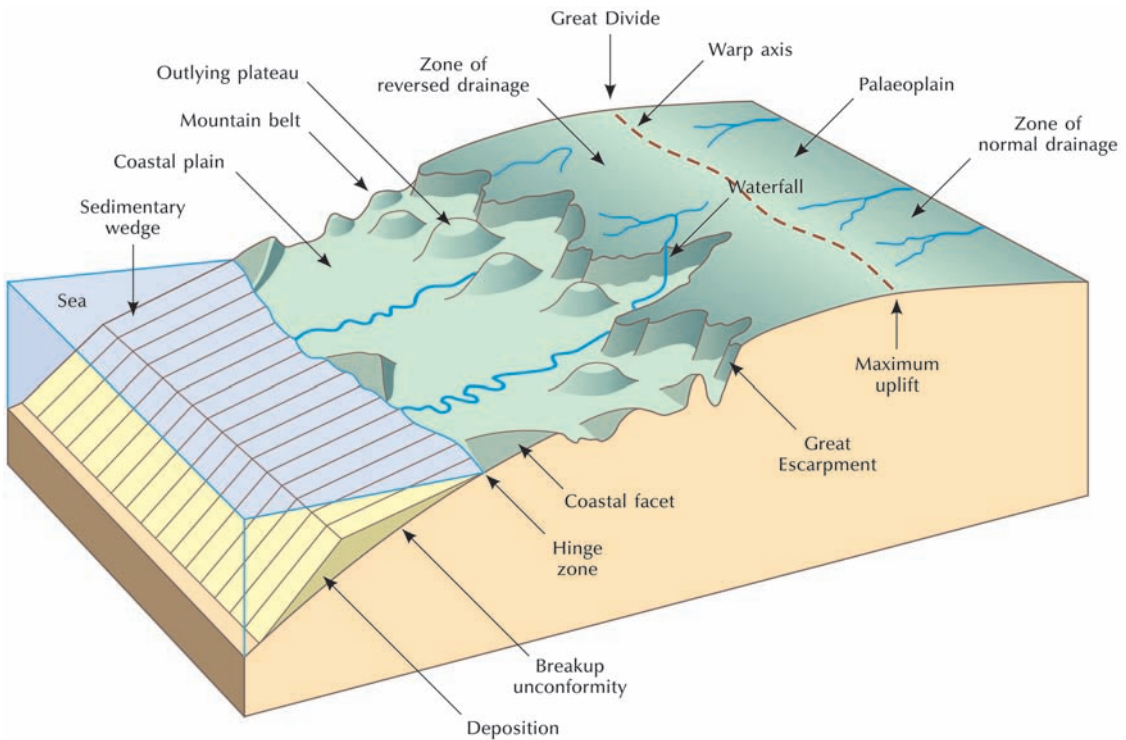
Figure 5.8 The chief morphotectonic features of a passive continent margin with mountains. Source: Adapted from Ollier and Pain (1997)
