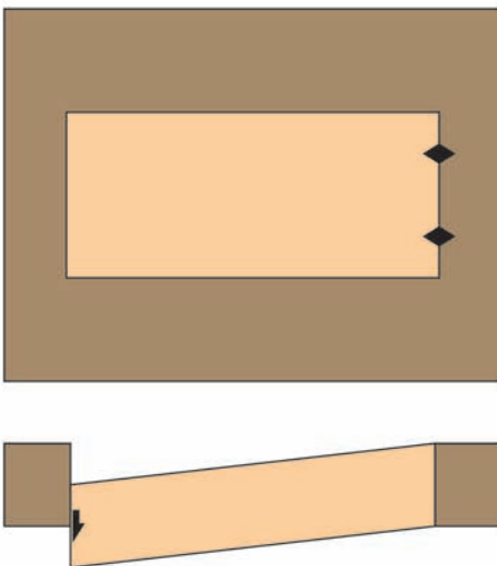
(c) Trapdoor
