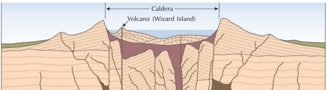
Figure 6.8 Crater Lake caldera, Oregon, USA; see Plate 6.5. Source: Adapted from MacDonald (1972, 301)
