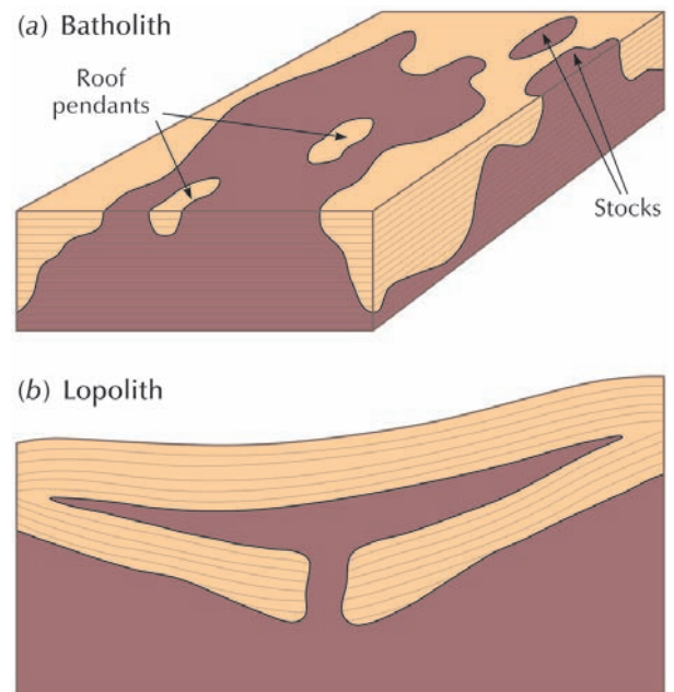
Figure 6.1 Major intrusions. (a) Batholith with stocks and roof pendants. (b) Lopolith. Source: Adapted from Sparks (1971, 68, 90)
