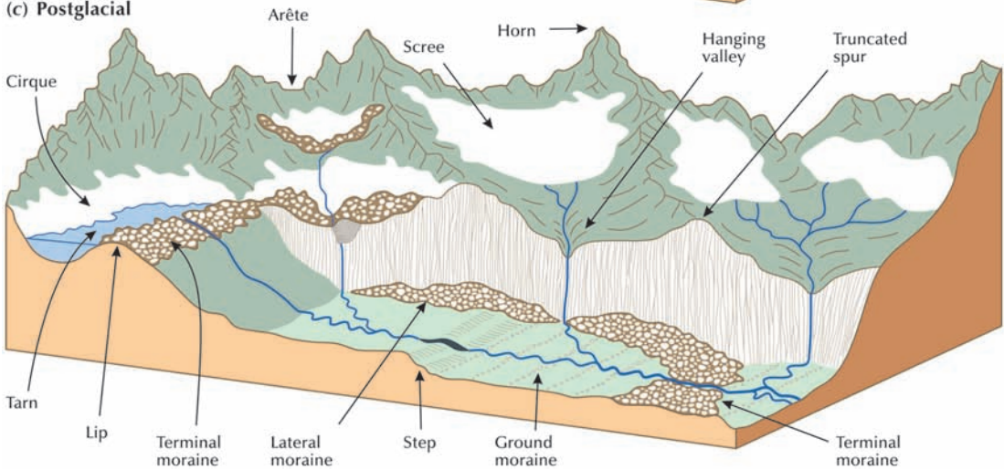
(c) Postglacial
