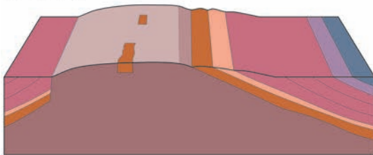
(c) Permian
