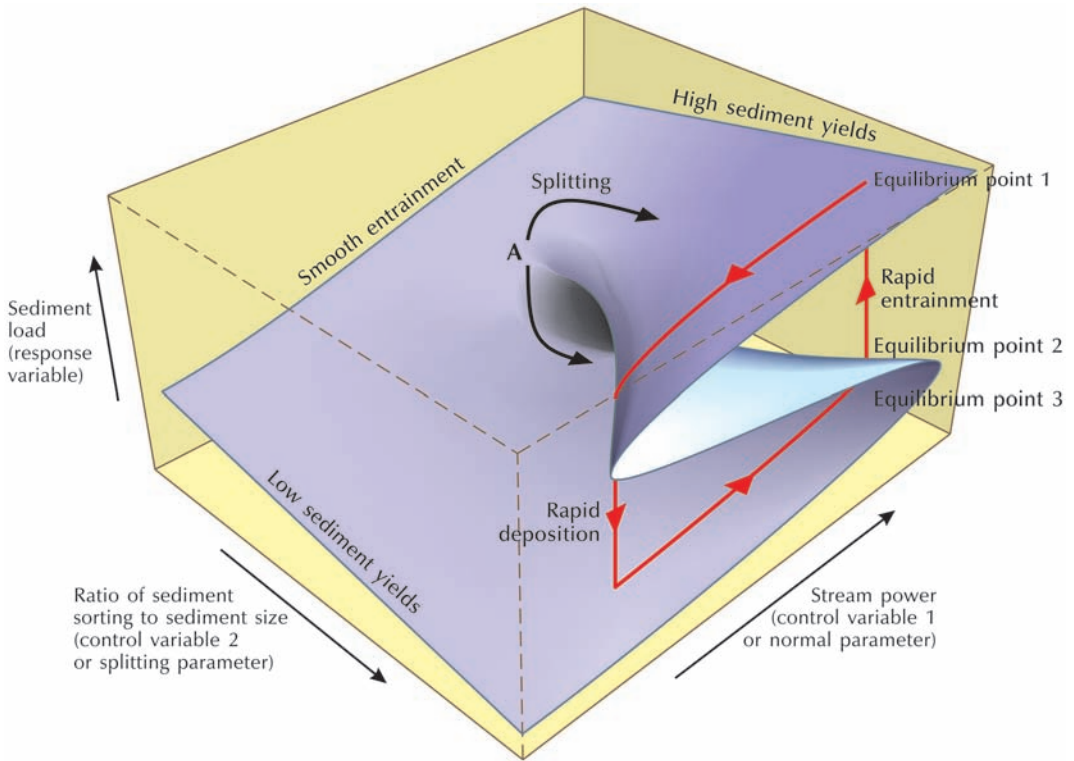
Figure 2.5 A cusp catastrophe model applied to sediment transport in a river. Source: Adapted from Thornes (1983)
