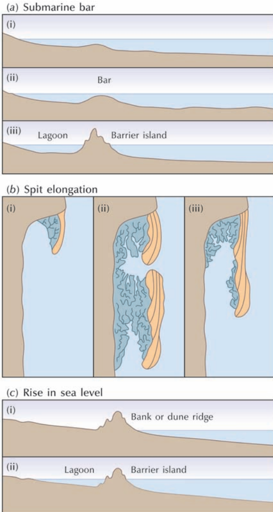
Figure 13.13 Ways in which barrier islands may form. (a) The growth of a submarine bar. (b) The elongation of a spit. (c) The submergence of a beach ridge or dunes by a rising sea-level. Source: Adapted from Hoyt (1967)
