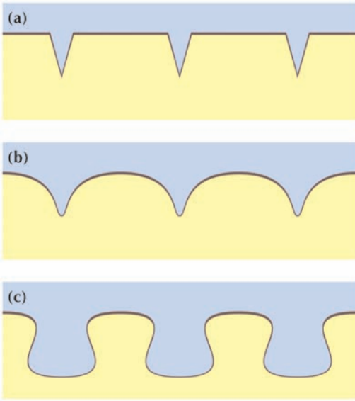
Figure 14.16 Proposed sequence of events leading to 'bollard' rock formation in quartzitic sandstone, north-central Thailand. (a) Polygonal cracks develop in a case-hardened surface that act as avenues of weathering. (b) Weathering deepens the cracks, forming a convex surface on each polygonal block. (c) Further weathering removes the edges of the polygonal blocks and deepens and widens the cracks. Source: Adapted from Robinson and Williams (1992) and Doerr (2000)
