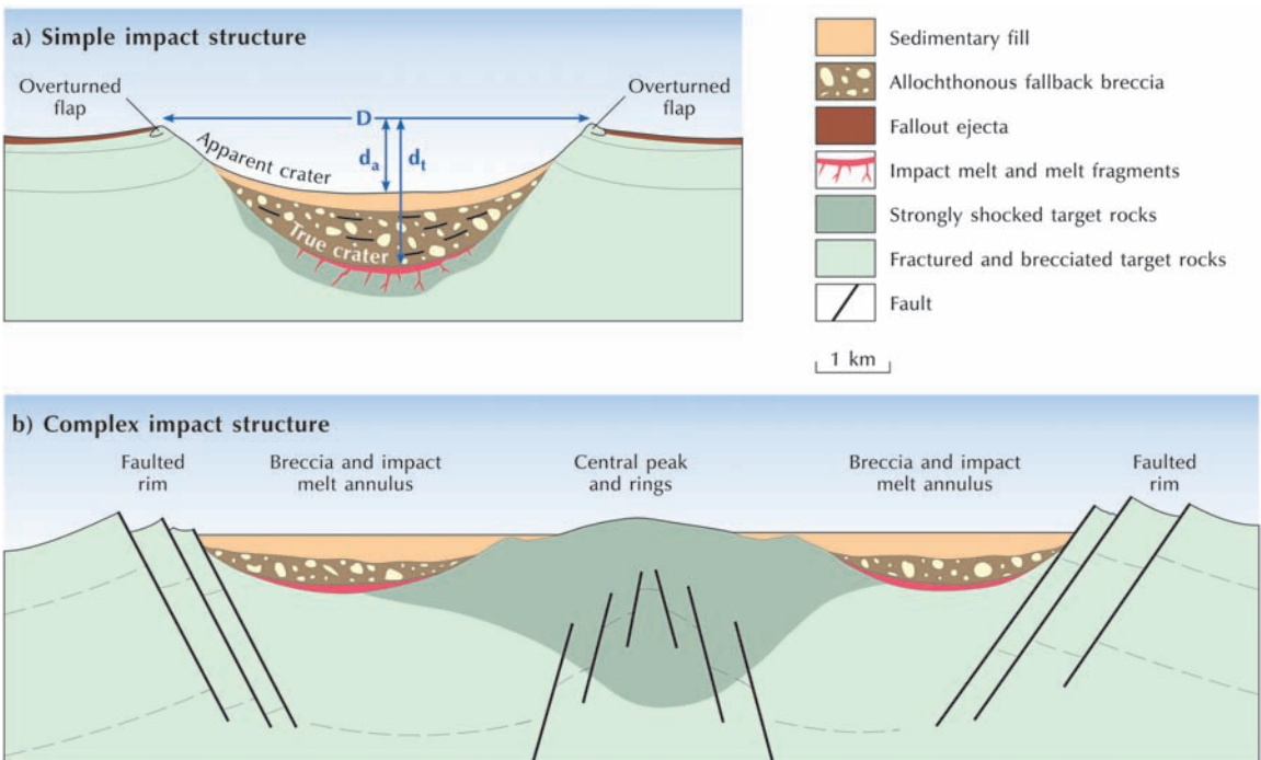
Figure 6.11 Simple and complex impact structures.
