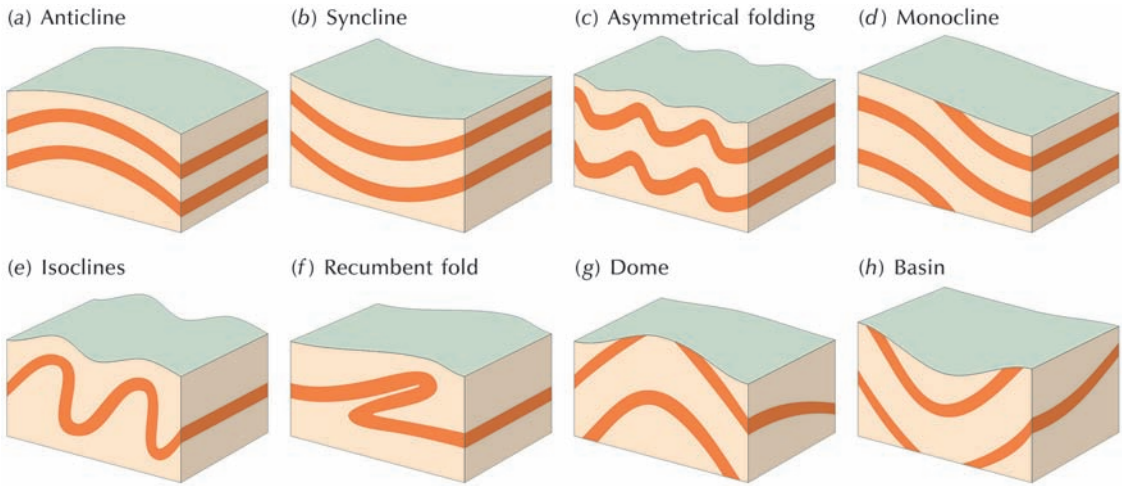
Figure 6.13 Structures formed in folded strata.
