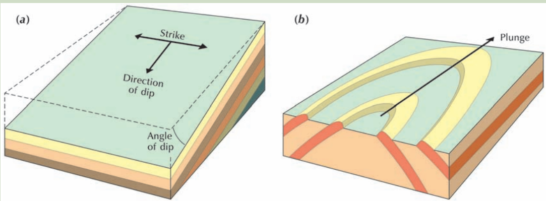
Figure 6.14 Terms relating to sedimentary structures. (a) Dip and strike. (b) Plunge.
