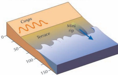
Figure 13.9 Beach types classified by wave and tide dominance. Source: Adapted from Short (2006, 2010) and Short and Woodroffe (2009)
