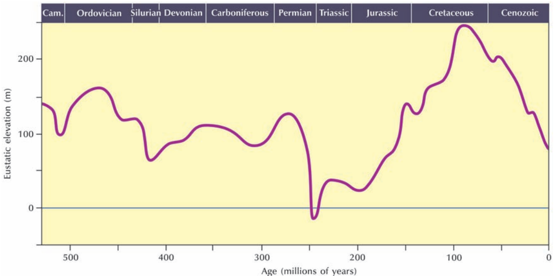
Figure 13.23 Proposed Phanerozoic eustatic curve. Sources: The Palaeozoic section is adapted from an average estimated by Algeo and Sessler (1995) and the Mesozoic and Cenozoic portion is adapted from Haq et al. (1987)
