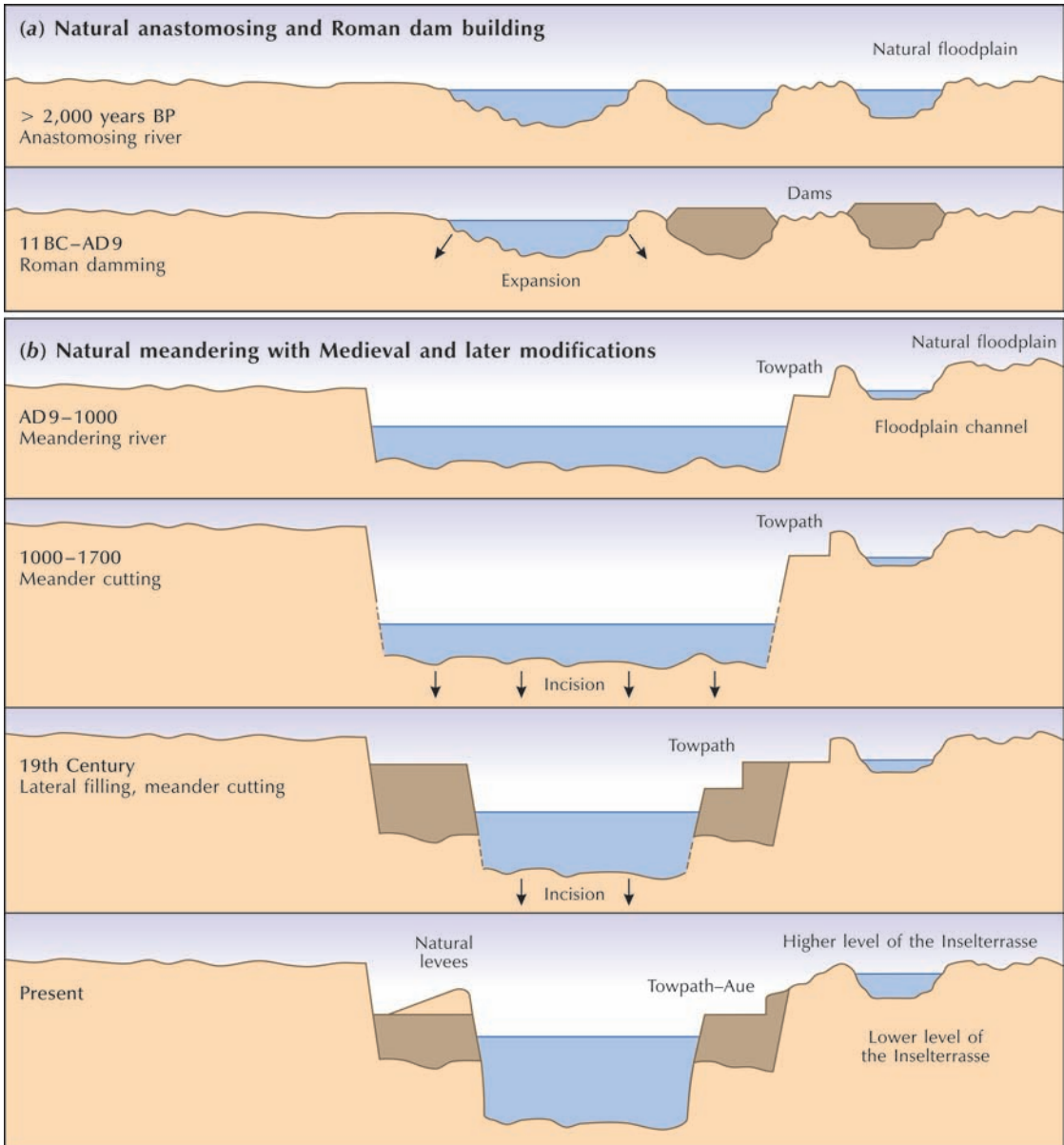
Figure 9.31 Evolution of Holocene terraces in the Lippe Valley. (a) Interpretation 1. (b) Interpretation 2. Source: Adapted from Herget (1998)
