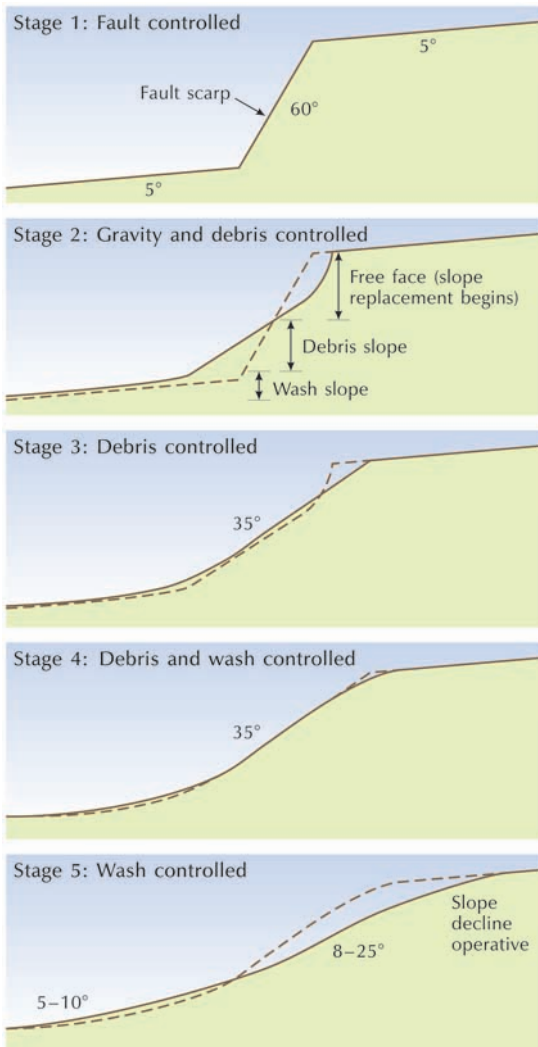
Figure 8.2 Proposed sequence of change on a fault scarp developed in alluvium, Nevada, USA. The changes are incremental, the dashed line shown at each stage representing the hillslope profile at the previous stage. Source: Adapted from Wallace (1977)
