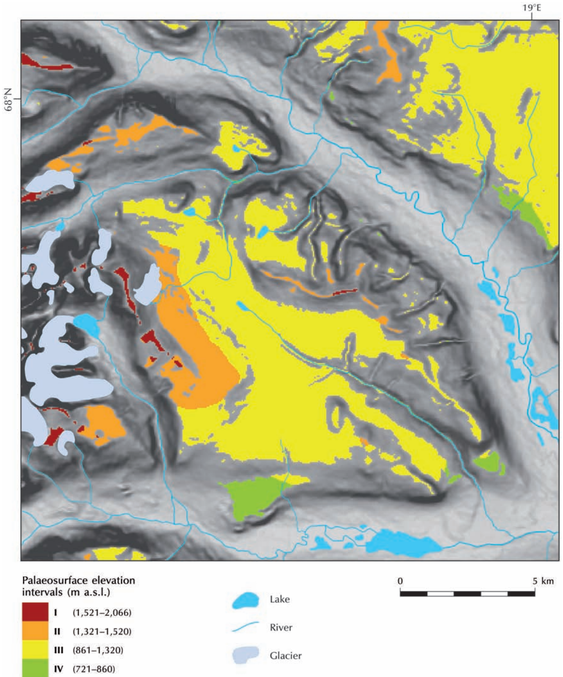
Figure 15.2 Surface and slope map of Tjeuralako Plateau, northern Sweden, and its surroundings with palaeosurface remnants and corresponding elevation classes shown in colour. Source: After Ebert (2009b)
