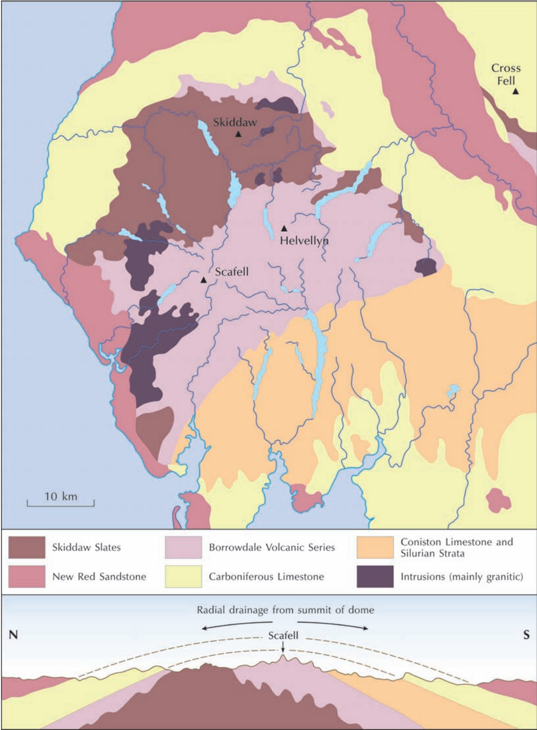
Figure 9.18 Superimposed drainage in the English Lake District. Source: Adapted from Holmes (1965, 564)
