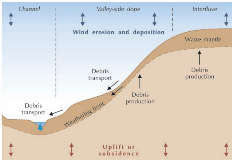
Figure 2.1 A hillslope as a system, showing storages (waste mantle), inputs (e.g. wind deposition and debris production), outputs (e.g. wind erosion), throughputs (debris transport), and units (channel, valley-side slope, interfluve).
