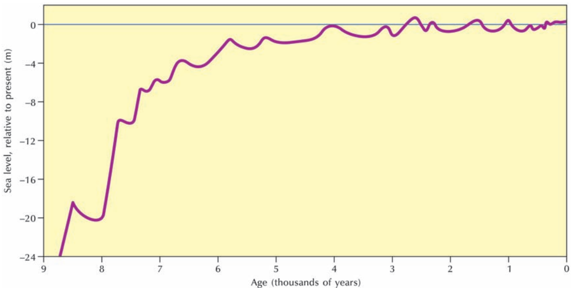
Figure 13.25 The Flandrian transgression in north-western Europe. Notice the rapid rise between about 9,000 and 7,000 years ago; this amounted to about 20 m, an average increase of 1 m per century. Source: Adapted from Mörner (1980)
