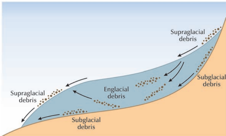
Figure 10.10 Transport by ice: supraglacial, englacial, and subglacial paths. Source: Adapted from Summerfield (1991, 271)
