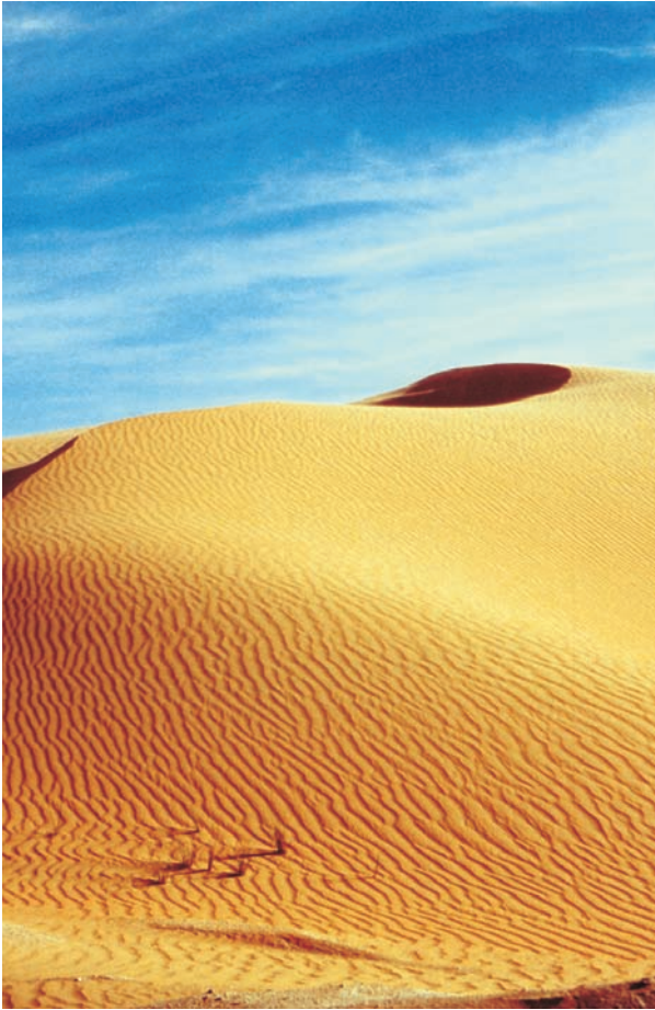
Plate 12.5 Rippled linear dune flank in the northern Namib Sand Sea, Namibia ( Photograph by Dave Thomas )
