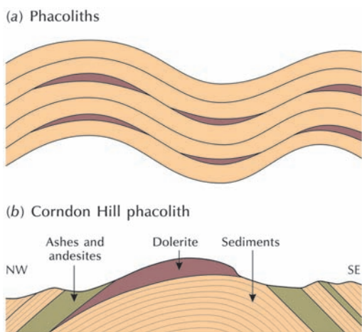
Figure 6.3 Phacoliths. (a) Occurrence in anticlinal crests and synclinal troughs. (b) Corndon Hill, near Montgomery in Wales, an eroded phacolith. Source: Adapted from Sparks (1971, 93, 94)
