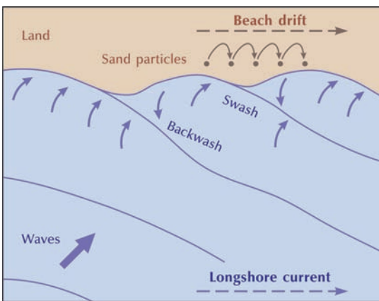
Figure 13.5 Beach drift. Source: Adapted from Butzer (1976, 226)
