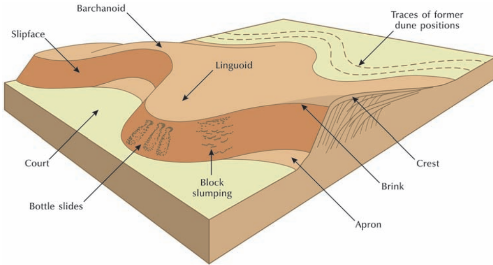
Figure 12.7 The main features of a dune. Source: Adapted from Livingstone and Warren (1996, 65)
