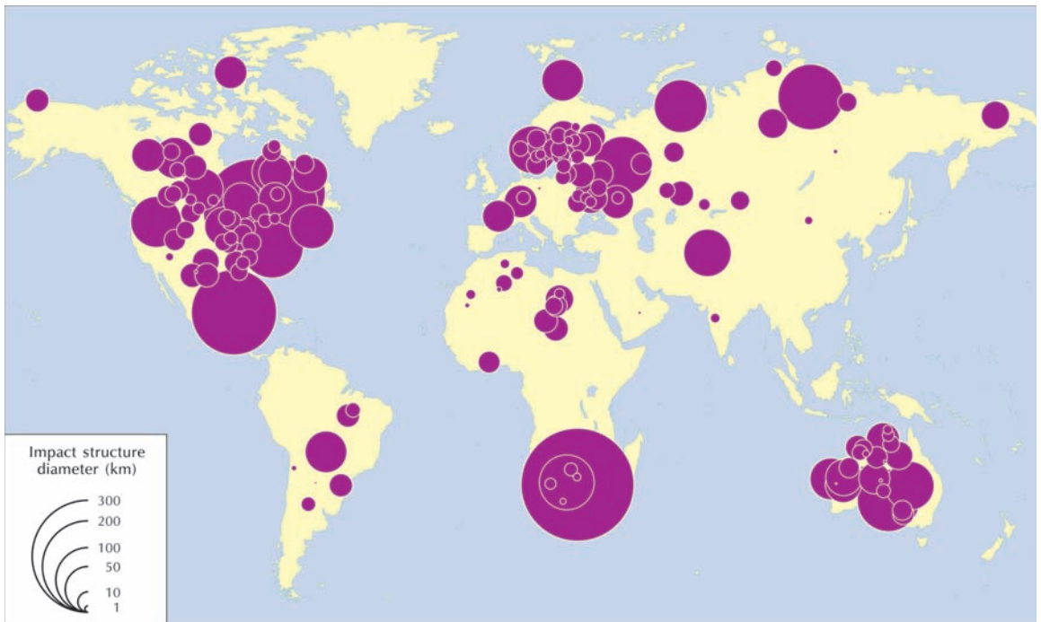
Figure 6.12 The distribution of known impact craters.
