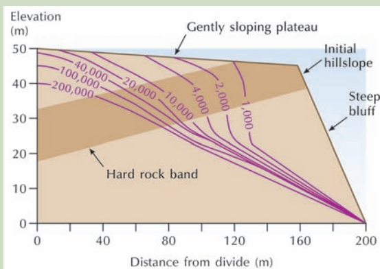
Figure 8.4 Simulation of hillslope change for an initial gently sloping plateau ending in a steep bluff with a band of hard rock dipping at 10° into the hillside. Time is in years. Source: Adapted from Kirkby (1985)
