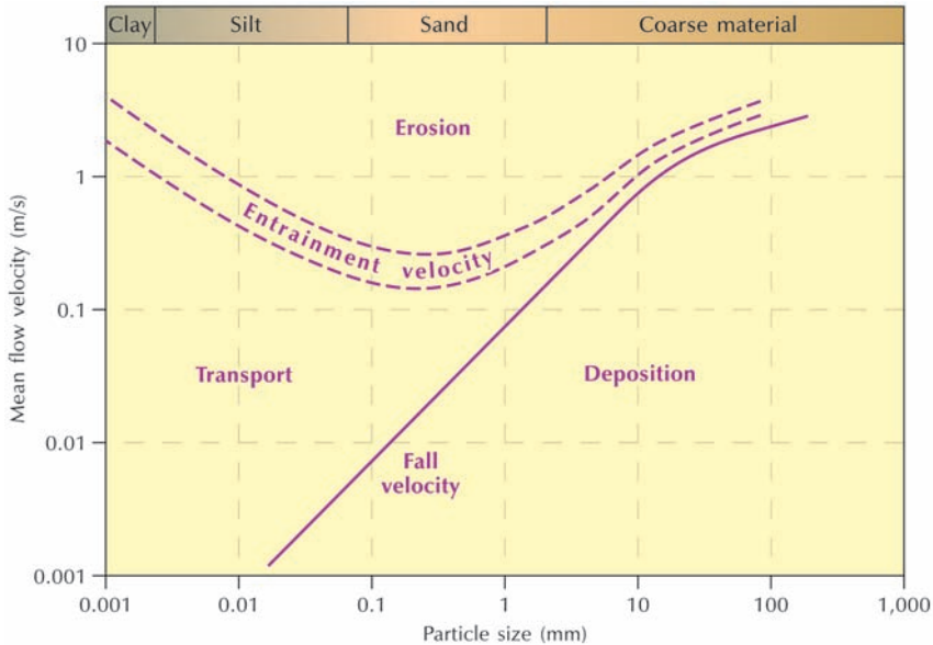
Figure 9.5 The Hjulstrøm diagram showing the water velocity at which entrainment and deposition occur for particles of a given size in well-sorted sediments. Source: Adapted from Hjulstrøm (1935)
