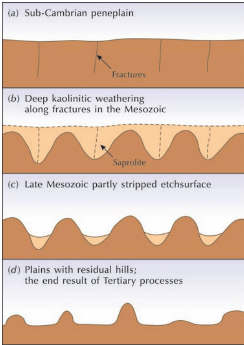
Figure 15.11 The three basic relief-types within the Fennoscandian Shield. (a) Sub-Cambrian peneplain. This exhumed and extremely flat palaeoplain, together with sub-Vendian and sub-Ordovician facets, is the starting point for all relief on the Fennoscandian shield. (b) Deep kaolinitic weathering along fractures in the Mesozoic. This is not a basic relief type, but led to (c) Late Mesozoic partly stripped etchplains, with a characteristic undulating hilly terrain and remnants of kaolinitic saprolite and Mesozoic cover rocks. (d) Late Tertiary plains with residual hills, which are the product of Tertiary surface denudation. Source: Adapted from Lidmar-Bergström (1999)
