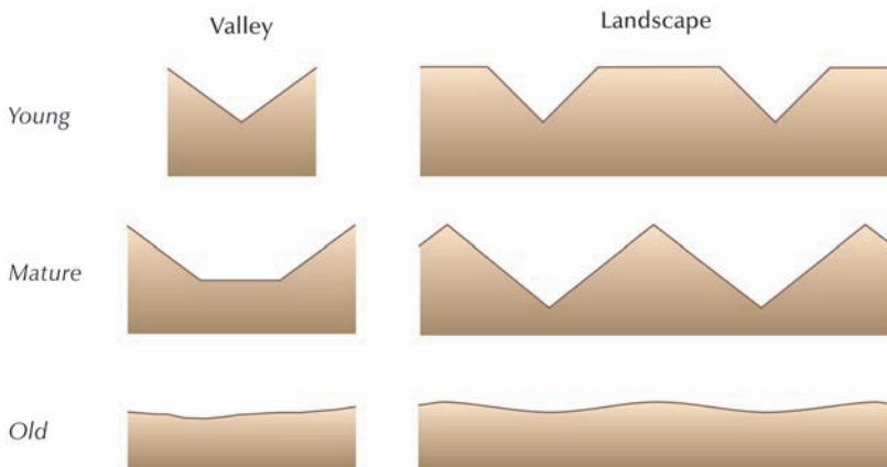
Figure 15.4 Traditional Davisian stage names for valley profiles and for landscape profiles. Source: Adapted from Ollier and Pain (1996, 204, 205)
