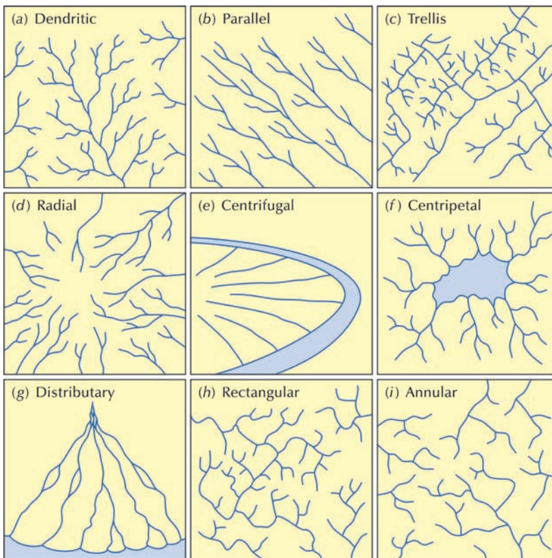
Figure 9.14 Drainage patterns controlled by structure or slope. Source: Mainly after Twidale and Campbell (2005, 191) and adapted from Twidale (2004, 173)
