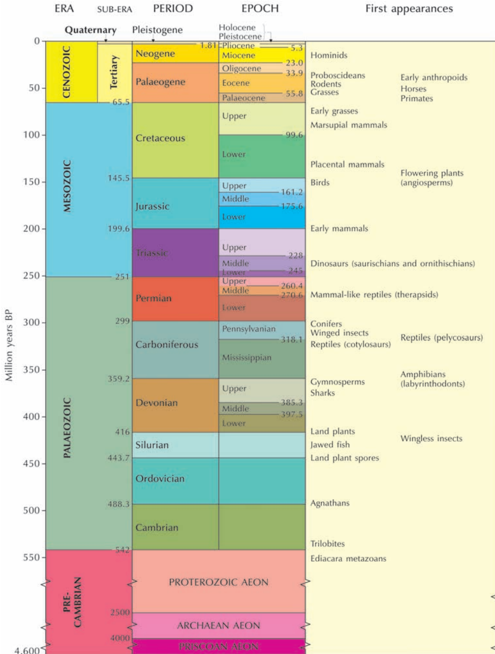
Figure A1 The geological timescale.
