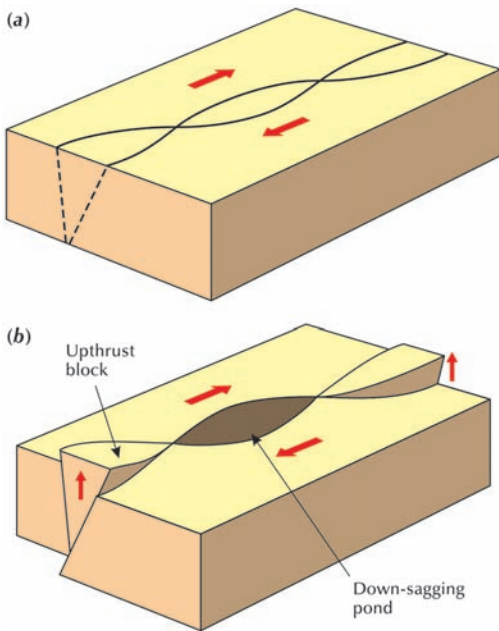
Figure 5.14 Landforms produced by anastomosing faults. (a) Anastomosing faults before movement. (b) Anastomosing faults after movement with upthrust blocks and down-sagging ponds. Source: Adapted from Kingma (1958)
