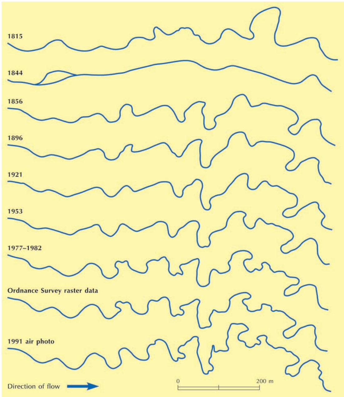
Figure 9.32 Channel change in Swinhope Burn, Upper Weardale, Yorkshire. The diagram shows the channel centre-line determined from maps, plans, and an air photograph. Source: After Warburton and Danks (1998)
