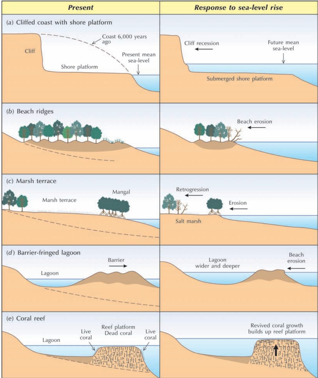
Figure 13.22 Coastal changes brought about by a rising sea level. (a) Cluffed coast with shore platform. (b) Beach ridges. (c) Marsh terrace. (d) Barrier-fringed lagoon. (e) Coral reef. Source: Adapted from Bird (2000, 278)
