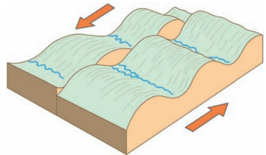
Figure 6.20 Shutter ridges along a strike-slip fault. Source: Adapted from Ollier (1981, 68)
