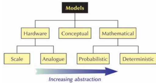
Figure 2.8 Types of model in geomorphology. Source: After Huggett (1993, 4)
