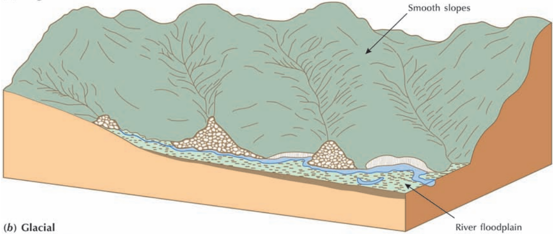
(b) Glacial
