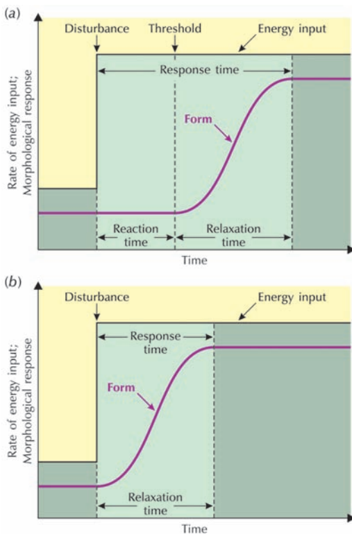
Figure 2.6 (a) Reaction time and (b) relaxation time in geomorphic systems.
