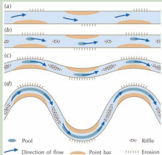
Figure 9.20 Pool-and-riffle sequences in river channels. (a) Alternating zones of channel erosion and accretion in response to faster and slower flow. (b) Pool spacing influencing the evolution of a straight channel into a meandering channel. (c) Additional pools form as the meandering channel lengthens. (d) Development of meandering channel with pools and riffles. Source: Adapted from Dury (1969)
