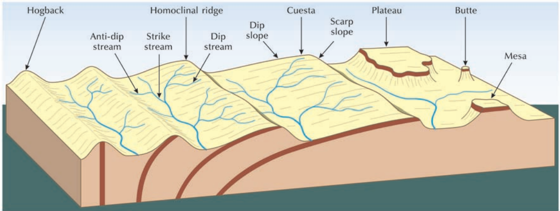
Figure 6.16 Landforms associated with dipping and horizontal strata – cuesta, homoclinal or strike ridge, hogback, butte, mesa, and plateau. The chief streams found in landscapes with dipping strata – strike streams, anti-dip streams, and dip streams – are shown. Notice that a cuesta consists of a dip slope and a steeper escarpment of scarp slope. The black band represents a hard rock formation that caps the butte, mesa, and plateau.
