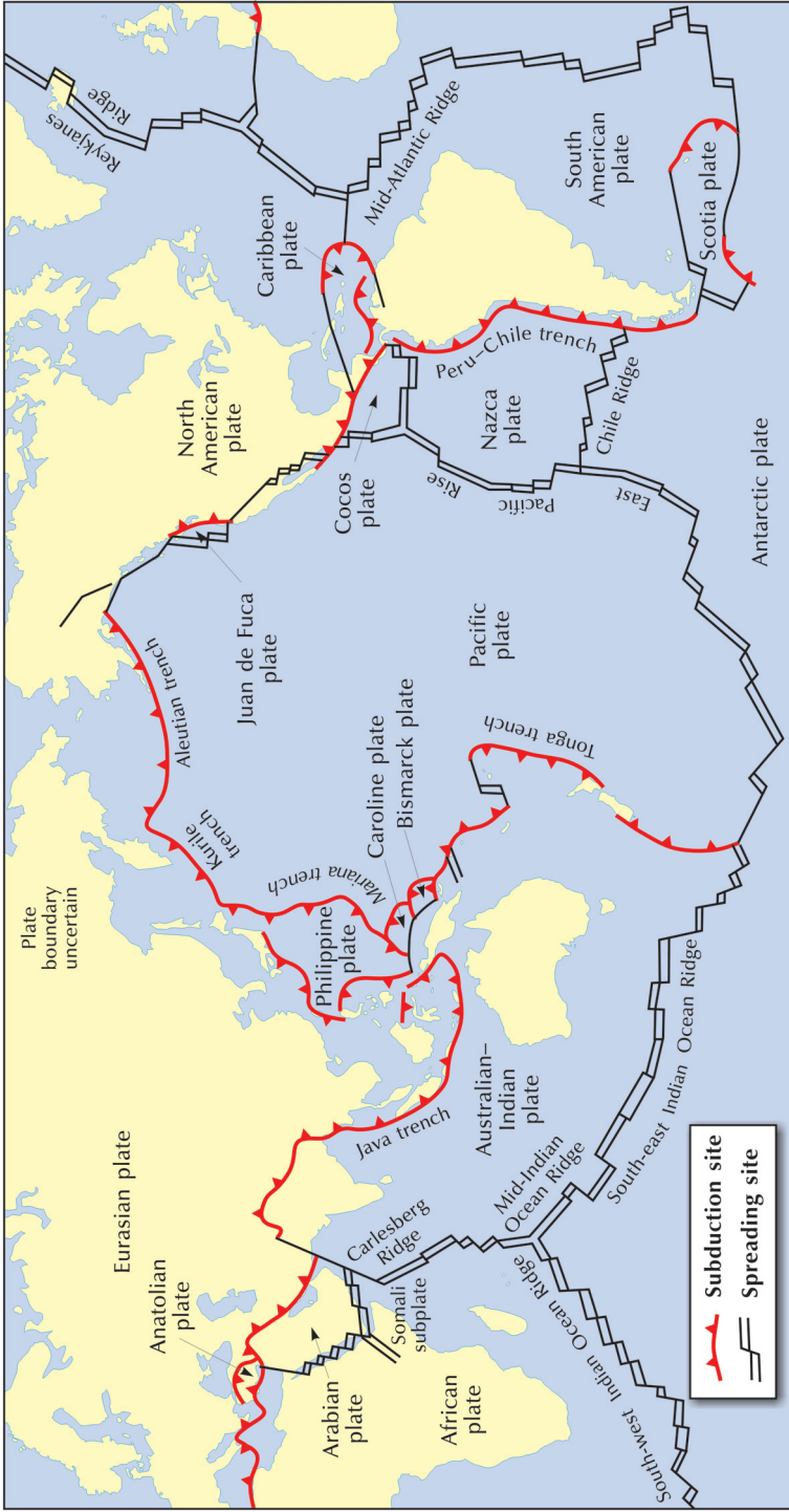
Figure 5.2 Tectonic plates, spreading sites, and subduction sites. Source: Adapted from Ollier (1996)
