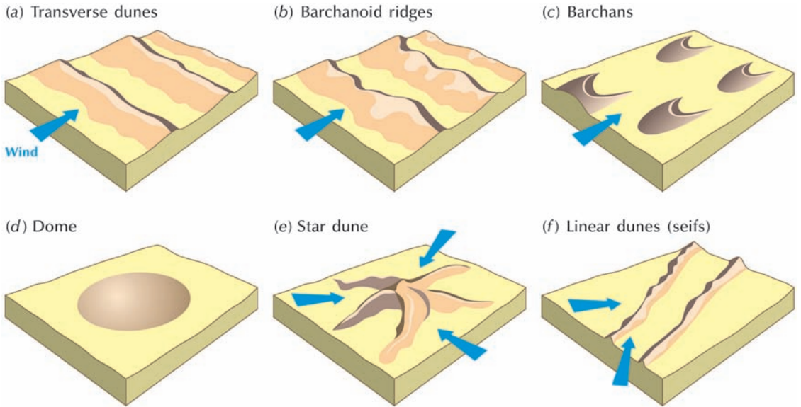
Figure 12.8 Types of free dunes. Source: Adapted from McKee (1979)
