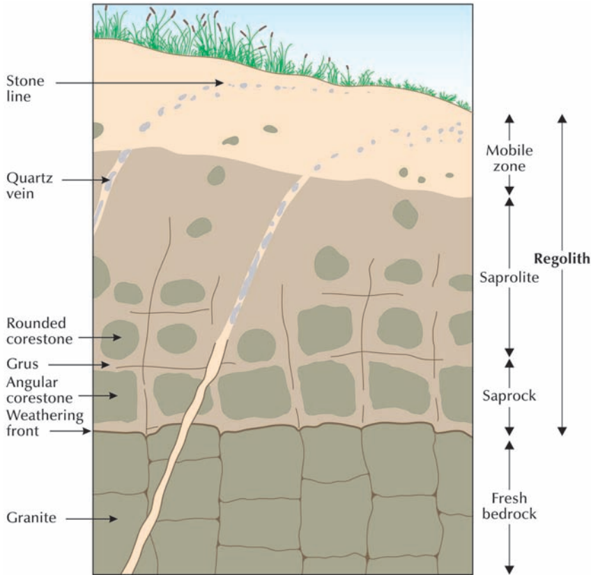
Figure 7.3 Typical weathering profile in granite. The weathering front separates fresh bedrock from the regolith. The regolith is divided into saprock, saprolite, and a mobile zone.
