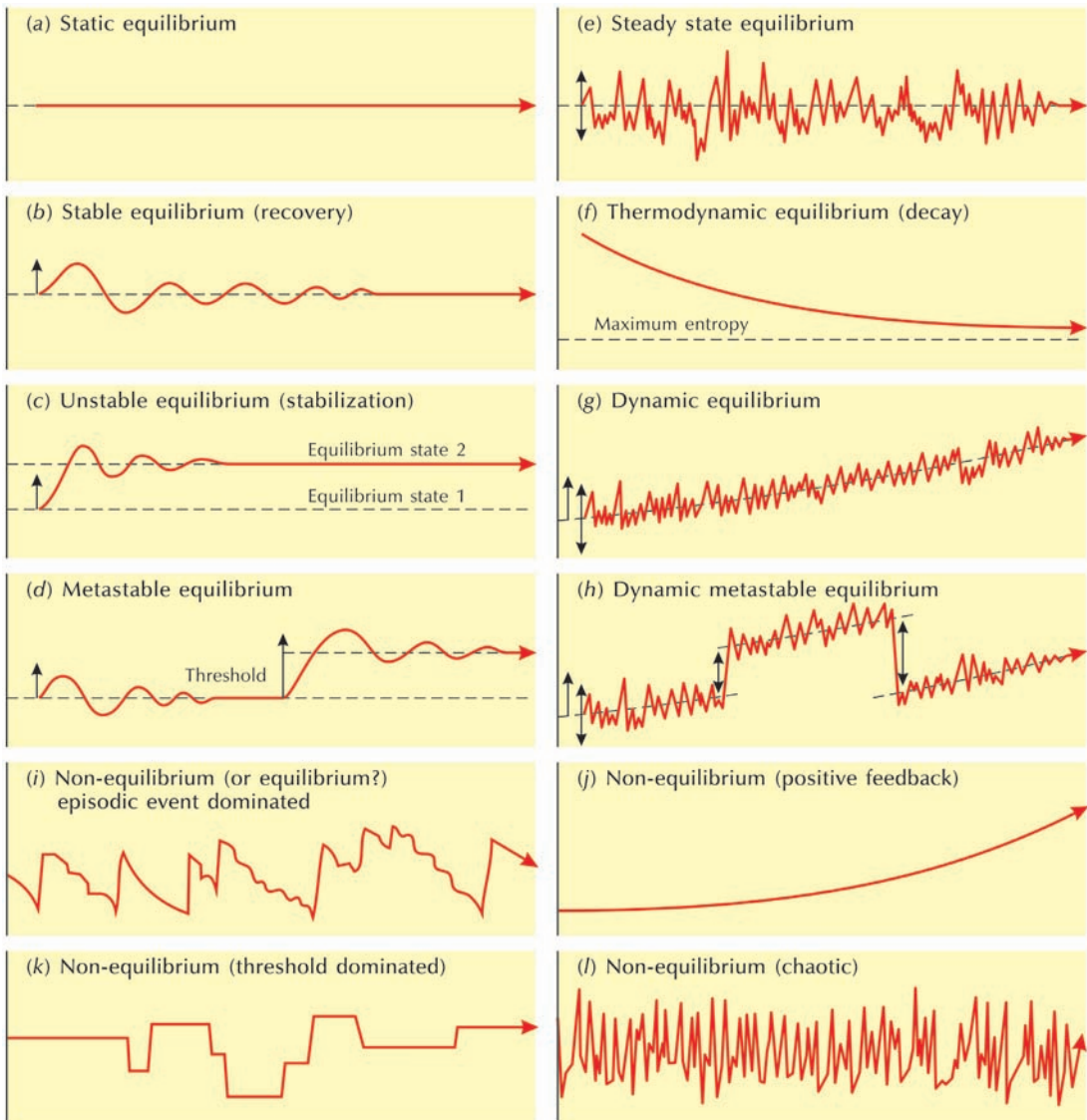
Figure 2.4 Types of equilibrium in geomorphology. Source: Adapted from Chorley and Kennedy (1971, 202) and Renwick (1992)
