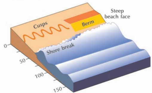
Figure 13.9 Beach types classified by wave and tide dominance. Source: Adapted from Short (2006, 2010) and Short and Woodroffe (2009)
