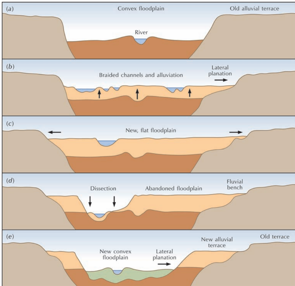
Figure 9.26 Alluvial terrace formation. (a) An initial convex floodplain. (b) Burial of the initial floodplain by coarser sediments through rapid alluviation of braided channels. (c) A stable, flat floodplain forms by alluviation and some lateral planation. (d) Another environmental change leads to dissection of alluvium and the abandonment of the flat floodplain. (e) A new convex floodplain is established by the alluviation of fine sediments and lateral planation. Source: Adapted from Butzer (1976, 170)
