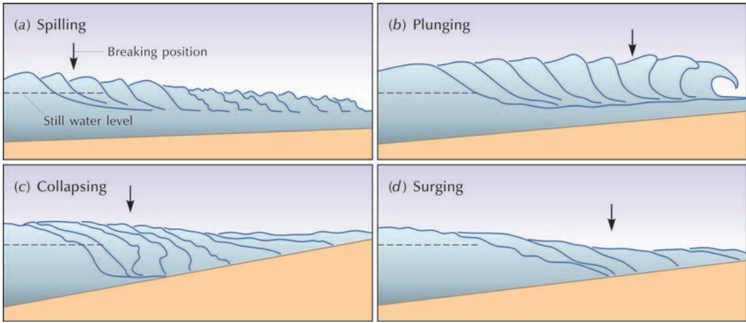
Figure 13.3 Kinds of breaking waves derived from high-speed moving pictures. Source: Adapted from Komar (1998, 210)
