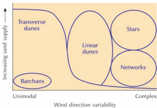
Figure 12.6 Dune types in relation to the variability of wind direction and sand supply. Source: Adapted from Livingstone and Warren (1996, 80)
