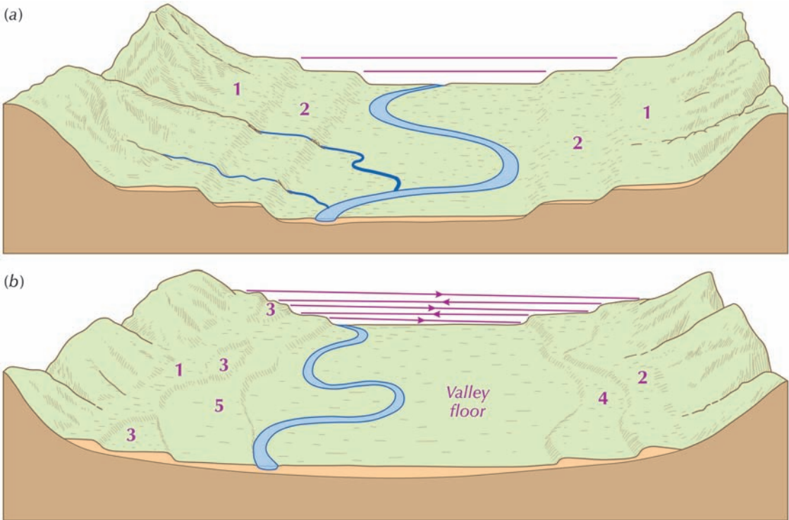
Figure 9.23 Paired and unpaired terraces. (a) Paired, polycyclic terraces. (b) Unpaired, noncyclic terraces. The terraces are numbered 1, 2, 3, and so on. Sources: Adapted from Sparks (1960, 221–23) and Thornbury (1954, 158)
