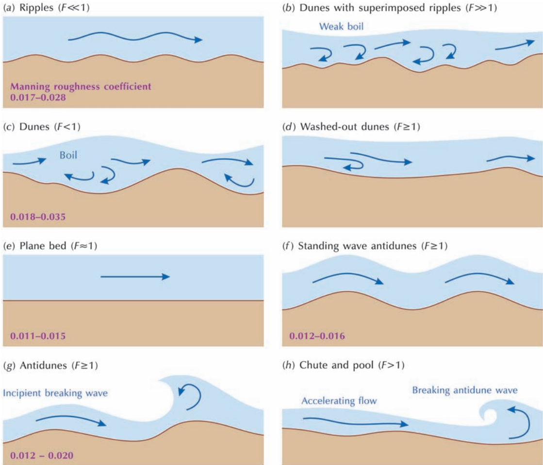
Figure 9.21 Bedforms in a sandy alluvial channel change as the Froude number, F , changes. At low flow velocities, ripples form that change into dunes as velocity increases. A further increase of velocity planes off bed undulations, and eventually a plane bed forms. The plane bed reduces resistance to flow, and sediment rates increase. The channel then stands poised at the threshold of subcritical and supercritical flow. A further increase of velocity initiates supercritical flow, and standing antidunes form. Flow resistance is low at this stage because the antidunes are in phase with the standing waves. The antidunes move upstream because they lose sediment from their downstream sides faster than they gain it through deposition. At the highest velocities, fast-flowing and shallow chutes alternate with deeper pools. Source: Adapted from Simons and Richardson (1963) and Simons (1969)
