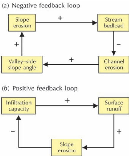
Figure 2.3 Feedback relationships in geomorphic systems. (a) Negative feedback in a valley-side slope–stream system. (b) Positive feedback in an eroding hillslope system. Details of the relationships are given in the text.
