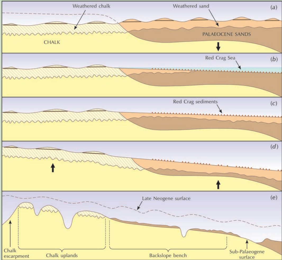
Figure 15.9 Cartoon depiction of a possible evolutionary model for the prominent backslope bench of the London Basin involving modified etchplanation. (a) Neogene duricrusted surface of low relief. (b) Red Crag incursion (see Figure 9.28) following downwarping to the east. (c) After marine regression. (d) Accentuated weathering beneath former marine platform leads to the development of an etch surface. (e) Differential uplift in the Pleistocene leads to dissection and the removal of much regolith with the remainder greatly disturbed and mixed by periglaciation. Source: After Jones (1999). Reproduced by permission of the Geological Society, London, and David Jones
