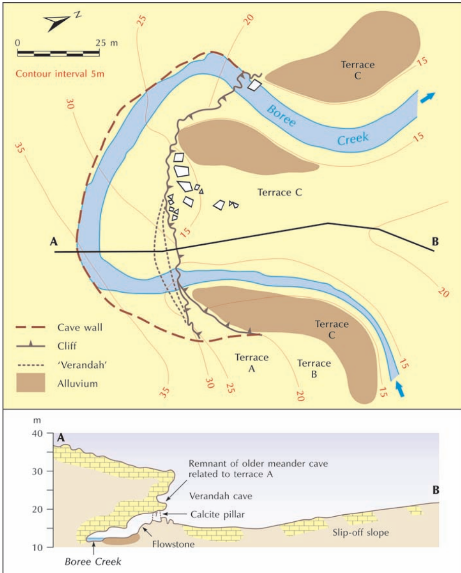
Figure 14.14 A meander cave on Boree Creek, Borenore, New South Wales, Australia. Source: Adapted from Jennings (1971, 101)
