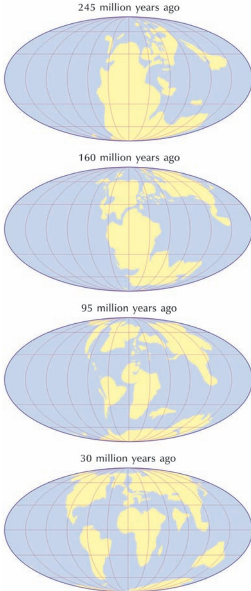
Figure 5.4 Changing arrangement of continents over the last 245 million years, showing the breakup of Pangaea, during the Early Triassic period; during the Callovian age (Middle Jurassic); during the Cenomanian age (Late Cretaceous); and during the Oligocene epoch. All maps use Mollweide's equal-area projection. Source: Adapted from maps in Smith et al. (1994)
