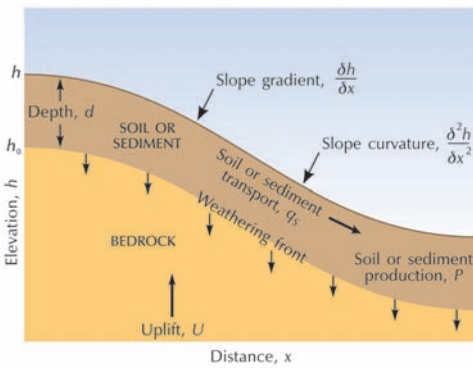
Figure 8.5 Components of numerical landscape models.
