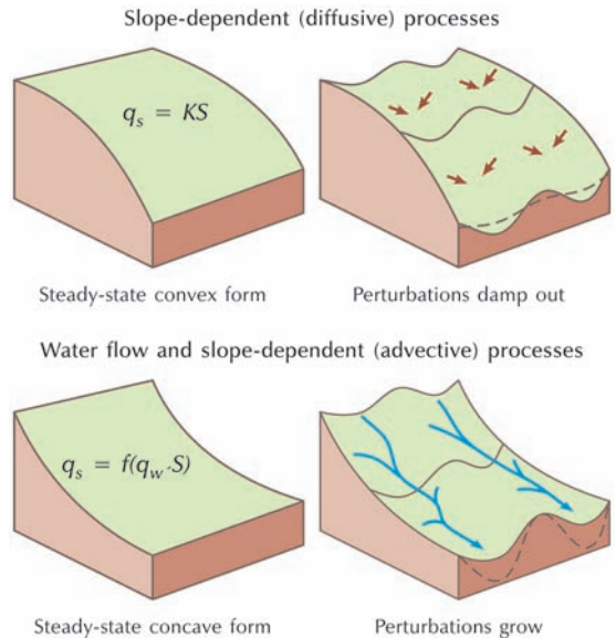
Figure 8.6 An explanation for the development of ridge-and-valley topography in soil-mantled terrain. Slope-dependent (diffusive) transport leads to convex hillslopes, and when the topography is laterally perturbed the transport direction (black lines) causes the topographic highs to lower and topographic lows to fill in, resulting in smooth topography, as suggested by the dashed line. In contrast, advective transport, which depends on water flow and slope gradient, carries sediment downslope and produces concave hillslopes. Flow concentrations (black flowpaths) resulting from lateral topographic perturbation lead to incision, as suggested by the dashed lines. The competition of these two processes leads to diffusion-dominated ridges and advection-dominated valleys. Source: Adapted from Dietrich and Perron (2006)
