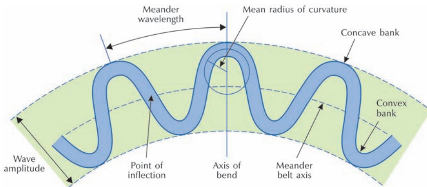
Figure 9.10 Parameters for describing meanders.
