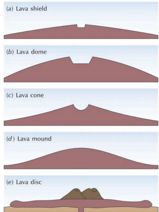
Figure 6.6 Types of basic-lava volcanoes, not drawn to scale. Source: Adapted from Ollier (1969, 21)
