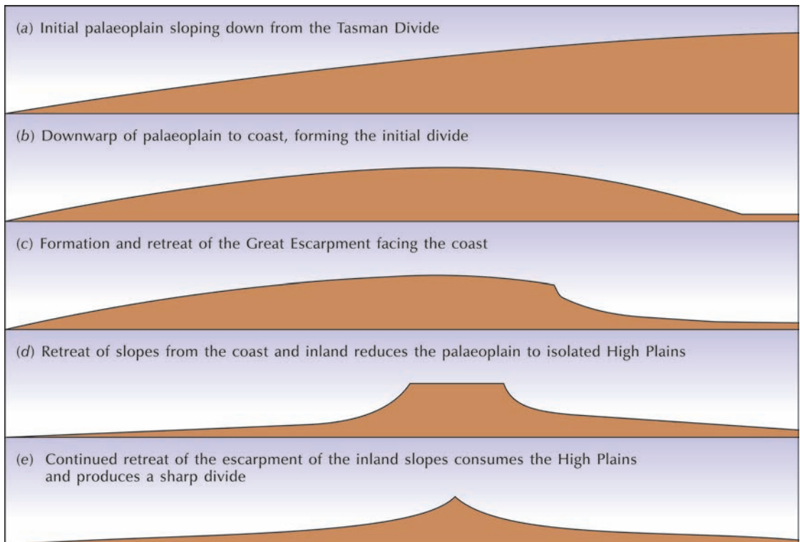
Figure 15.17 Evolution of the south-east Australian drainage divides. Source: Adapted from Ollier (1995)
