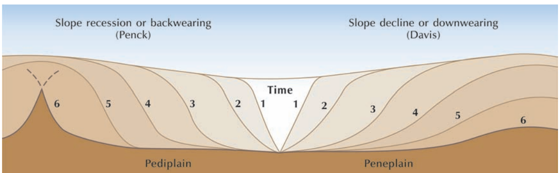
Figure 15.1 Slope recession, which produces a pediplain (p. 439) and slope decline, which produces a peneplain. Source: Adapted from Gossman (1970)
