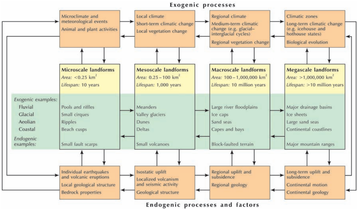
Figure 1.1 Landforms at different scales and their interactions with exogenic (external) and endogenic (internal) processes.
