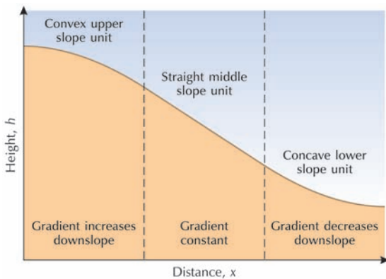
Figure 8.7 Three form elements of slopes.
