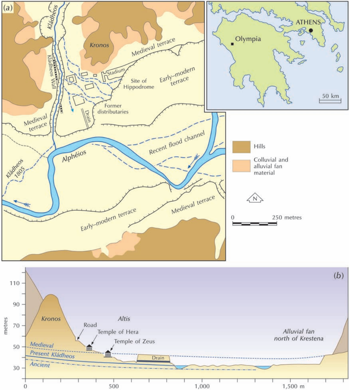
Figure 9.29 Olympia. (a) The archaeological site (Altis) with the Kládheos stream running alongside it to enter the Alphéios from the north. (b) North–south cross-section of Kronos Hill and the Alphéios terraces and valley floor. Source: Adapted from Büdel (1963)
