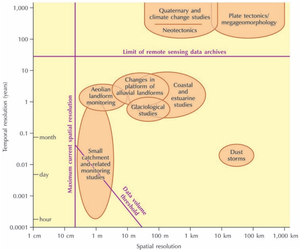
Figure 2.11 Constraints of spatial and temporal resolutions of satellite sensors on geomorphic studies. Source: Adapted from Millington and Townshend (1987) and Smith and Pain (2009)
