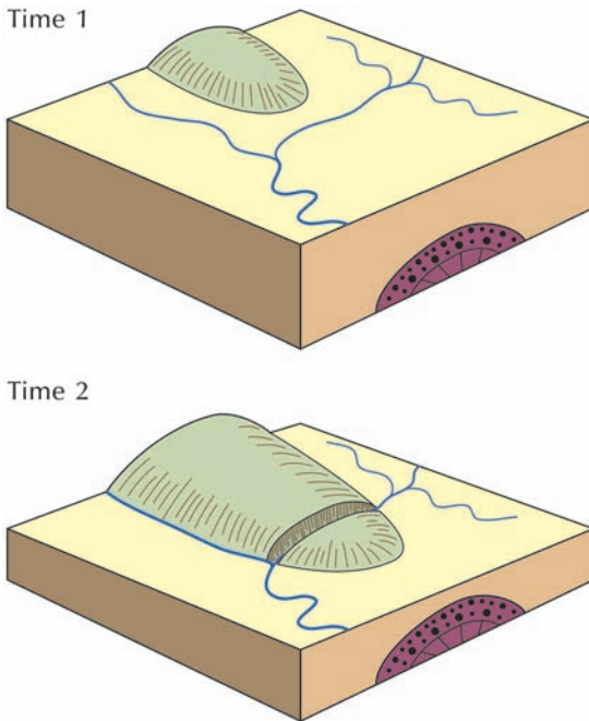
Figure 9.19 Gorge development in a snout of a resistant rock formation by stream persistence across a plunging anticline. Source: After Twidale and Campbell (2005, 195)
