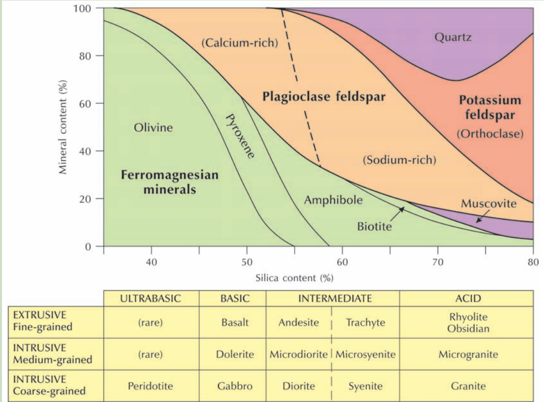
Figure 4.1 Igneous rocks and their component minerals. The classification is based on the silica content, which produces an ultrabasic–acid axis. The terms ‘acid’ and ‘basic’ are not meant to suggest that the rocks are acidic or alkaline in the customary sense, but merely describe their silica content.
