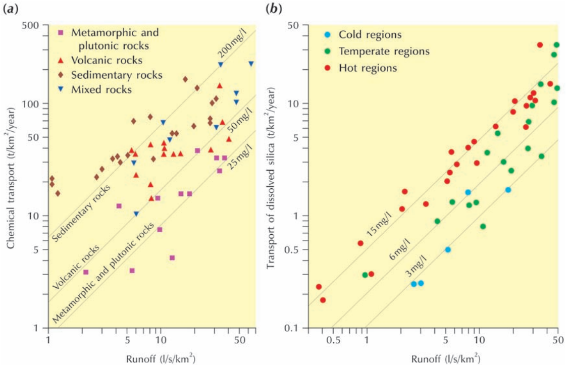
Figure 4.8 Dissolved loads in relation to runoff. (a) Chemical transport of all major ions plus dissolved silica versus runoff (specific discharge) for various major drainage basins underlain by sedimentary, volcanic, and metamorphic and plutonic rocks. (b) Evolution of the specific transport of dissolved silica for cold, temperate, and hot regions. Source: Adapted from Meybeck (1987)
