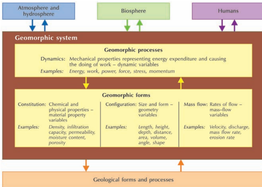
Figure 1.2 Process–form interactions – the core of geomorphology.
