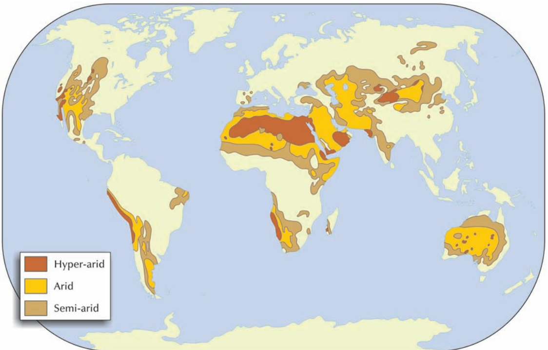
Figure 12.1 The world's deserts. Source: Adapted from Thomas (1989)
