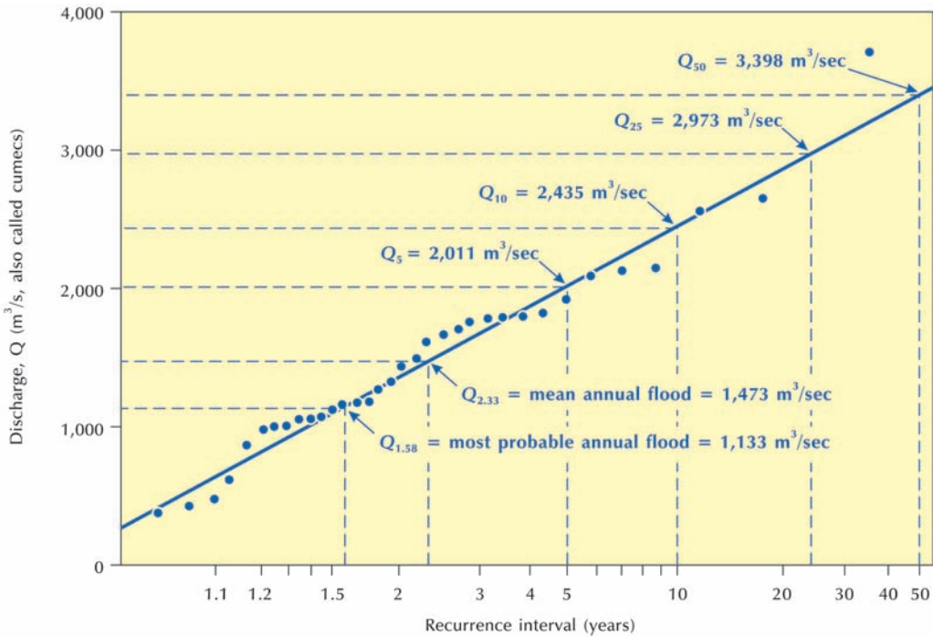
Figure 2.7 Magnitude–frequency plot of annual floods on the Wabash River, at Lafayette, Indiana, USA. See text for details. Source: Adapted from Dury (1969)
