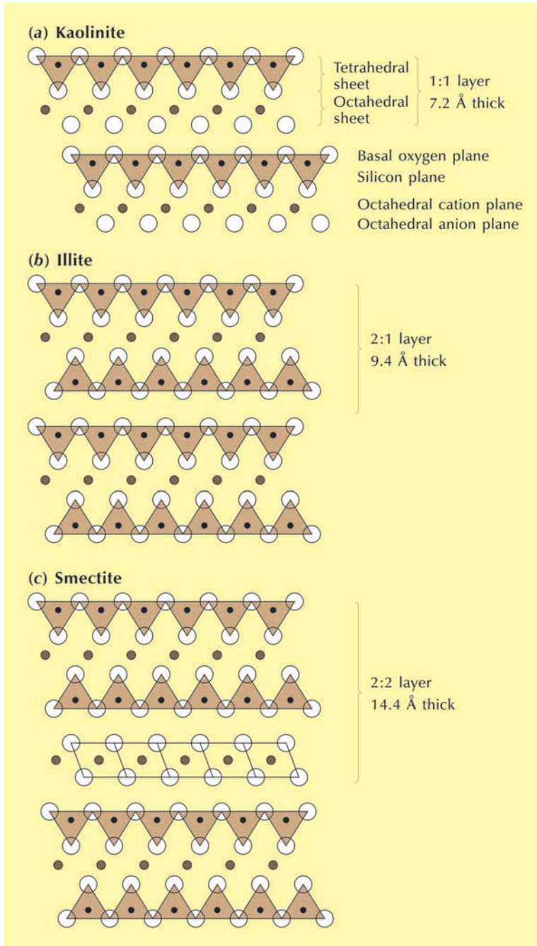
Figure 7.1 Clay mineral structure. (a) Kaolinite, a 1 : 1 dioctahedral layer silicate. (b) Illite, a 2 : 1 layer silicate, consisting of one octahedral sheet with two flanking tetrahedral sheets. (c) Smectite, a 2 : 2 layer silicate, consisting of 2 : 1 layers with octahedral sheets between. Å stands for an angstrom, a unit of length (1Å = 10 -8 cm). Source: After Taylor and Eggleton (2001, 59, 61)
