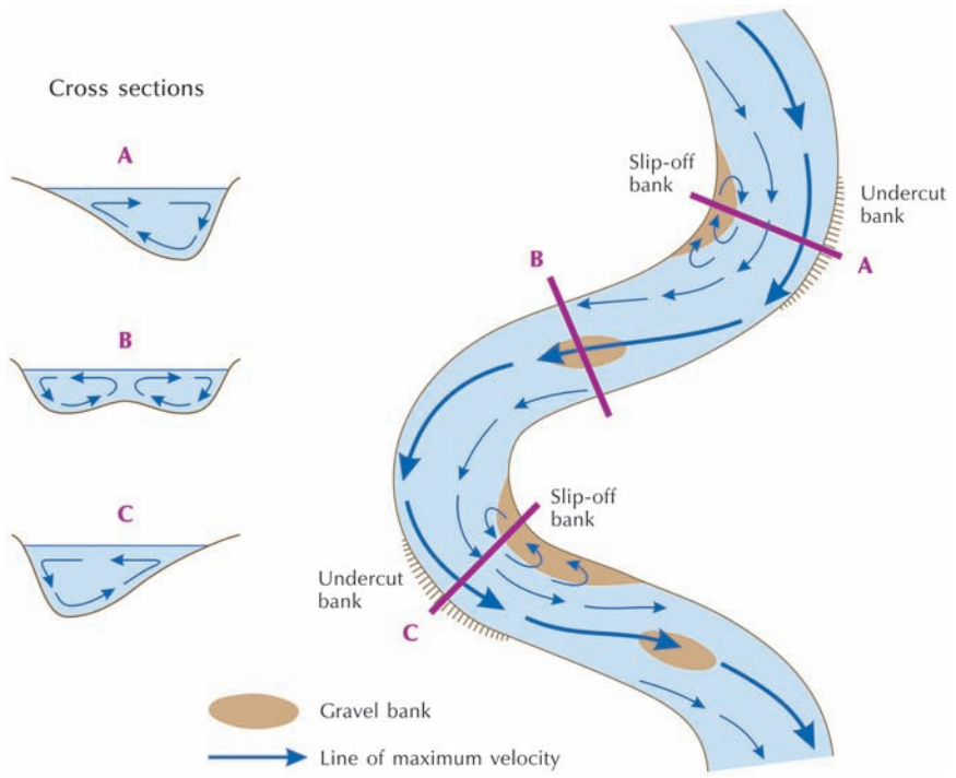
Figure 9.9 Water flow in a meandering channel.
