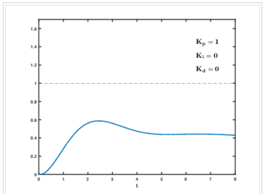
Effects of varying PID parameters ( K_p, K_i, K_d ) on the step response of a system.
