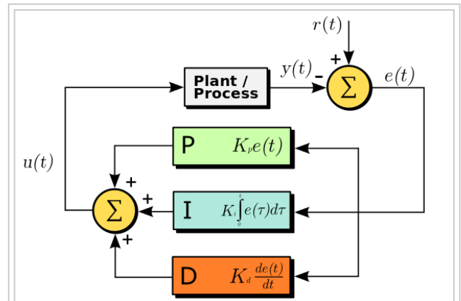
A block diagram of a PID controller in a feedback loop
