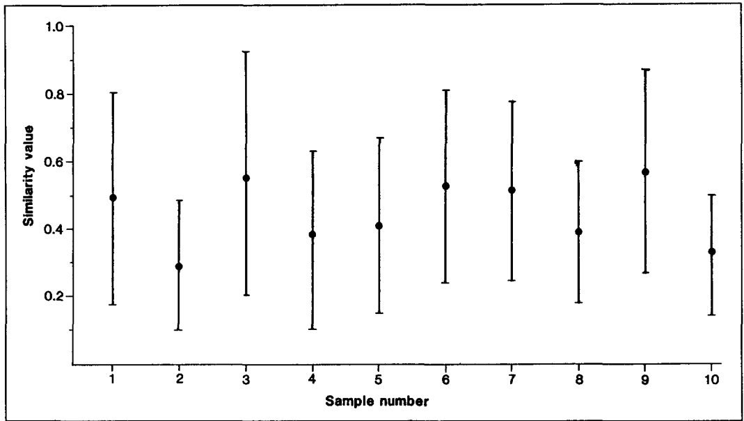
Figure 1—Mean values of Spatz' modification of Jaccard's index of similarity ( IS_{sp} ), for random subsamples of fecal samples used in developing the technique.
