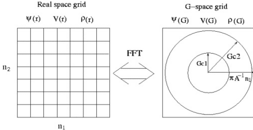
Fig.1, the due space representation of the PW method. The reciprocal space (right box) and real space (left box). The wavefunction q vectors ( G=q in this figure) inside the cutoff G_{c1} are chosen in the summation of Eq.(6), while the potential V and charge density \rho are represented by the planewave q inside a larger cutoff G_{c2} . G_{c1} is half of G_{c2} . FFT is used to transform the wavefunction from reciprocal space representation to a real space grid.
