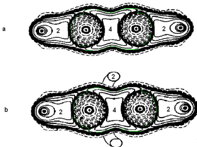
Figure 4: Contour map of the Ethyne molecule and its electron count. There is a lack of two electrons (a). This electrons are fused in a toroidal lone pair around the C-C bond (b). The green line shows how the C-C bond was cut. This is a modified figure taken from [7].
