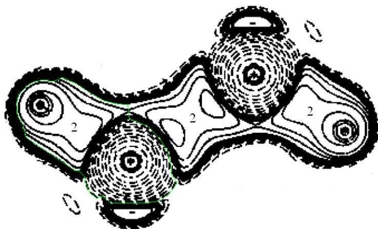
Figure 3: Contour map of the Ethane molecule and its electron count. The green line shows how the C-H bond was cut. The C-C bond was also cut accordingly. This is a modified figure taken from [7].
