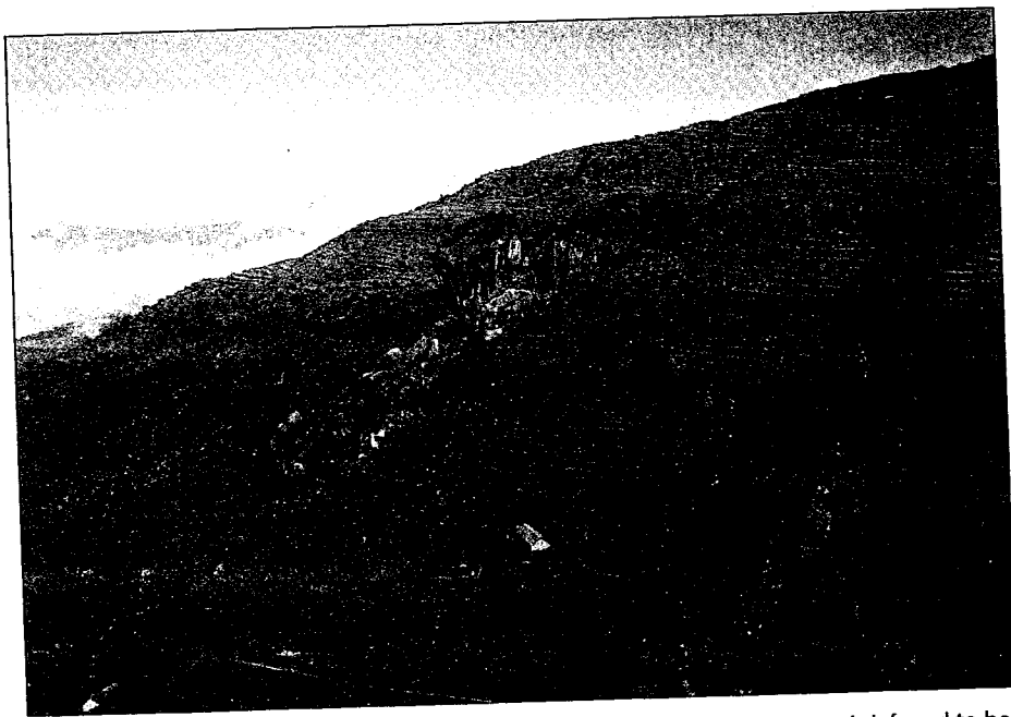
Figure 1. A slope in Nepal, terraced for agriculture. The rock tower in the center is inferred to be a volcanic neck. Its height above the rest of the slope (see house for scale) represents differential erosion over a time period that must be long compared with that represented by the terracing.
