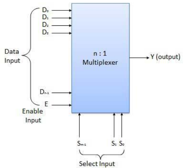
Fig.3 Multiplexer
