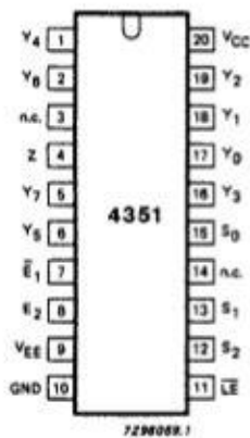
Fig.6 IC 74HCT4351 Pin Diagram
