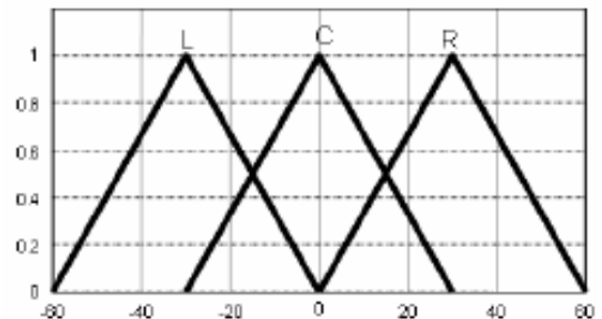
Fig-5: Fuzzy Set Definition for the Output Variable \theta
