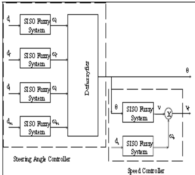
Fig-1: Structure of the Proposed Controller
