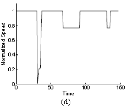
Fig-16 : a): Robot Trajectory; b) Variation of weighting factors; c) Variation of steering angle; d) Variation of speed with time for case 8.
