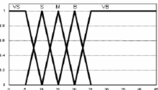
Fig-6: Fuzzy Set Definition for the Second Stage Input Variable |\theta|
