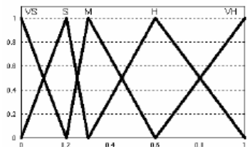
Fig-7: Fuzzy Sets Definition for the Second Stage Output Variable v
