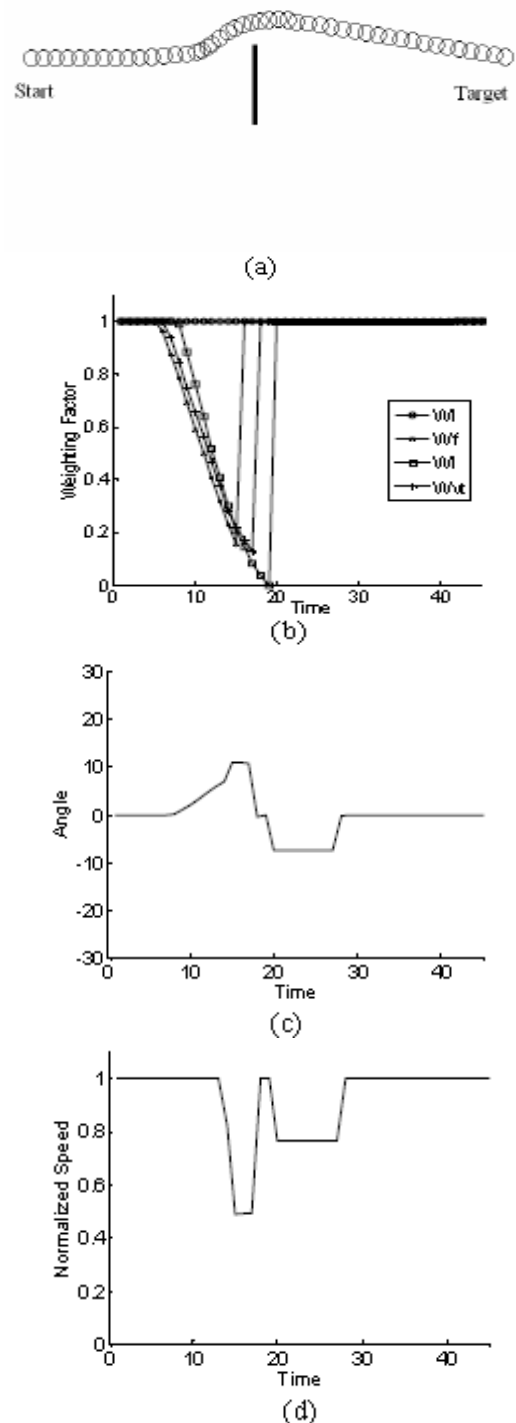
Fig-11: a): Robot Trajectory; b) Variation of weighting factors; c) Variation of steering angle; d) Variation of speed with time for case 3.
