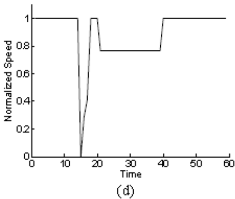
Fig-15 : a): Robot Trajectory; b) Variation of weighting factors; c) Variation of steering angle; d) Variation of speed with time for case 7.
