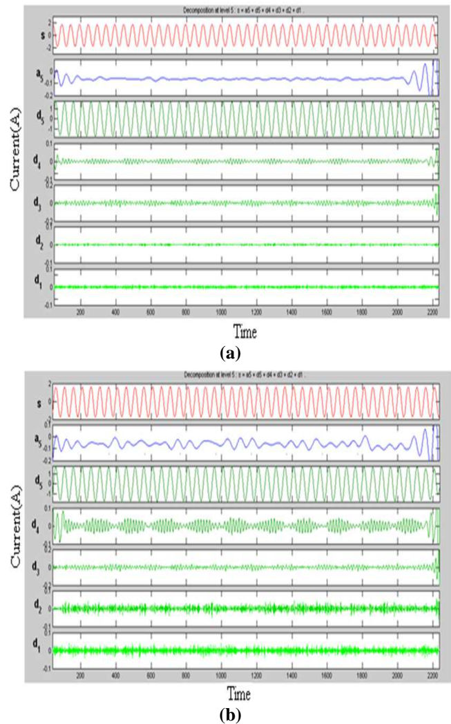
Figure 5. Decomposition of stator current in matlab
