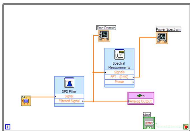
Figure 2. Block diagram of the created virtual instrument panel analogical
