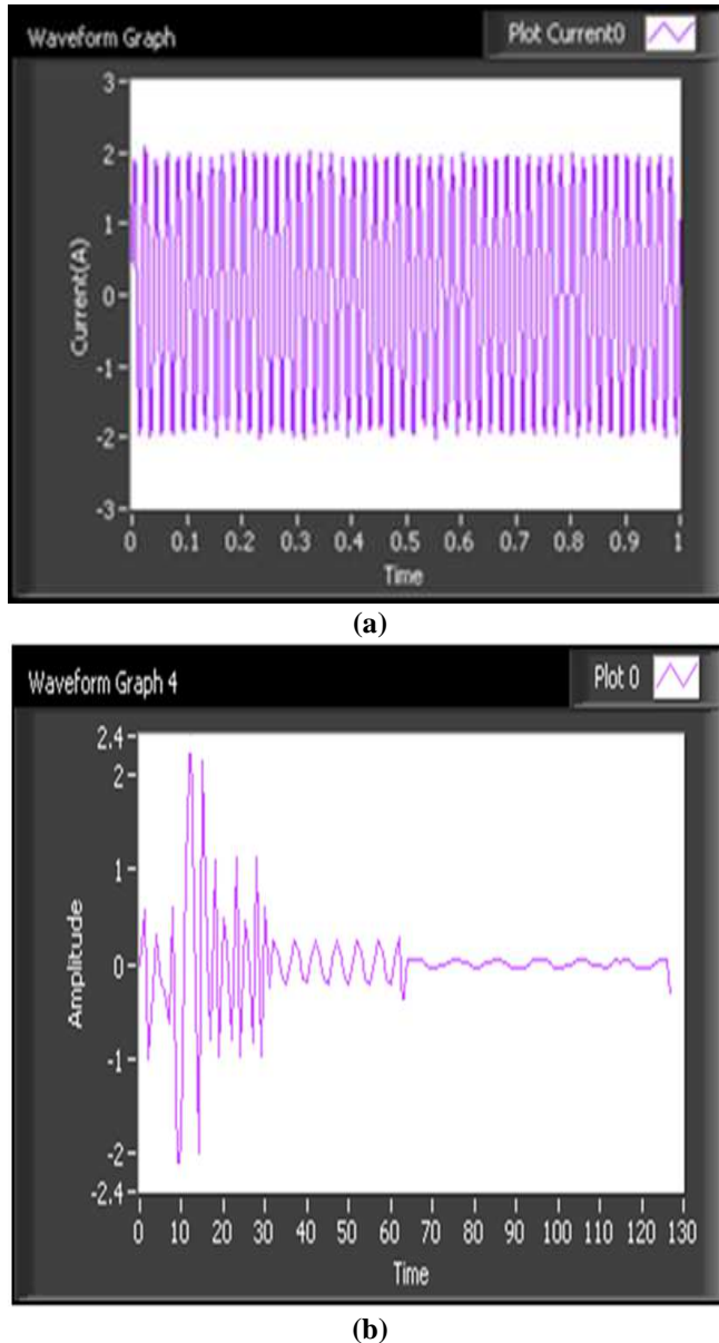
Figure 4. Stator current waveform and wavelet transform in faulty state
