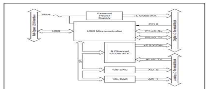
Figure 1. NI data acquisition device
