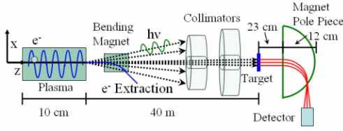
Figure 1: Experimental schematic. Not drawn to scale.
