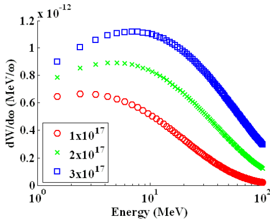
Figure 3: Calculated dW/d\omega for the collimated 8mm photon beam from a 28.5 GeV Gaussian beam at three different densities ( \text{cm}^{-3} ). All cases assume L_p = 10\text{cm} , \sigma_r = 10\mu\text{m} , and n_e = 9.6 \times 10^9 where n_e is 60 percent of the incident electrons.
