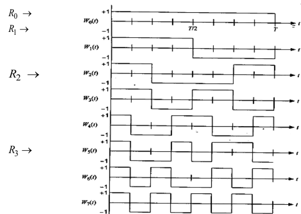
Figure 1. Walsh functions of order 8 = 2^3
