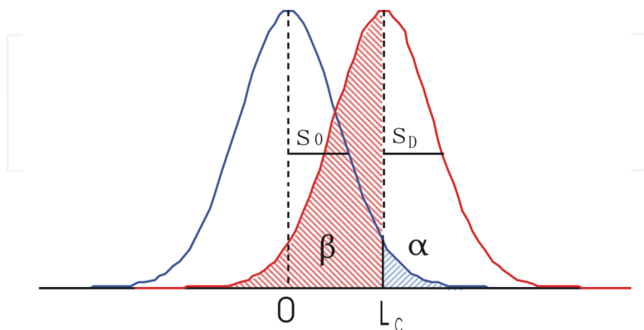
Figure 2. Critical level and limit of detection with probability \alpha . The risk of a false negative is 50%.
