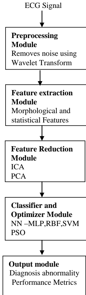
Fig.2 Flow Diagram of ECG Beat Classification
