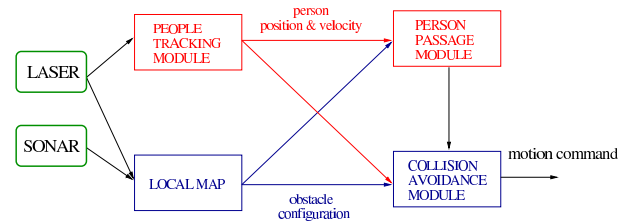
Fig. 4. The overall control system architecture.
