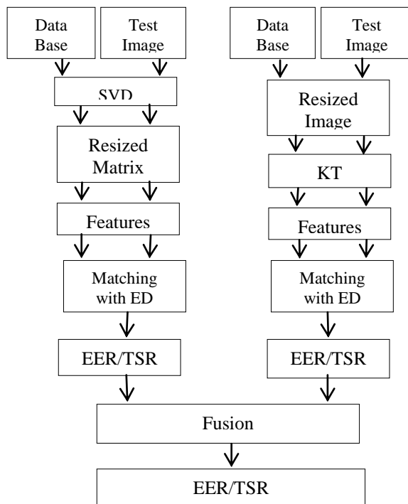
Figure 1: Block diagram of FRLSK model
