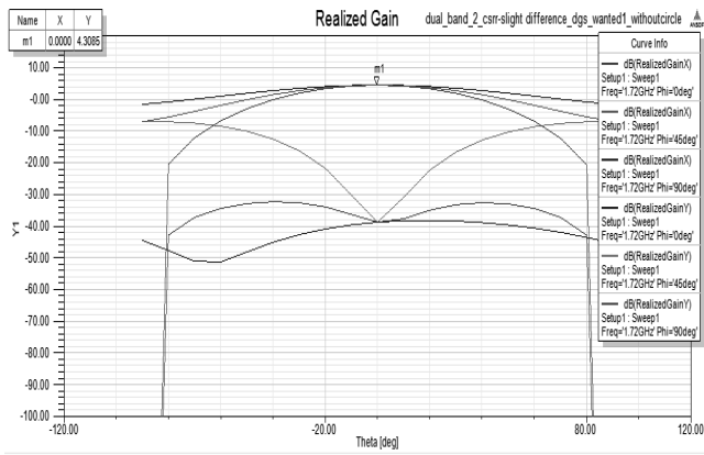
Figure 5 Realized Gain at 1.72 GHz
