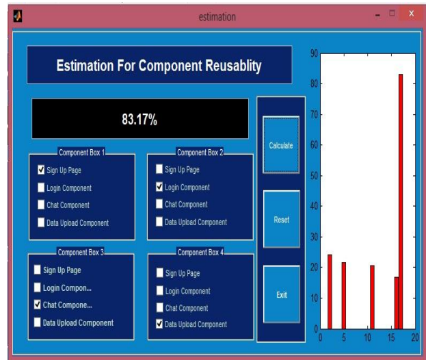
Fig 1: Automation Tool
