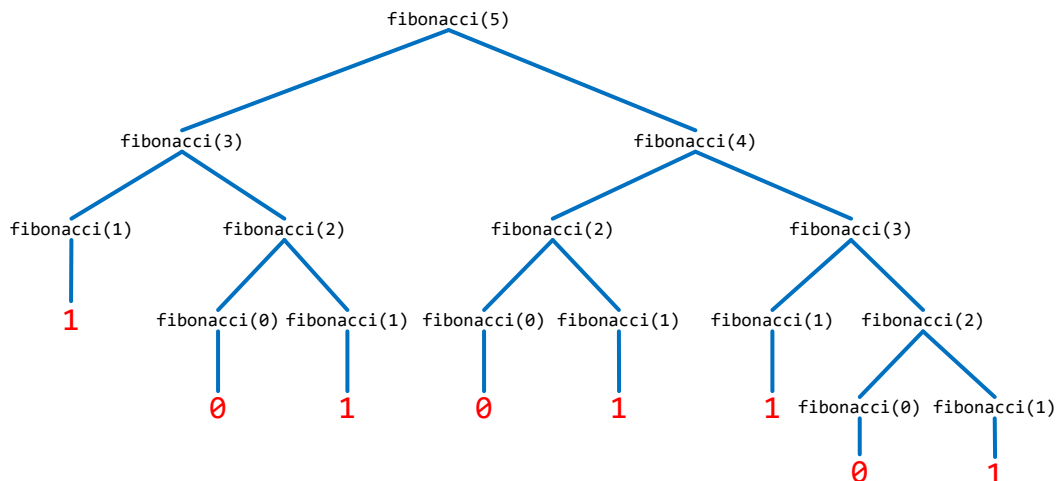
Figure 15.10 The hierarchy of recursive function calls that result from the call fibonacci(5) . Note that the recursion process calls fibonacci(1) five times.
