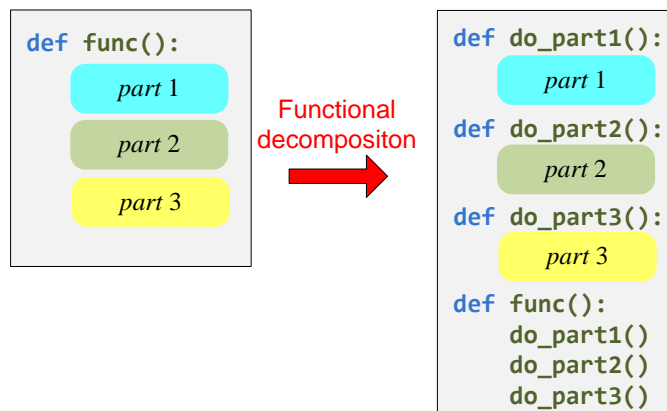
Figure 8.6 Decomposing a larger function into a collection of smaller functions. Callers now have access to the individual functions do_part1 , do_part2 , and do_part3 , as well as to func .
