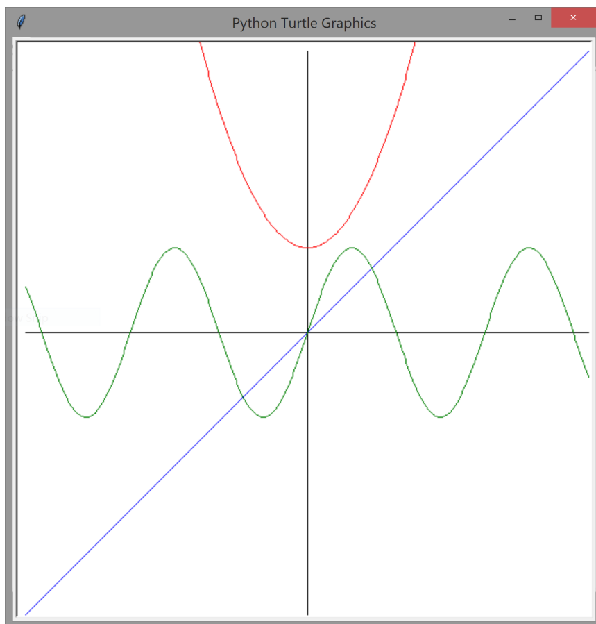
Figure 8.5 A screenshot of the plot function rendering the mathematical functions f(x) = \frac{1}{2}x^2 + 3 (red), f(x) = x (blue), and f(x) = 3\sin x , all over the range -10 \leq x < 10 .
