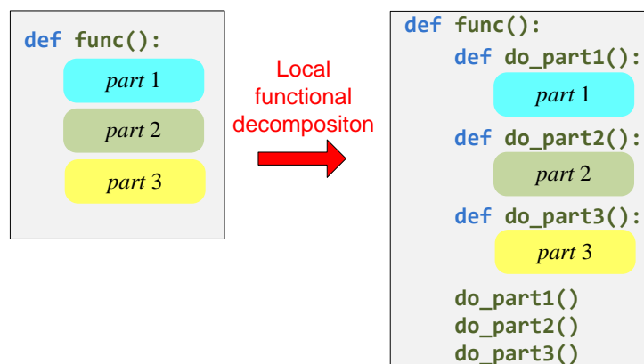
Figure 8.7 The local functions do_part1 , do_part2 , and do_part3 are available to function func but are inaccessible outside the func function
