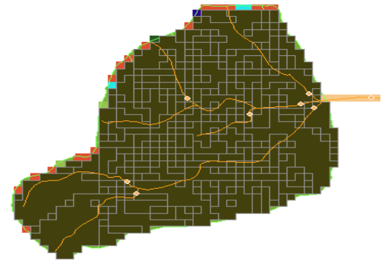
Figure 2. HRUs map generated by SWAT
