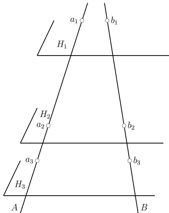
Figure 19.13: The theorem of Thales
