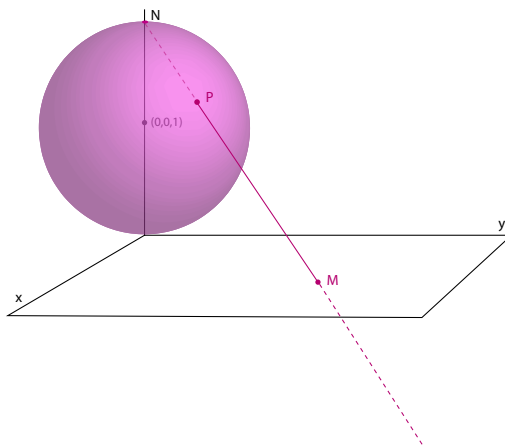
Figure 27.35: The stereographic projections of x^2 + y^2 + (z - 1)^2 = 1 onto the xy -plane.
