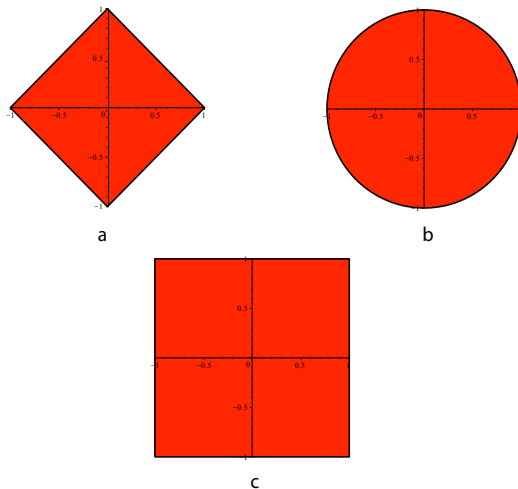
Figure 27.1: Figure (a) shows the diamond shaped closed ball associated with \|\cdot\|_1 . Figure (b) shows the closed unit disk associated with \|\cdot\|_2 , while Figure (c) illustrates the closed unit ball associated with \|\cdot\|_\infty .
