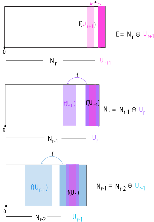
Figure 21.2: A schematic illustration of N_i = N_{i-1} \oplus U_i with f(U_i) \subseteq U_{i-1} for i = r+1, r, r-1 .
