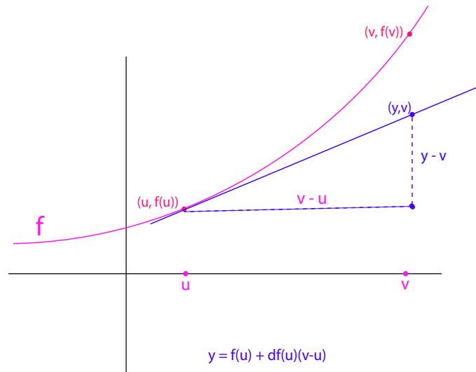
Figure 30.3: An illustration of a convex valued function f . Since f is convex it always lies above its tangent line.
