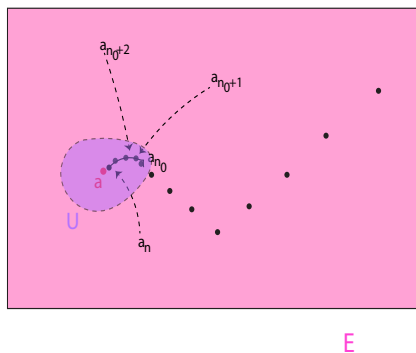
Figure 27.20: A schematic illustration of 27.16.
