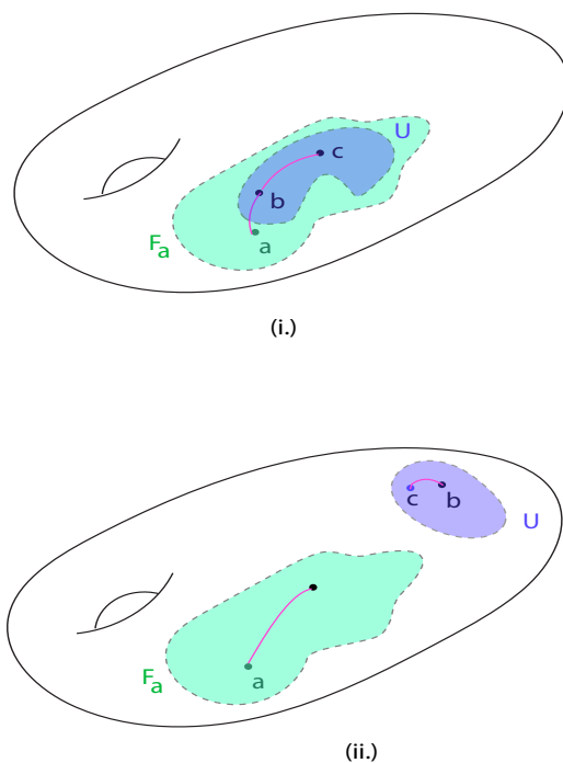
Figure 27.27: Schematic illustrations of the proof techniques that show F_a is both open and closed.
