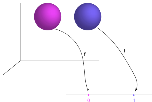
Figure 27.23: An example of a locally constant, but not constant, real-valued function f over the disconnected set consisting of the disjoint union of the two solid balls. On the pink ball, f is 0, while on the purple ball, f is 1.
