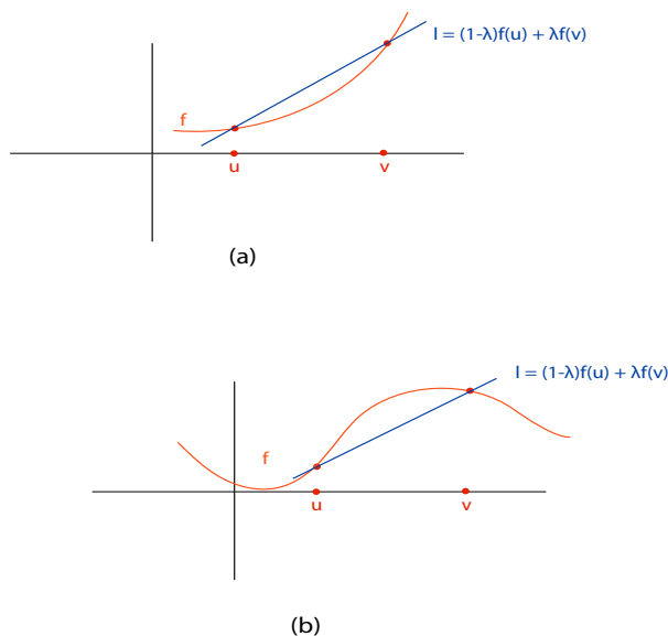
Figure 30.2: Figures (a) and (b) are the graphs of real valued functions. Figure (a) is the graph of convex function since the blue line lies above the graph of f . Figure (b) shows the graph of a function which is not convex.
