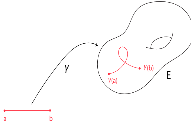
Figure 27.26: Let E be the torus with subspace topology induced from \mathbb{R}^3 with red arc \gamma([a, b]) . The torus is both arcwise connected and locally arcwise connected.
