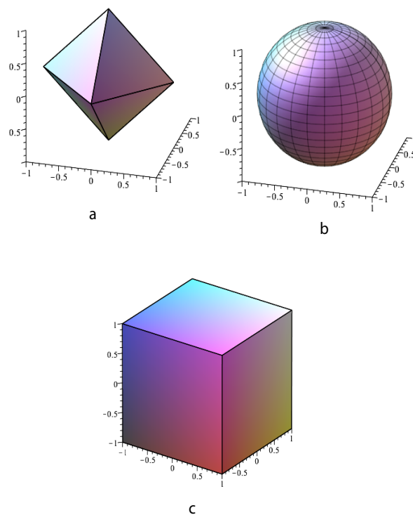
Figure 27.3: Figure (a) shows the octahedral shaped closed ball associated with \|\cdot\|_1 . Figure (b) shows the closed spherical associated with \|\cdot\|_2 , while Figure (c) illustrates the closed unit ball associated with \|\cdot\|_\infty .
