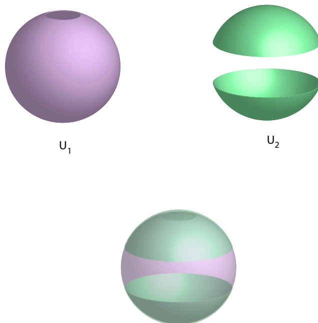
Figure 27.28: An open cover of S^2 using two open sets induced by the Euclidean topology of \mathbb{R}^3 .
