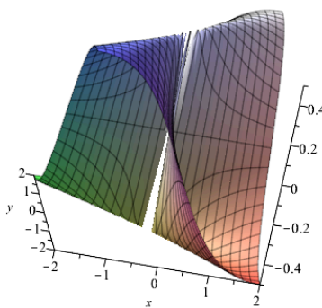
Figure 27.18: The graph of f(x, y) = \frac{xy}{x^2+y^2} for (x, y) \neq (0, 0) . The bottom of this graph, which shows the approach along the line y = -x , does not have a z value of 0.
