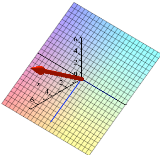
Figure 21.1: The direct sum decomposition of \mathbb{R}^3 = W_1 \oplus W_2 where W_1 is the plane x + z = 0 and W_2 is line t(1, 0, 1) . The spanning vectors of W_1 are in blue.
