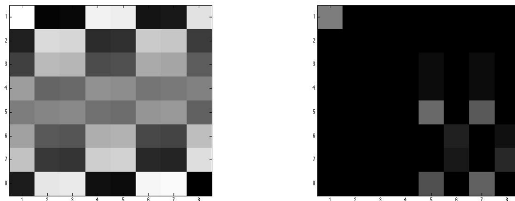
Figure 3.10: An image and its Haar transform
