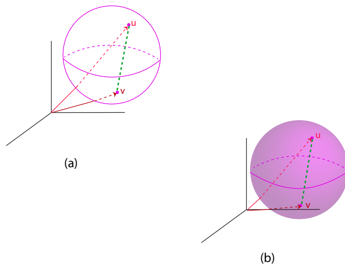
Figure 30.1: Figure (a) shows that a sphere is not convex in \mathbb{R}^3 since the dashed green line does not lie on its surface. Figure (b) shows that a solid ball is convex in \mathbb{R}^3 .
