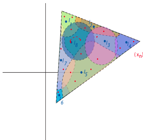
Figure 27.40: The space E the closed triangular region of \mathbb{R}^2 . Given a sequence (x_n) of red points in E , if the sequence has no accumulation points, then each l_i for 1 \leq i \leq 8 , is not an accumulation point. But as implied by the illustration, l_8 actually is an accumulation point of (x_n) .
