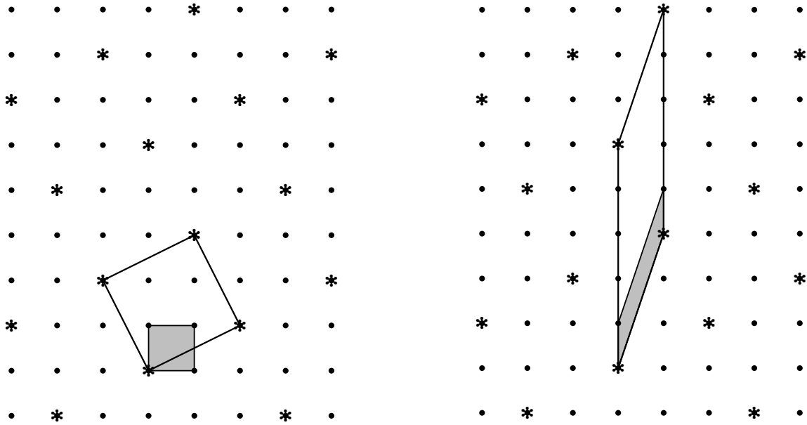
Figure 25.1: Diagonalization applied to a lattice
