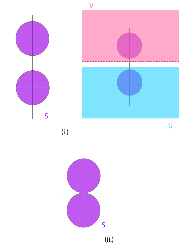
Figure 27.22: Figure (i.) shows that the union of two disjoint disks in \mathbb{R}^2 is a disconnected set since each circle can be separated by open half regions. Figure (ii.) is an example of a connected subset of \mathbb{R}^2 since the two disks can not be separated by open sets.
