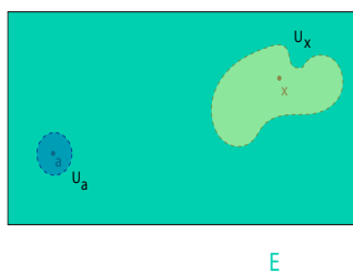
Figure 27.6: A schematic illustration of the Hausdorff separation property
