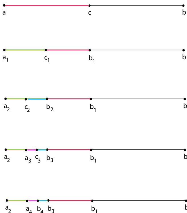
Figure 27.29: The first four stages of the nested interval construction utilized in the proof of Proposition 27.22.
