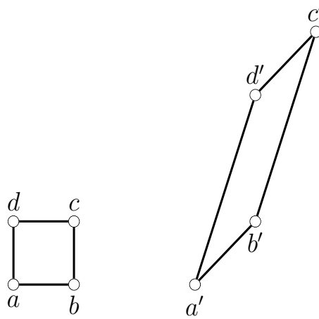
Figure 19.11: The effect of an affine map
