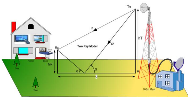
Fig 3. The ground, a perfect reflector in two ray model.
