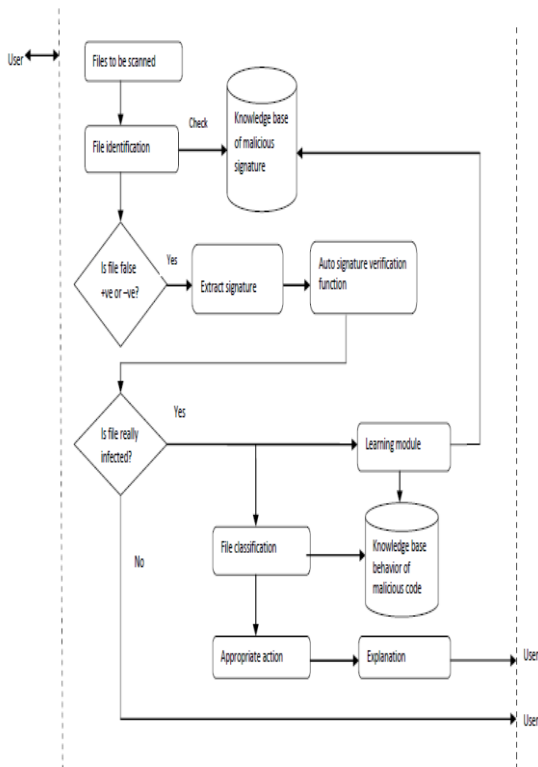
Figure.8. Flowchart for malware detection expert system
