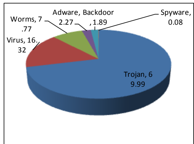
Figure.1. Distribution of various types of malware
