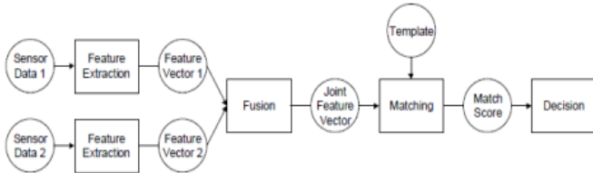
Fig. 6. Fusion at the feature extraction level
