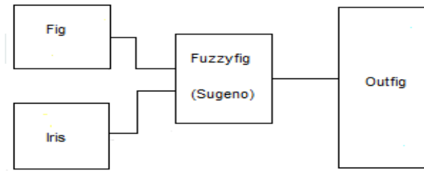
Fig. 10. Membership function
