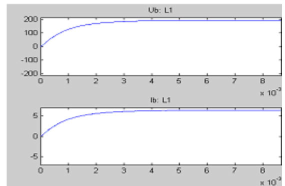
Fig 5 (e) Output voltage and current
