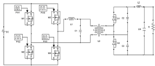
Fig 2. Half Bridge DC-DC Converter.
