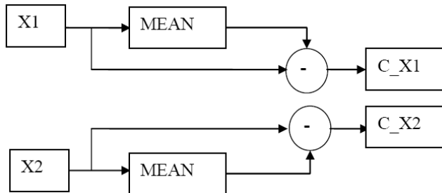
Fig.2 Implementation of Centering
