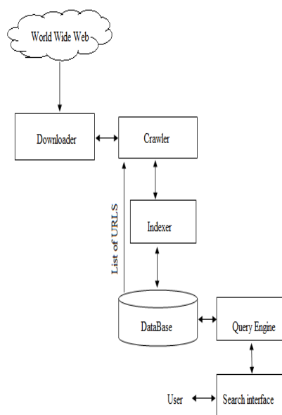
Figure 1 Architecture of a web search engine [5]
