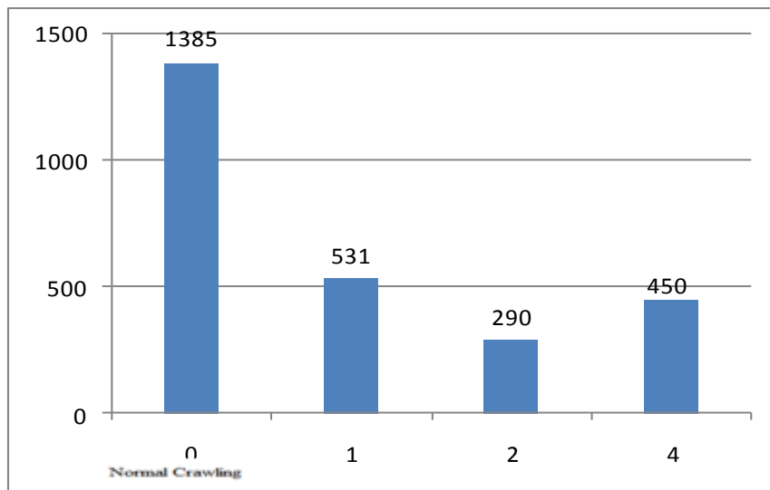
Graph 1 Time Take by Crawler to Download Updated Web Page in Test (time in millisecond)
