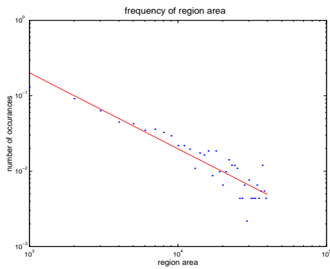
Figure 14: Region Area: This log-log graph shows the distribution in region areas. We fit a curve of the form y = \frac{A}{x^\alpha} yielding an \alpha = 1.008 . For the purposes of fitting, we throw out those sparsely populated bins which contain regions that are greater than 25% of the total image area.
