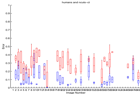
Figure 10: The GCE for human vs. human (blue) and NCuts vs. human (red) for each image for which we have \geq 3 human segmentations. The LCE data is similar.
