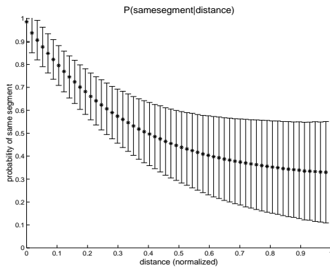
Figure 11: Proximity: this graph documents probability that two points belong to the same segment given their distance. For each segmentation of an image we sample 1000 points at random and compute all pairwise distances. Distances have been scaled per image as discussed in the text and normalized to range from 0 to 1. Error bars show \pm\sigma intervals.
