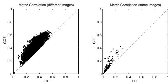
Figure 6: LCE vs. GCE for segmentations of different images (left) and the same image (right). The dashed line x = y shows that GCE is a stricter measure than LCE.
