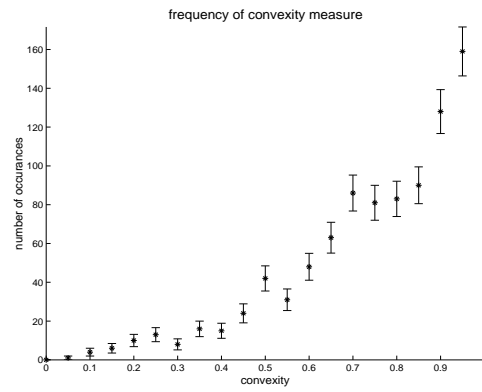
Figure 13: Convexity: this graph captures the distribution in convexity of segments. Convexity is measured as ratio of a region's area to the area of its convex hull yielding a number between 0 and 1. Error bars show \pm\sigma intervals.
