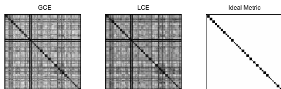
Figure 5: Error matrix for all image pairs, for GCE (left) and LCE (middle). M_{ij} corresponds to the error between segmentations i and j , where black signifies zero error. Segmentations are sorted by image, so segmentations of the same image are adjacent. The spurious horizontal and vertical bands confirm that the spike in the different-image graphs of Figure 4 are caused by degenerate segmentations of one image. The right-most matrix shows the block-diagonal structure of the ideal error measure applied to a flawless dataset.
