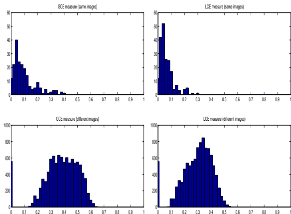
Figure 4: Distributions of the GCE (left) and LCE (right) measures over the segmentation database. The upper graphs show the error for segmentations of the same image. The lower graphs show the error for segmentations of different images. The spike at zero in the different-image graphs is due to degenerate segmentations of one particular image, of which everything else is a refinement.
