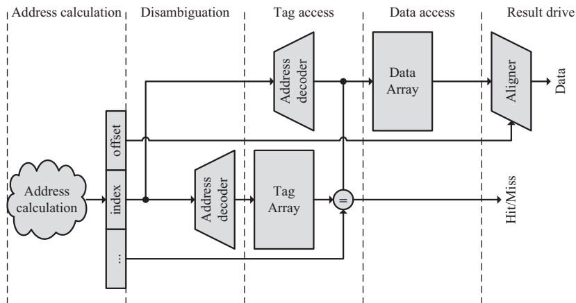
FIGURE 2.4: Serial tag and data array access pipeline.
