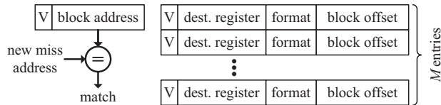
FIGURE 2.6: An explicitly addressed MSHR.
