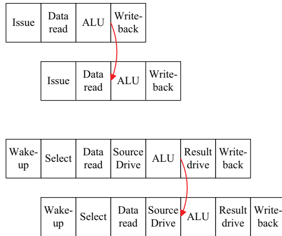
FIGURE 7.9: Dependent instruction execution with value bypassing in a simple pipelined processor (top) and in a deeply pipelined processor (bottom).
