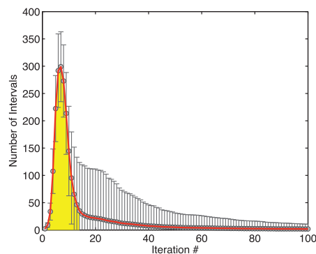
Fig. 7. The average and standard deviation of the number of SA intervals generated per iteration during simulated read alignment on the reference multi-genome (averaged over 10K reads)
