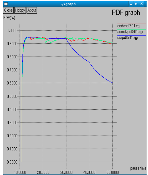
5.2 Comparison of AODV, AOMDV and DSR on basis of PDF at maximum connection 50
