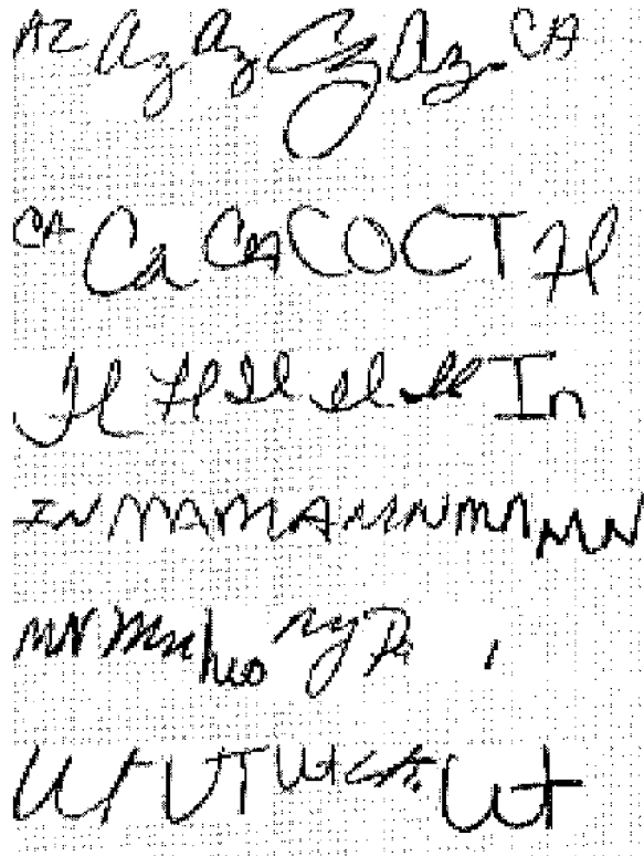
Fig. 11. State abbreviations recognition with 66 classes. The valid abbreviations are: AA, AE, AK, AL, AP, AR, AS, AZ, CA, CM, CO, CT, CZ, DC, DE, FL, FM, GA, GU, HI, IA, ID, IL, IN, KS, KY, LA, MA, MD, ME, MH, MI, MN, MO, MP, MS, MT, NC, ND, NE, NH, NJ, NM, NV, NY, OH, OK, OR, PA, PR, PW, RI, SC, SD, SQ, TN, TX, TT, UT, VA, VI, VT, WA, WI, WV, WY. The figure shows image snippets containing two-letter abbreviations collected from actual mail.
