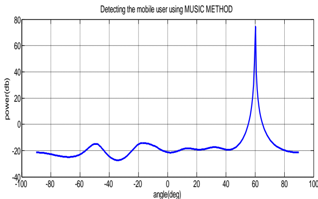
Figure 2: Detection of user in look direction by MUSIC for 8 antenna elements
