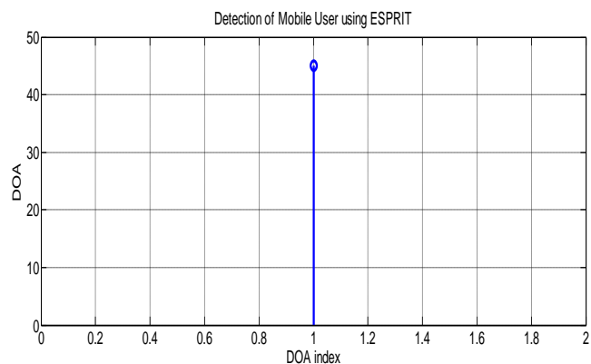
Figure 3: Detection of User in look direction by ESPIRT for 100 antenna elements
