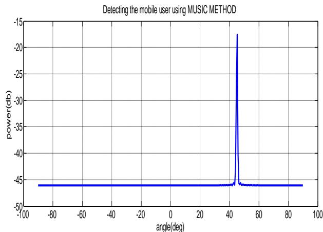
Figure 4: Detection of user in look direction by MUSIC for 100 antenna elements.
