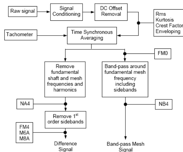
Figure 2. Processing Flow for Feature Extraction Techniques
