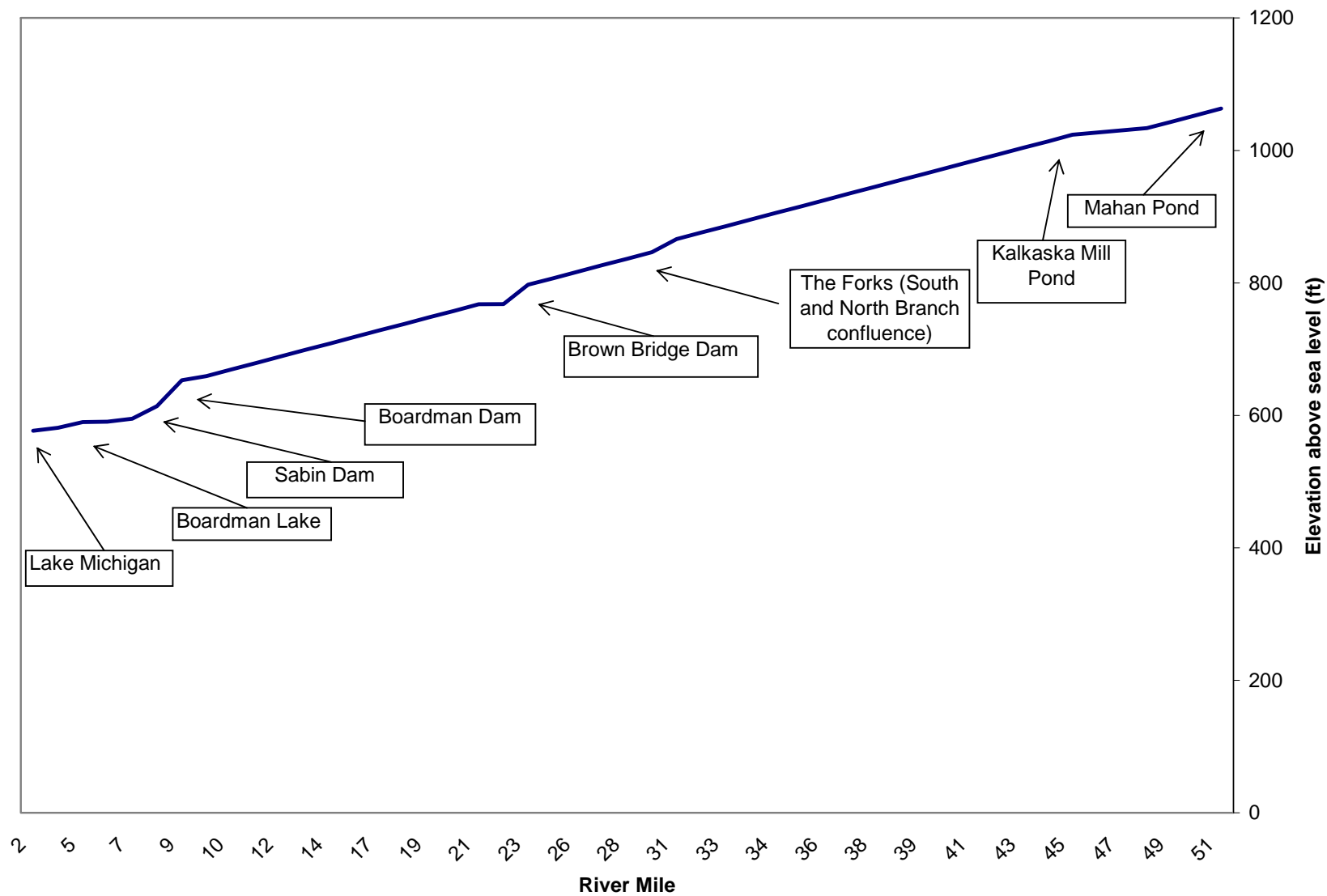
Figure 10.—Elevation changes, by river mile, from headwaters to the mouth of the Boardman River.
