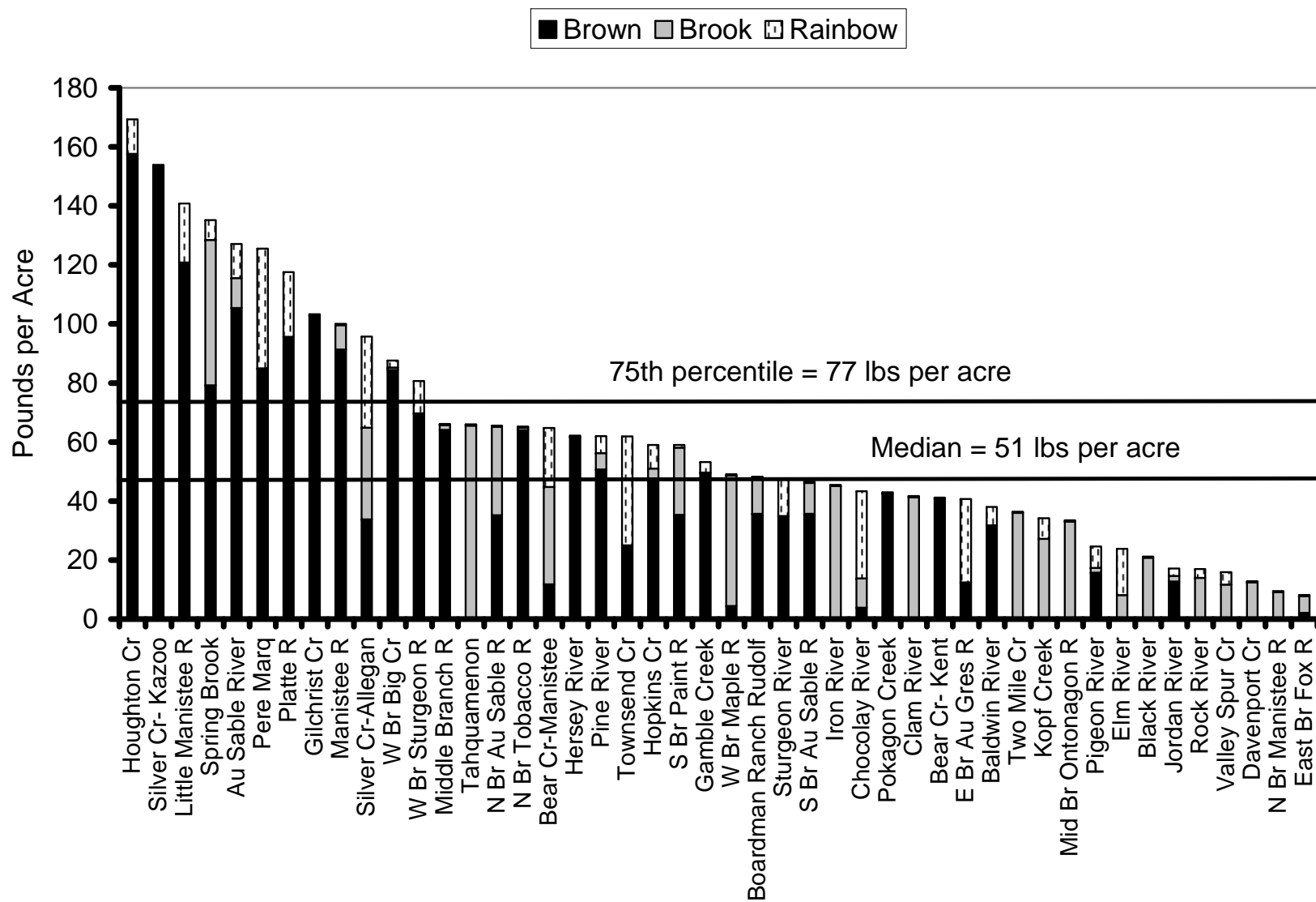
Figure F.8.—Pounds per acre of trout at 46 fixed SSTP sites.
