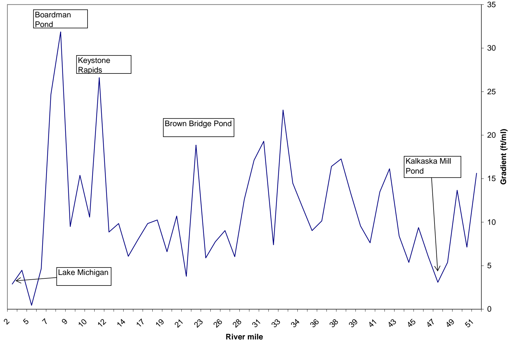
Figure 9.—Gradient (elevation change in feet per mile) of the Boardman River.
