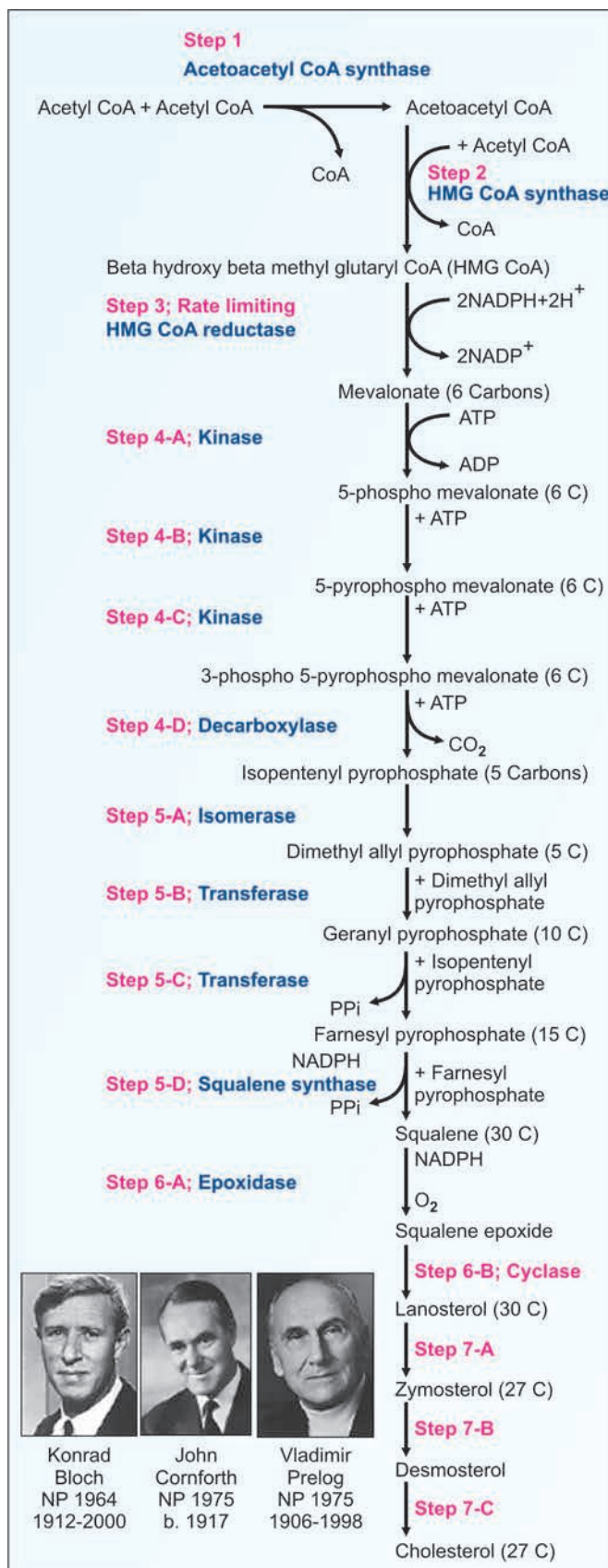
Fig. 12.4. Cholesterol biosynthesis
