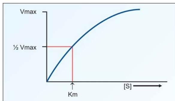
Fig. 5.13A. Effect of substrate concentration (substrate saturation curve)
