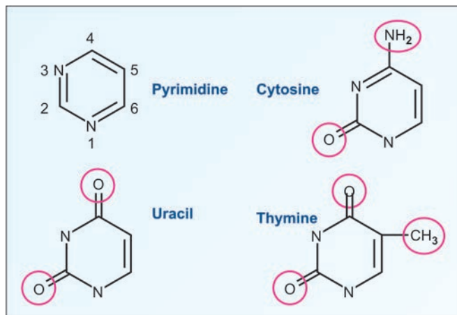
Fig. 39.3. Common pyrimidines
