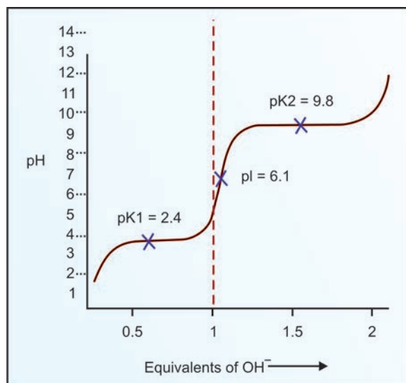
Fig. 3.14. Titration curve of glycine; pH in Y-axis
