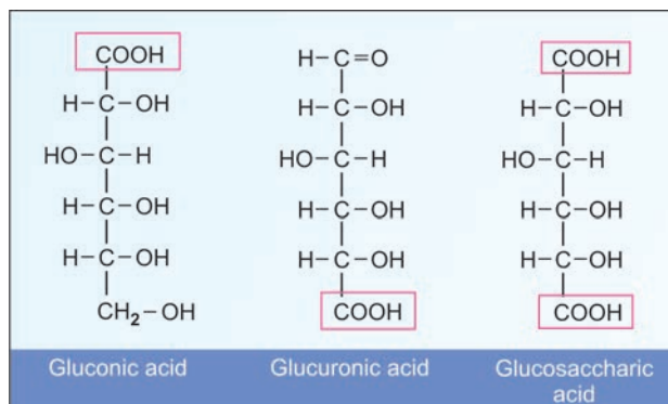
Fig. 6.12. Oxidative products of glucose
