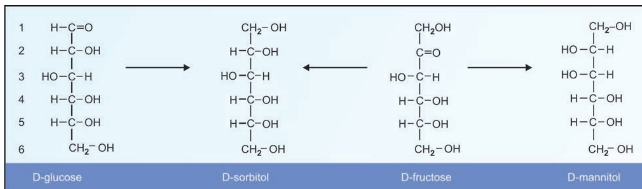
Fig. 6.13. Reduction of sugar to alcohol
