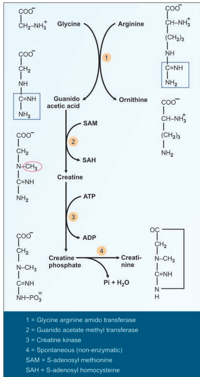
Fig. 15.5. Creatine metabolism
