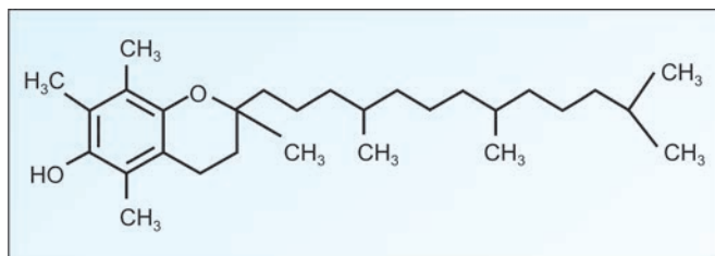
Fig. 33.12. Alpha tocopherol
