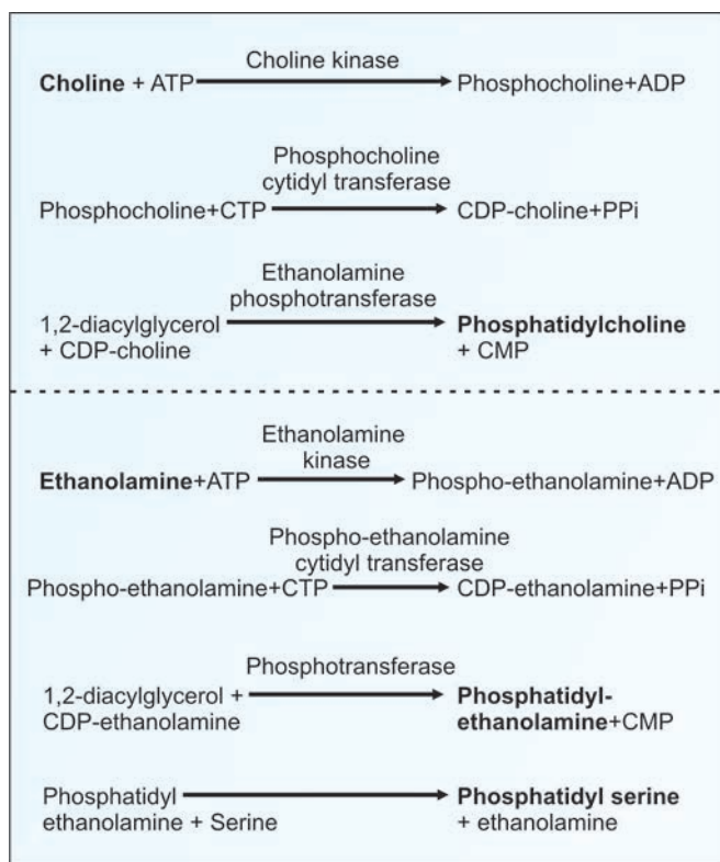
Fig. 13.6. Synthesis of phosphatidylcholine; phosphatidyl ethanolamine; phosphatidyl serine
