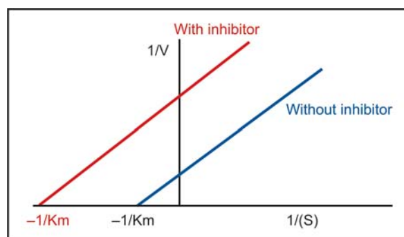
Fig. 5.24. Uncompetitive inhibition
