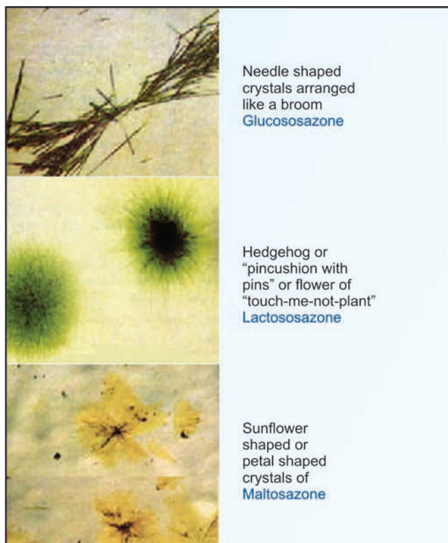
Fig. 6.11. Shape of osazones under microscope
