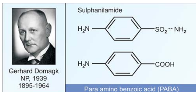
Fig. 5.21. Competitive inhibition
