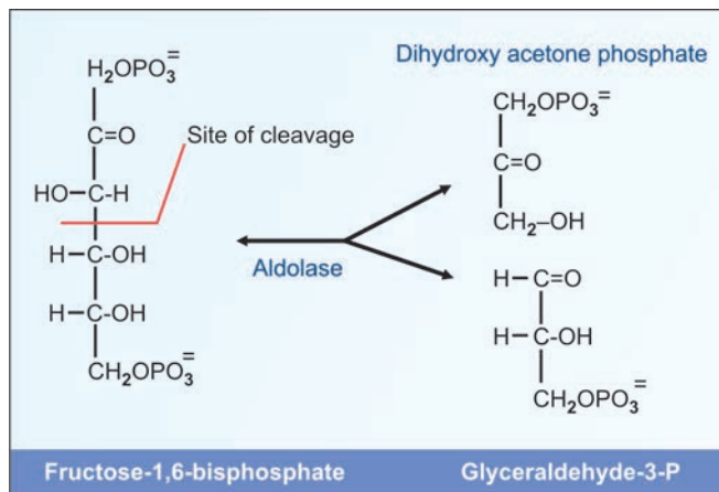
Fig. 9.8. Step 4 of glycolysis; reversible
