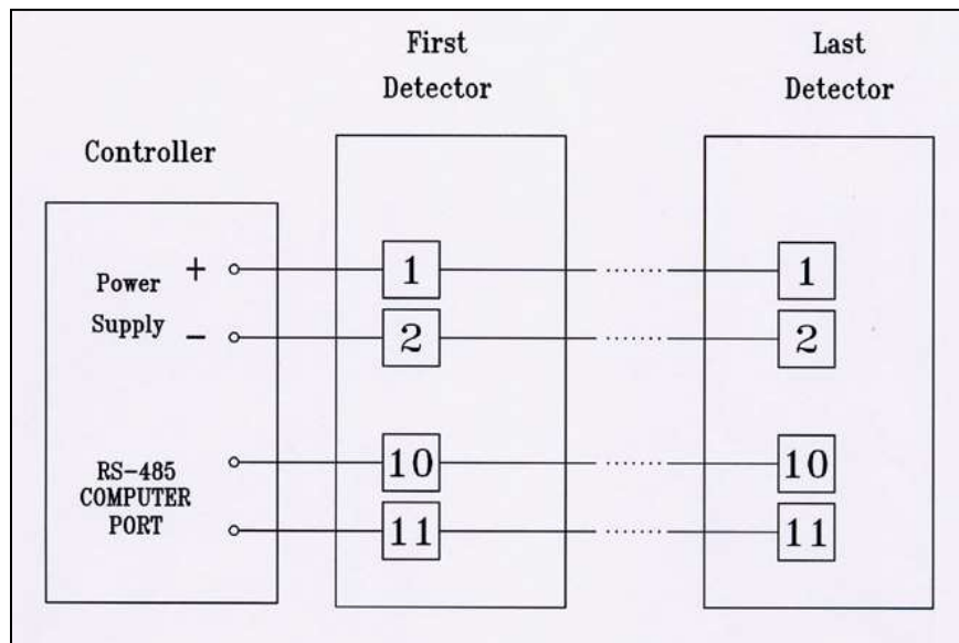
Figure 15: RS-485 Networking
