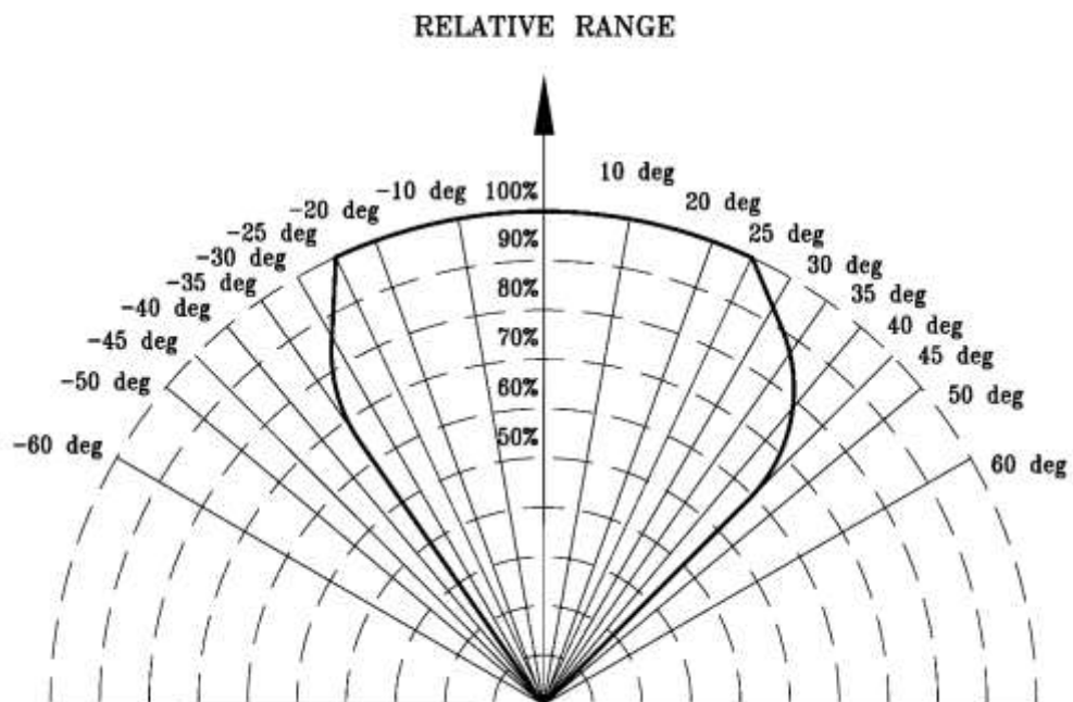
Figure 2: Horizontal Fields of View for Hydrogen
