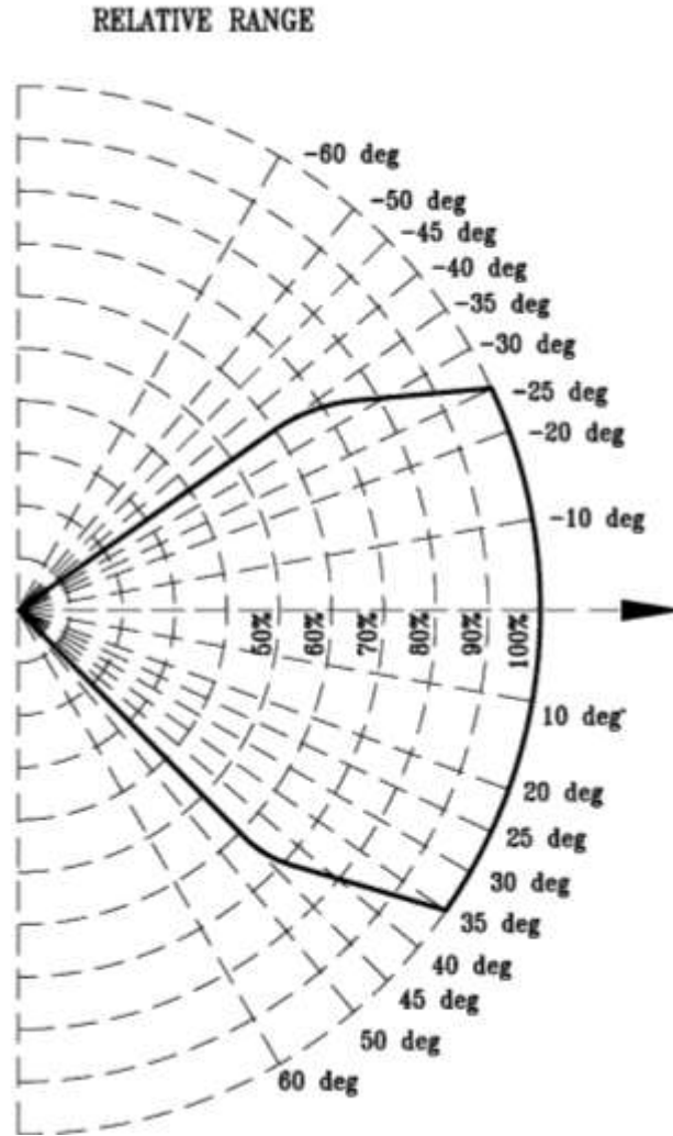
Figure 3: Vertical Field of View for Hydrogen
