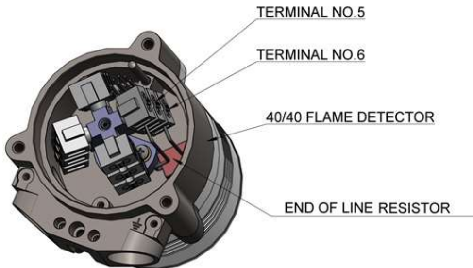
Figure 22: End of Line Resistor Assembly
