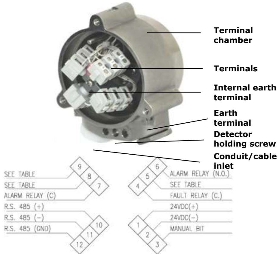
Figure 8: Detector with Cover Removed
