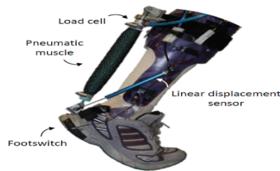
Figure 8.5 Exoskeleton for lower limb
