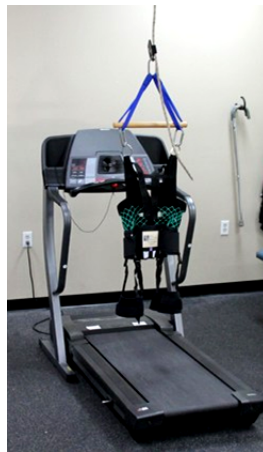
Figure 8.8 Over head suspension unit Figure 8.9 Body weight supported treadmill training device
