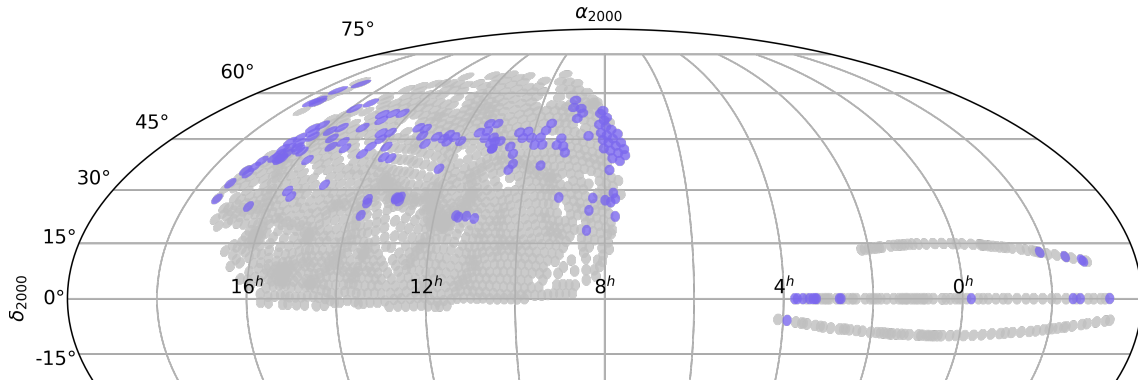
FIG. 5.— The sky distribution (Mollweide equatorial projection for \text{Dec} > -20^\circ ) of possible MaNGA plates (in grey). Because MaNGA targets are selected from a sample with SDSS-I photometry and redshifts, this footprint corresponds to the Data Release 7 imaging data (Abazajian et al. 2009). Each plate contains 17 MaNGA targets, and around 30% of all possible plates will be observed in the full 6-year survey. The purple indicates plates with data released as part of DR14.
