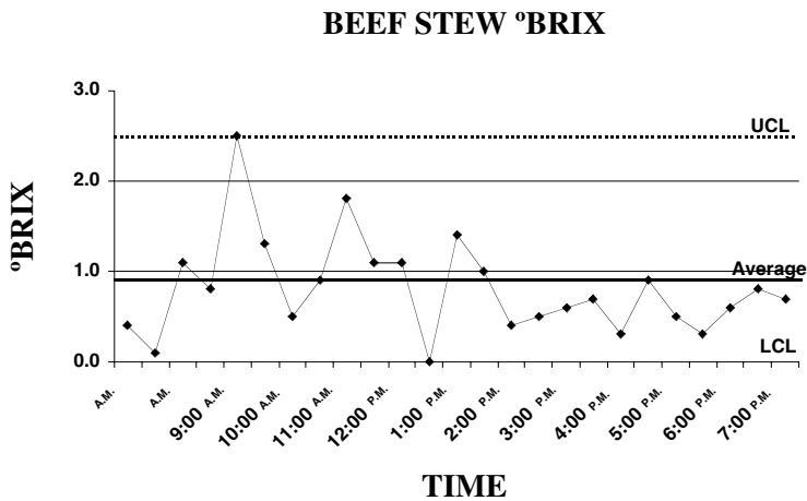
Figure 2.8 Range chart.
