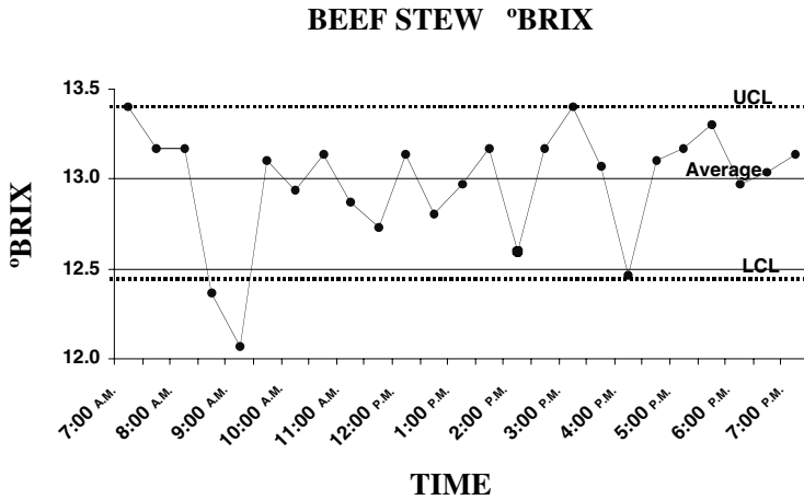
Figure 2.7 Average (X) chart.
